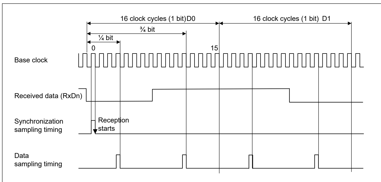
Figure 27.59 Data reception sampling timing in Manchester mode
