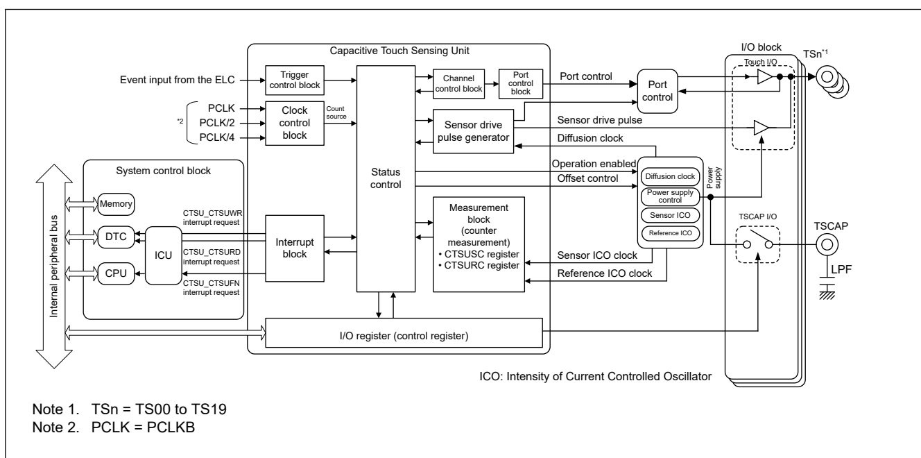
Figure 40.3 CTSU block diagram
