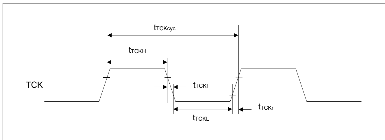
Figure 47.67 JTAG TCK timing
