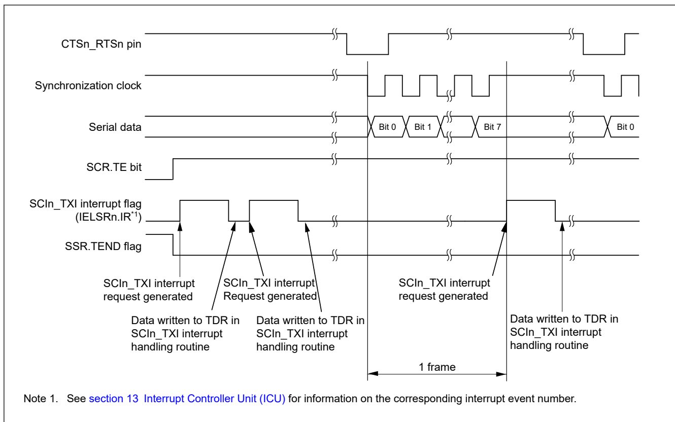
Figure 27.67 Example of serial data transmission in clock synchronous mode when the CTS function is used at the beginning of transmission
