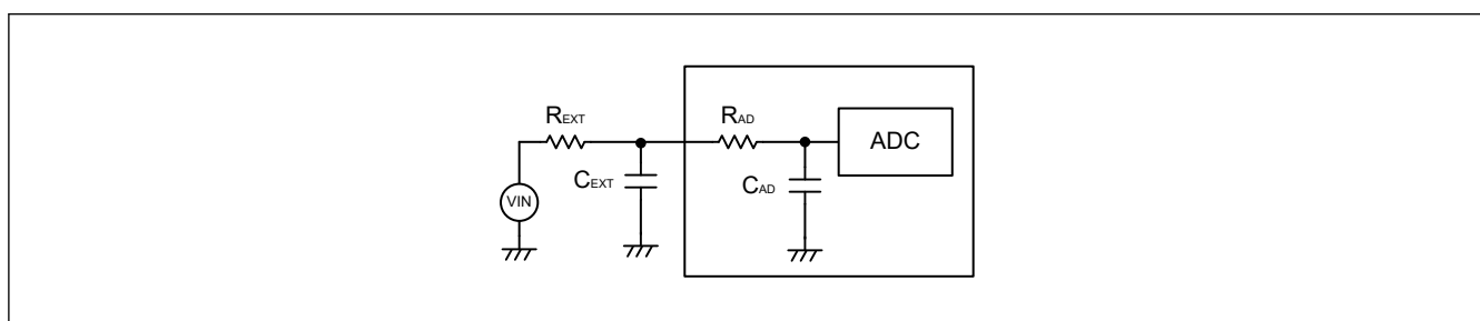
Figure 37.40 Sample and hold circuit simplified diagram
