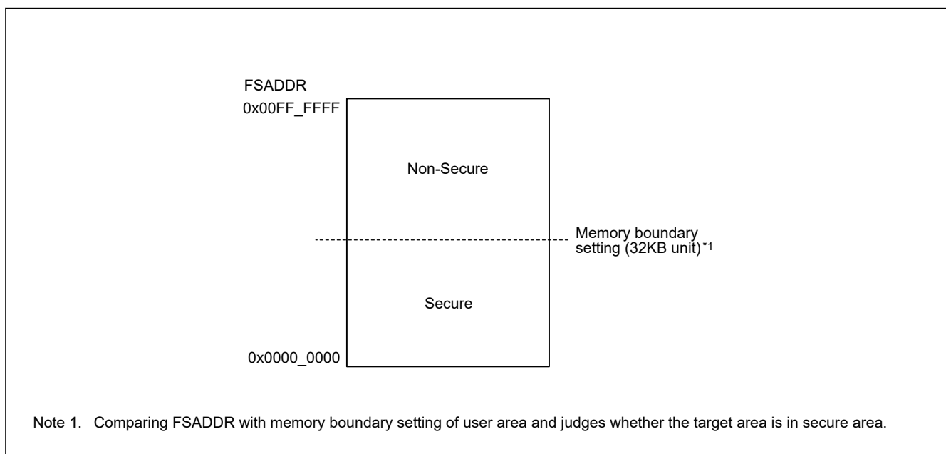
Figure 44.33 Secure/non-secure region in user area
