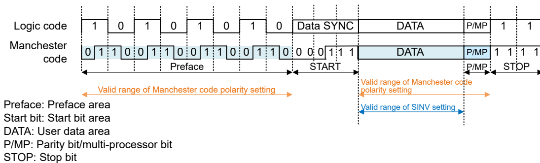
Figure 27.64 Valid range of the Manchester code polarity setting
