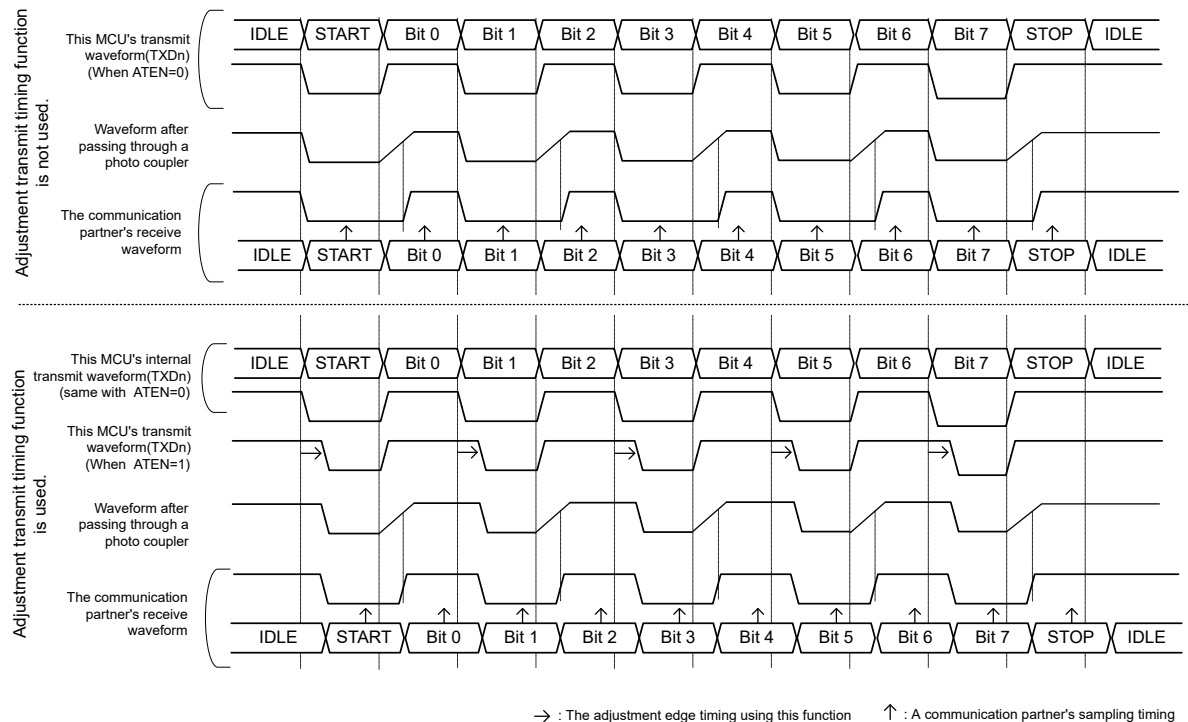
Figure 27.37 Explanation for a transmit waveform through a photo coupler
