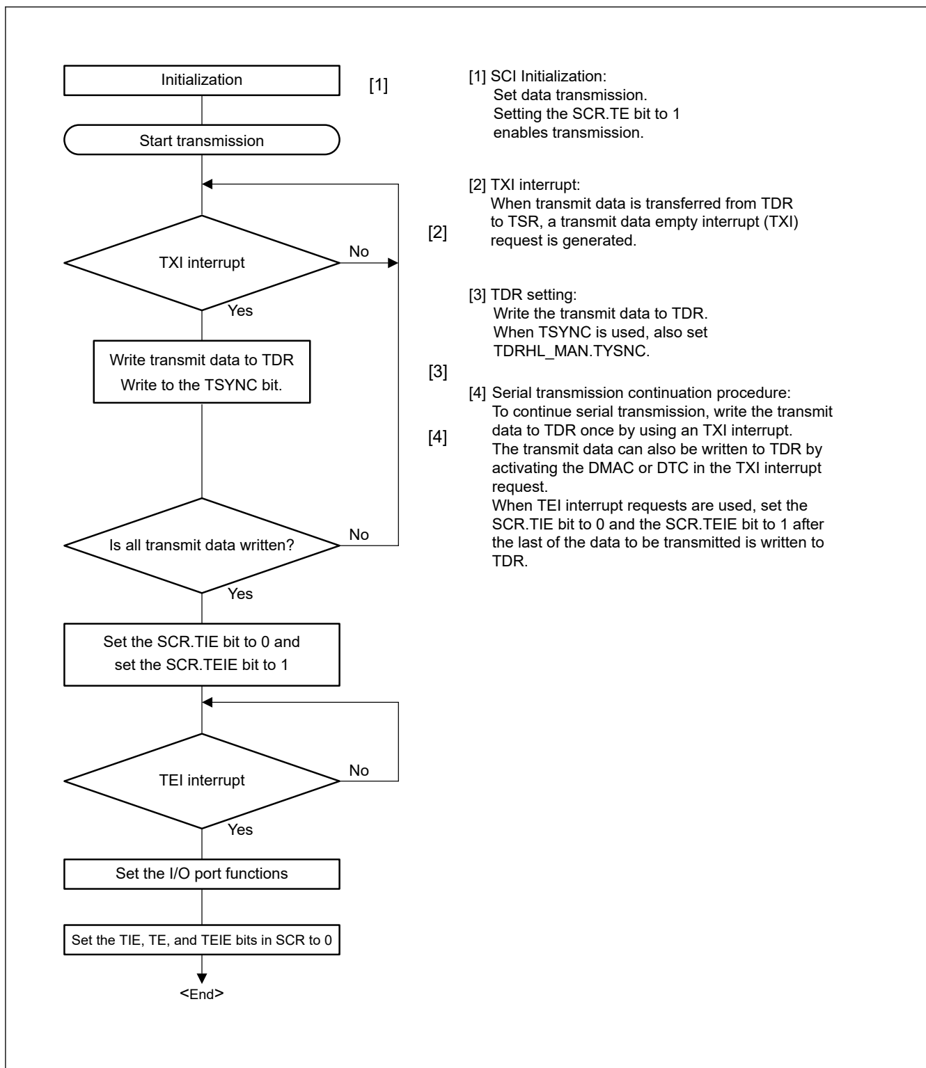
Figure 27.55 Example flow of a serial transmission in Manchester mode
