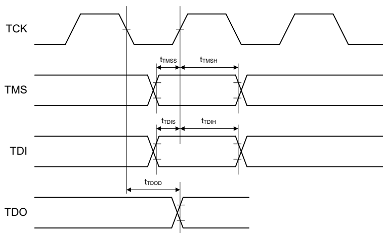
Figure 47.65 Boundary scan input/output timing
