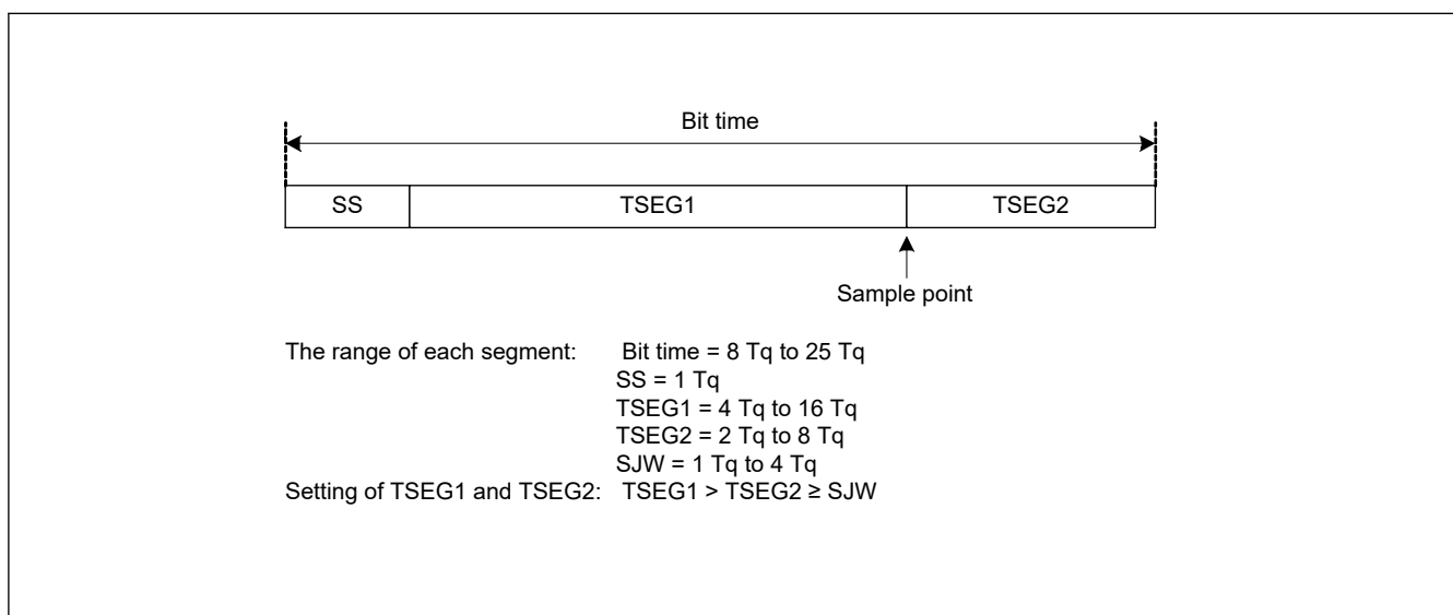
Figure 29.12 Bit timing
