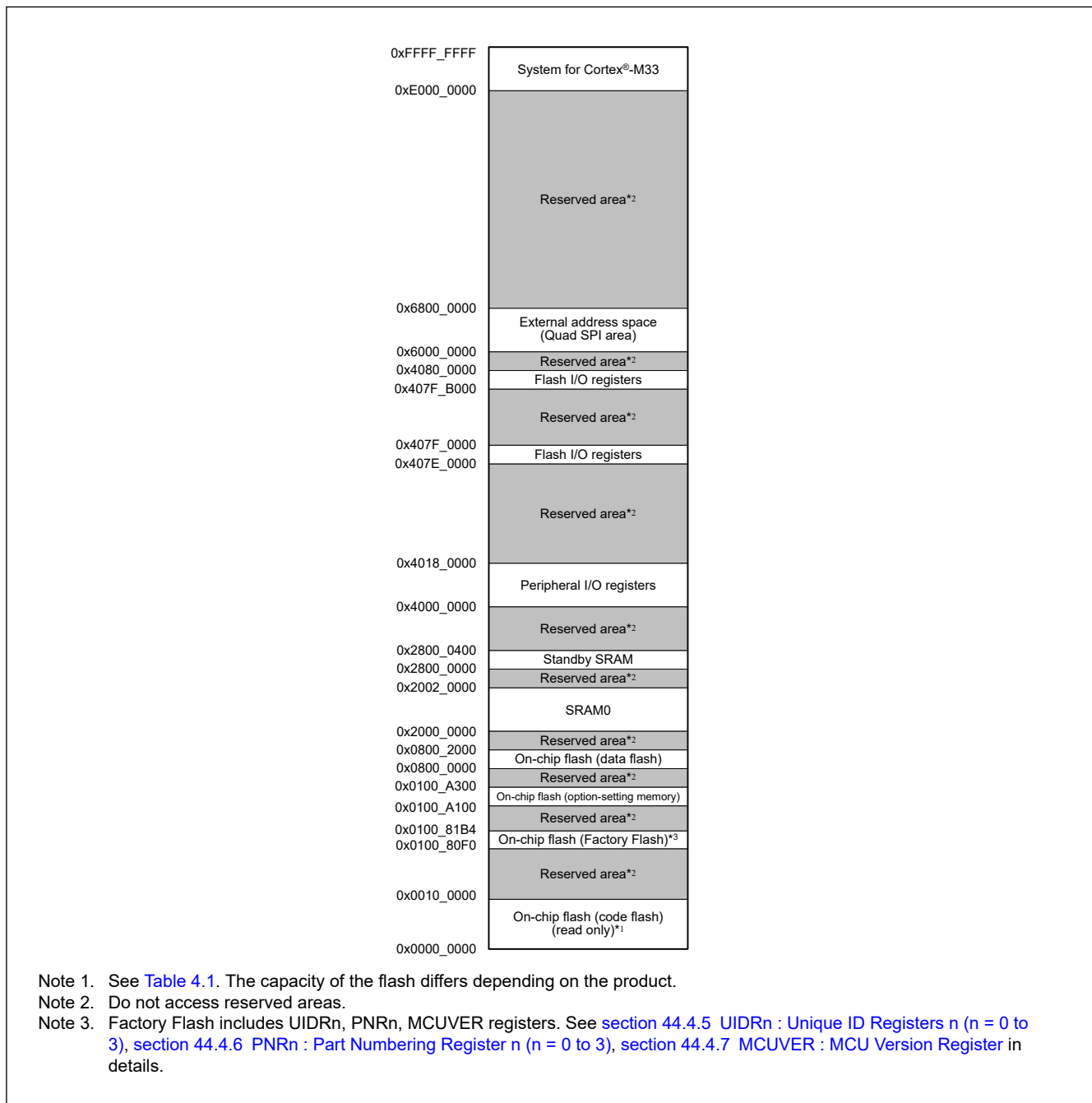
Figure 4.1 Memory map
