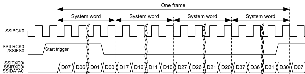
Figure 32.41 TDM format (without padding: system word length = data word length)
