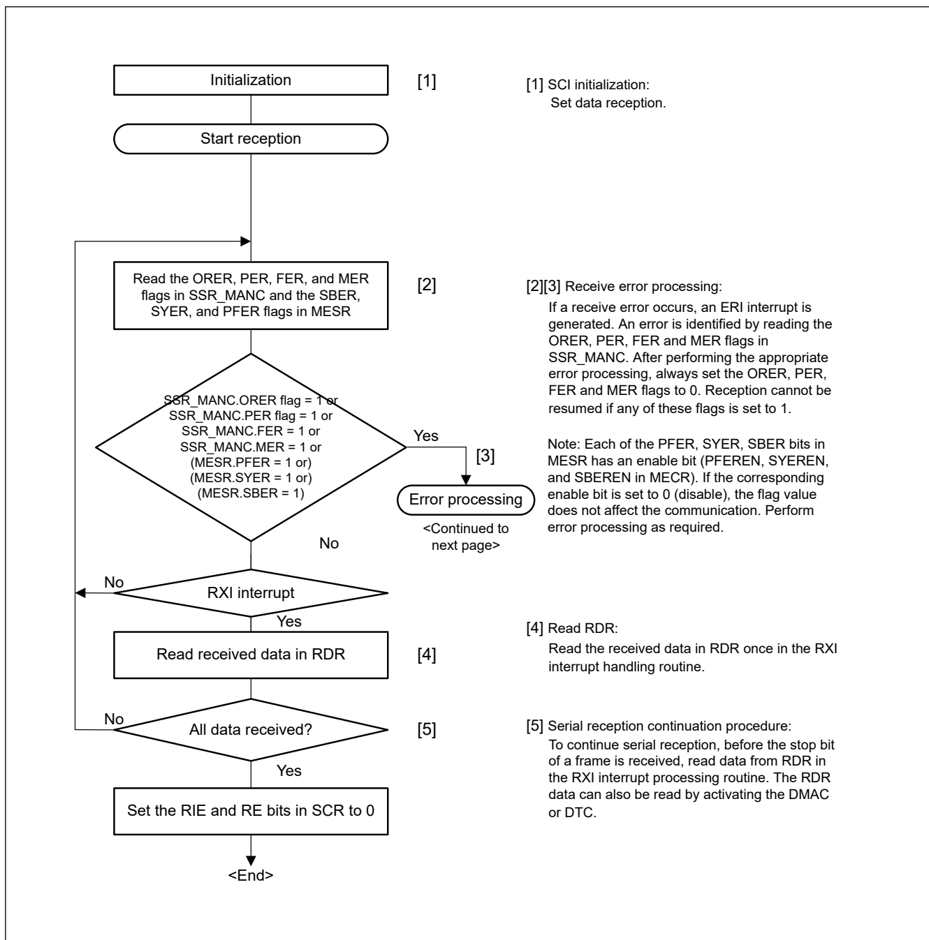
Figure 27.61 Example flow of serial data reception in Manchester mode (normal reception)
