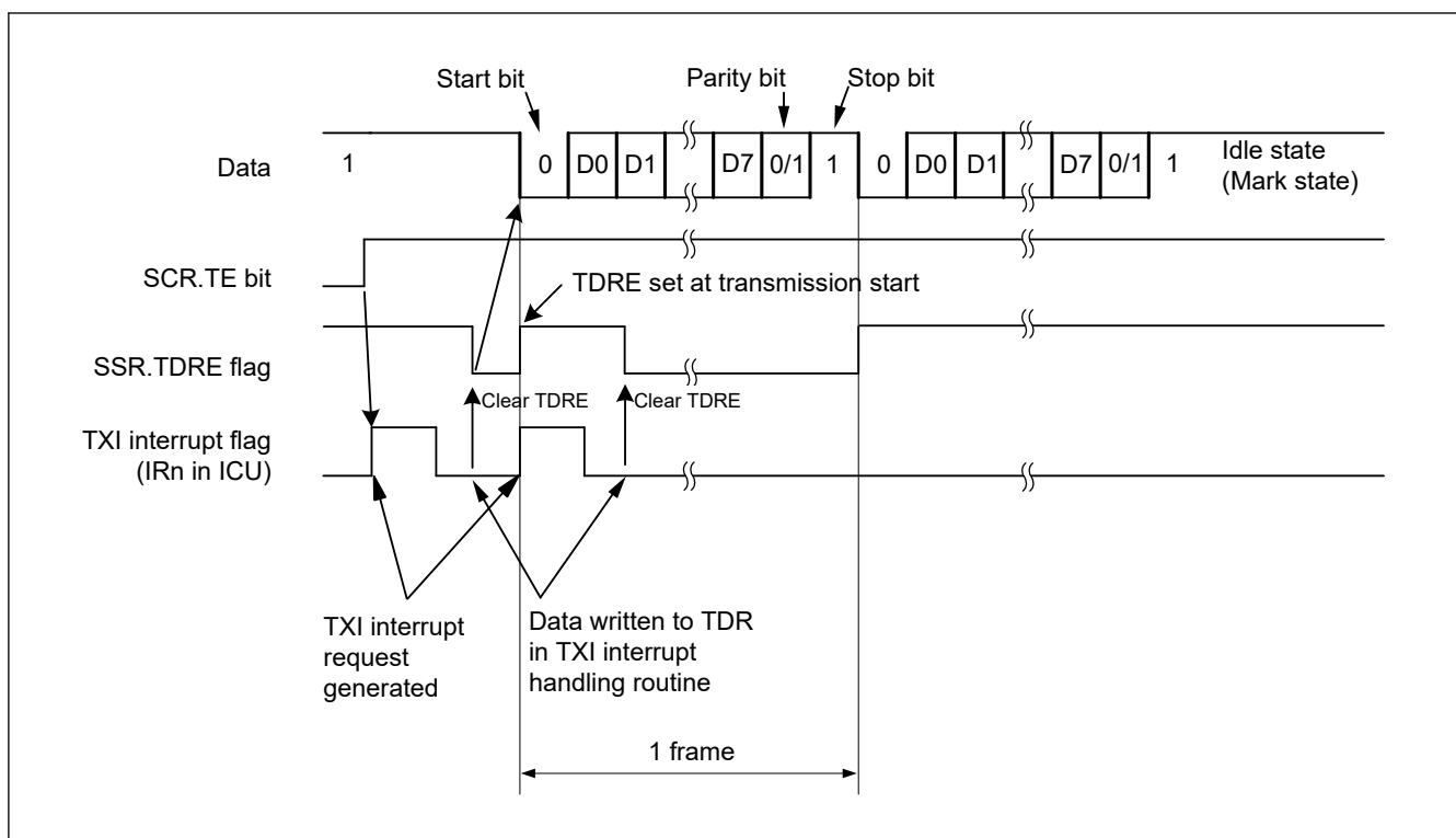
Figure 27.14 Example of operation for serial transmission in asynchronous mode (4) (with 8-bit data, parity, 1 stop bit, CTS function not used, from the middle of transmission until transmission completion, stop preamble)
