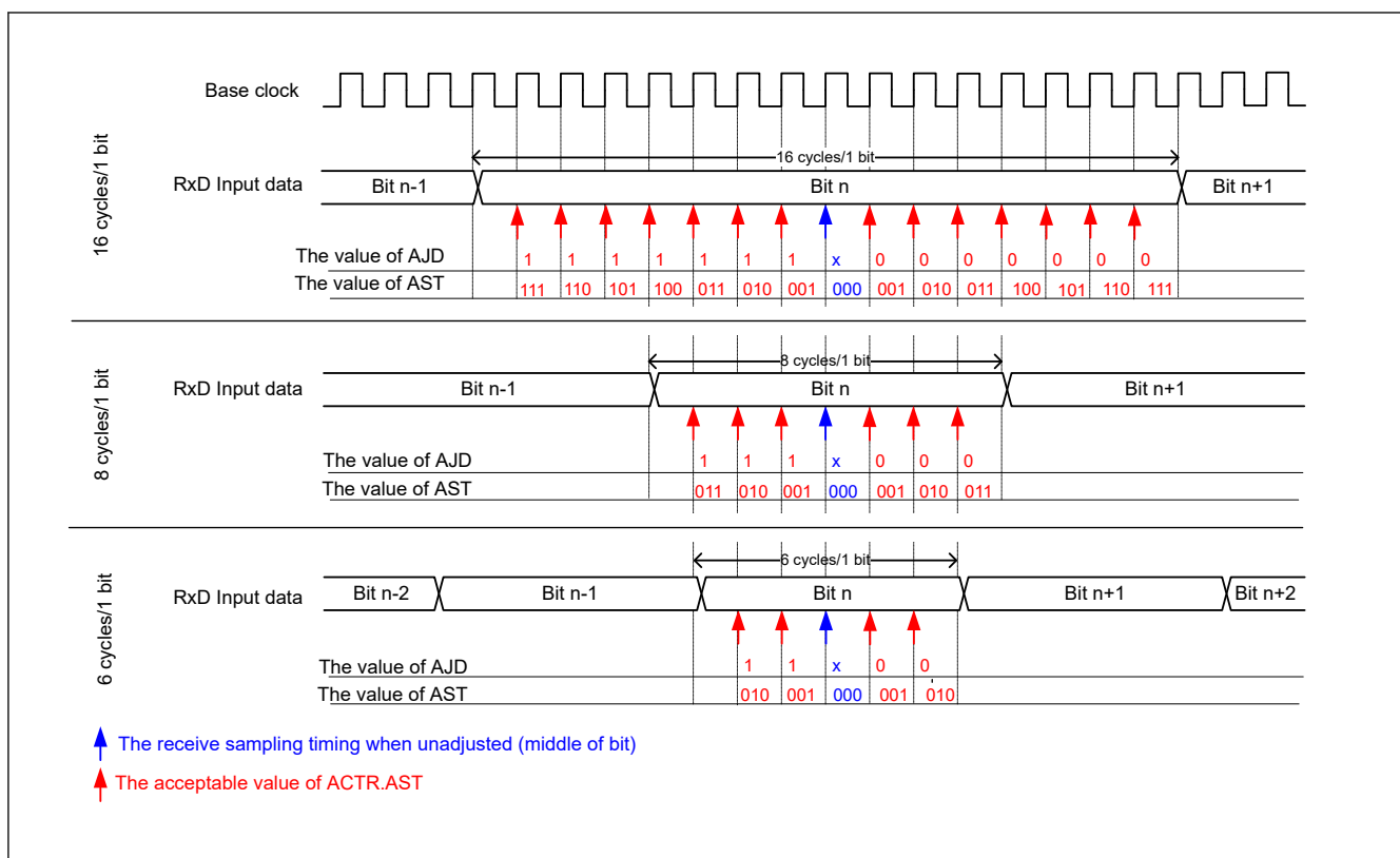
Figure 27.34 Overview of the adjustment operation for the reception sampling timing (asynchronous mode using an internal clock)
