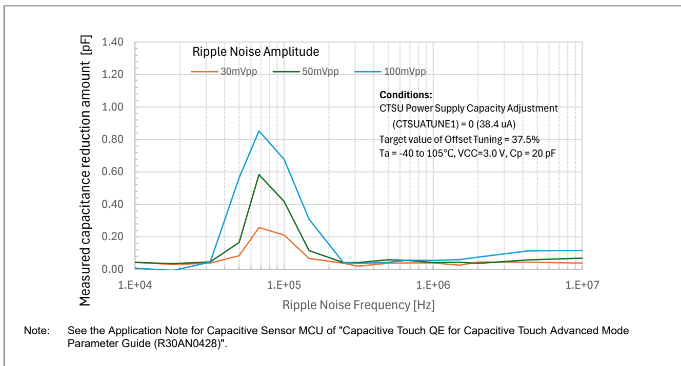
Figure 47.62 Measured capacitance reduction amount
