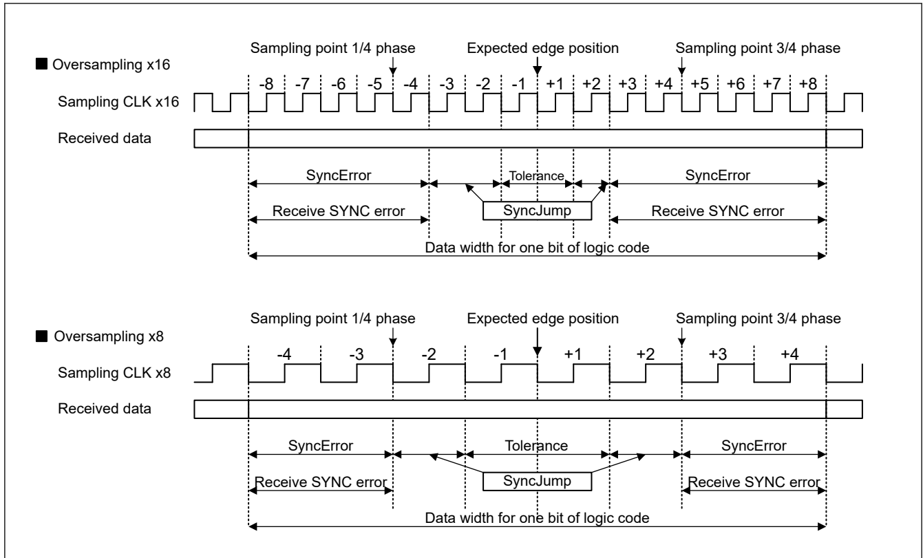
Figure 27.63 Conceptual image of a reception retiming range
