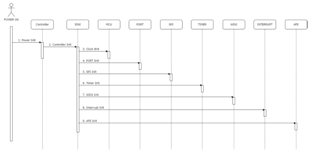
Fig. 7 Software initialization
