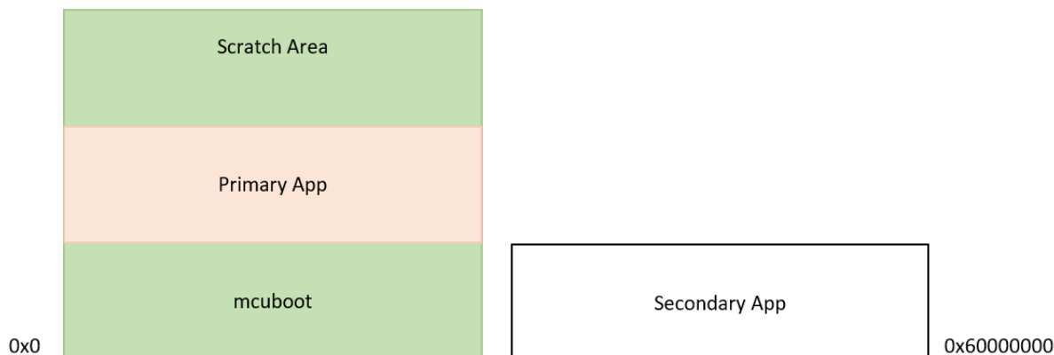
Figure 150: MCUboot Memory Map with QSPI
