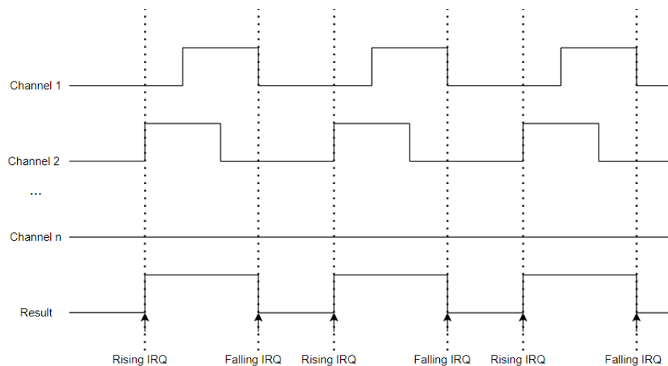
Figure 339: IPLS IRQ Generation
