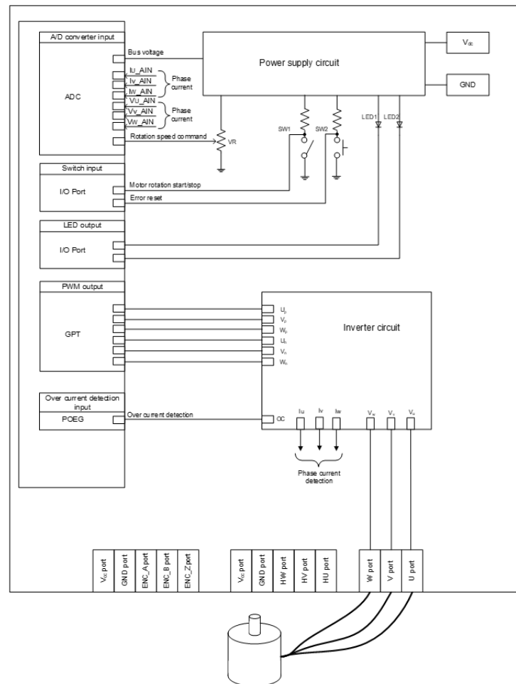
Figure 273: Example of target hardware of motor 120-degree sensorless
