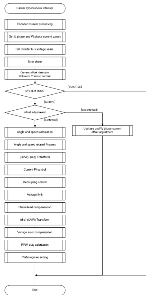
Figure 318: Current control process
