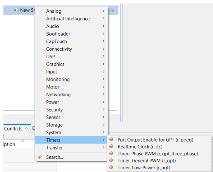
Figure 35: Select a driver
