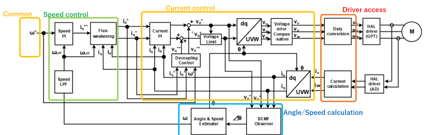
Figure 272: Image of Current Control Module(yellow block)
