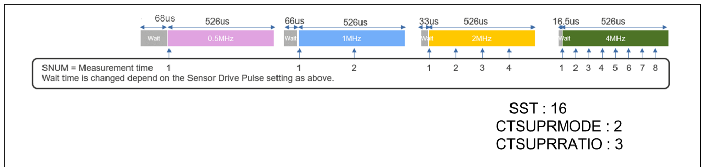
Figure 182: Self-capacitance Measurement Period (CTS1)
