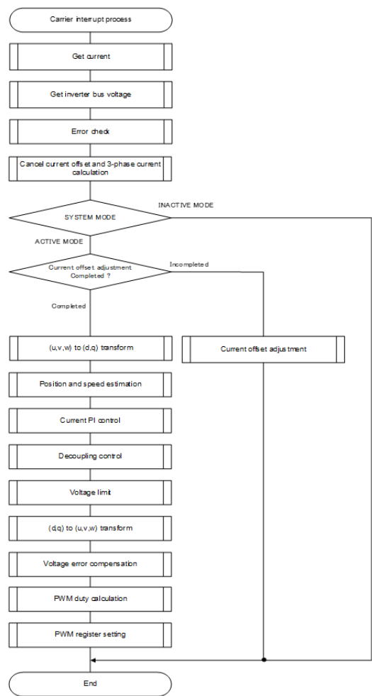
Figure 309: Current control process
