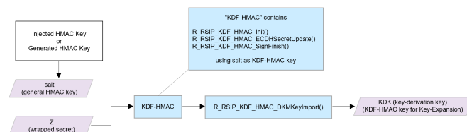
Figure 347: Two-Step Key Derivation Randomness Extraction flow
