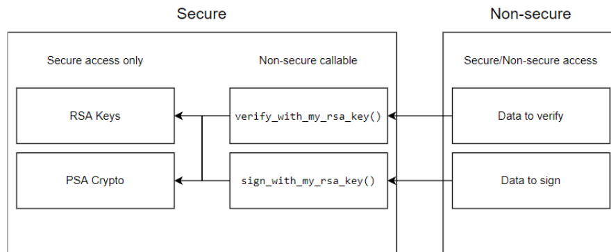
Figure 340: PSA Crypto Non-secure callable example
