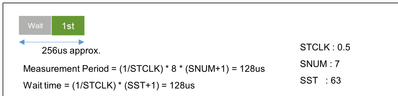
Figure 185: Current Measurement Period
