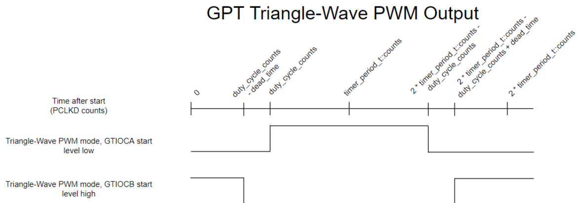
Figure 362: GPT Triangle-Wave PWM Output
