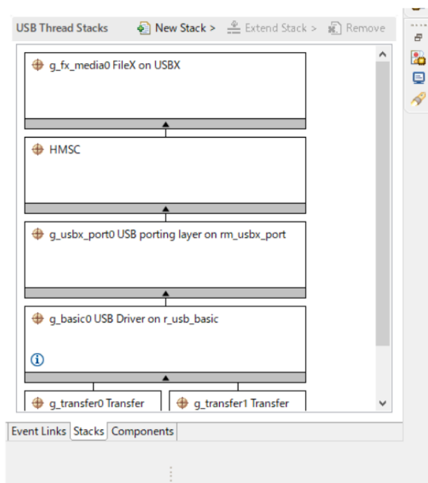
Figure 215: FileX on USBX Stack
