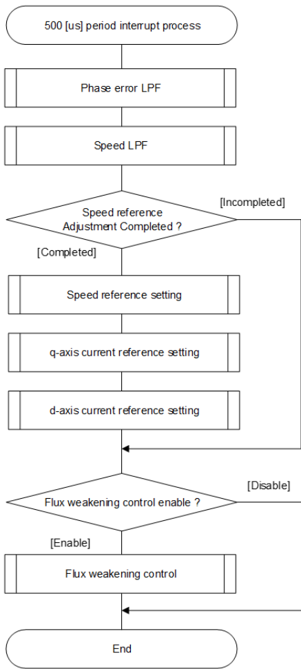
Figure 301: Speed control process
