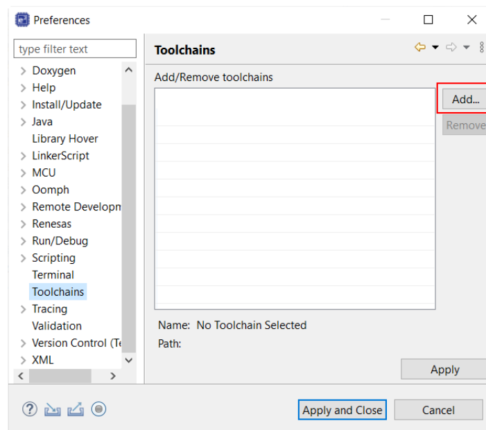
Figure 60: Add Toolchain
