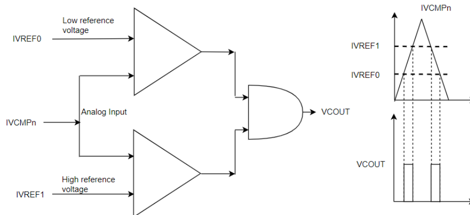
Figure 168: ACMPPLP Window Mode Operation
