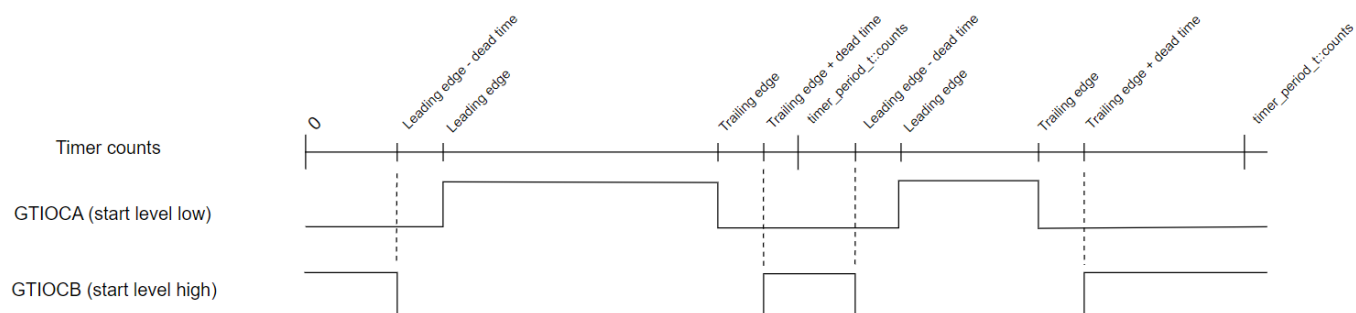
Figure 359: GPT One-Shot Pulse Output (with dead time)
