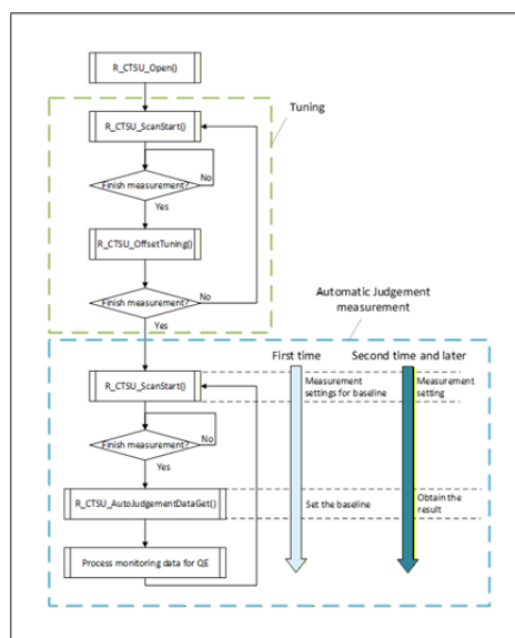
Figure 186: Basic operation model of automatic judgment mode
