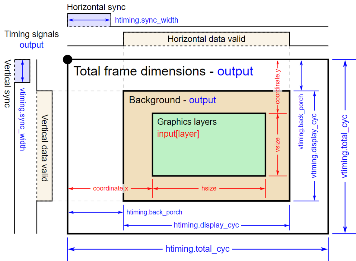
Figure 266: GLCDC layers and timing
