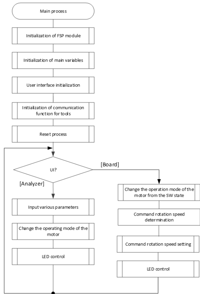
Figure 299: Main process
