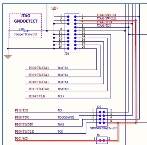
Figure 140: Example of MD Mode Pin Connection to Debugger Connector (from EK schematic)
