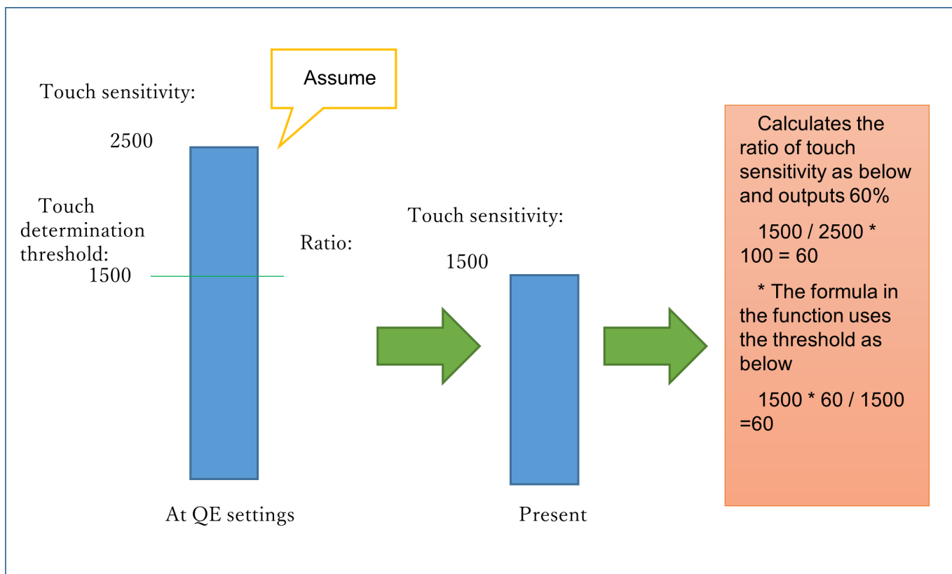
Figure 205: Example of decrease touch sensitivity for thicker overlay panels
