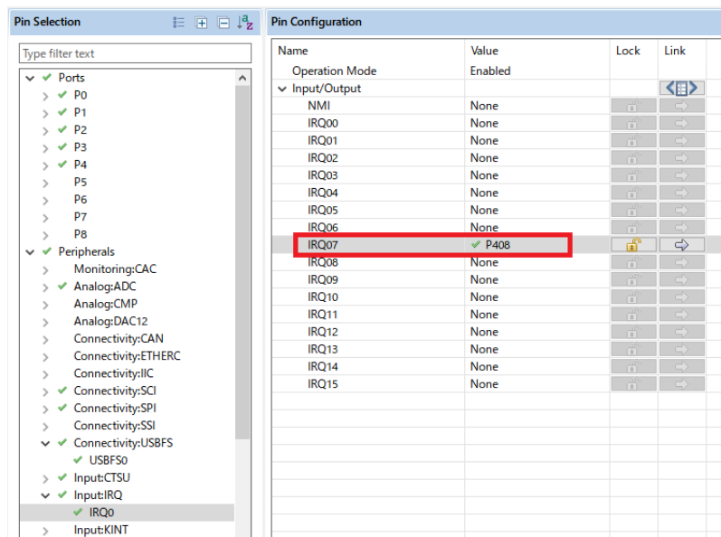
Figure 220: IRQ Pin Setting
