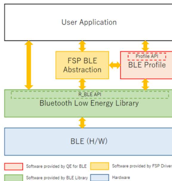
Figure 322: BLE software structure
