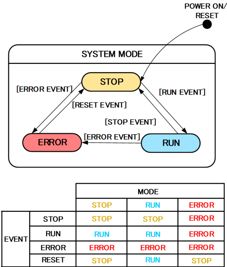
Figure 316: State transition diagram
