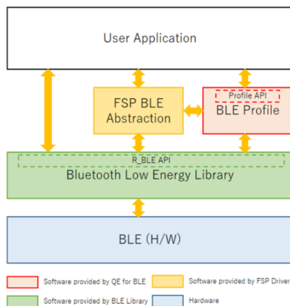
Figure 321: BLE software structure
