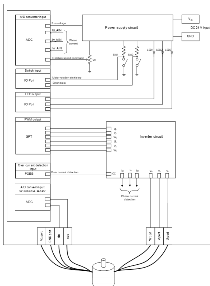
Figure 312: Example of target hardware of motor induction module
