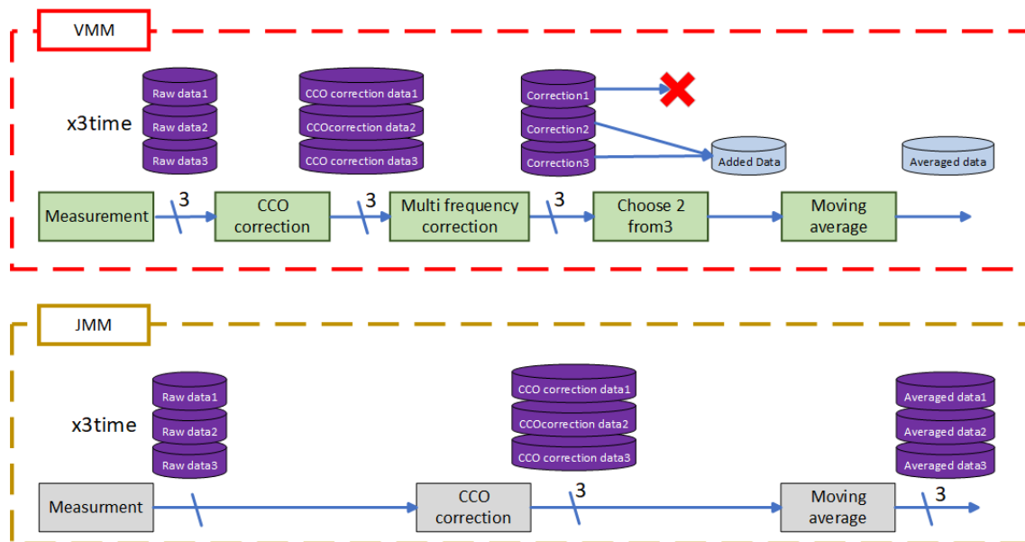
Figure 192: Data flow Comparison of JMM and VMM
