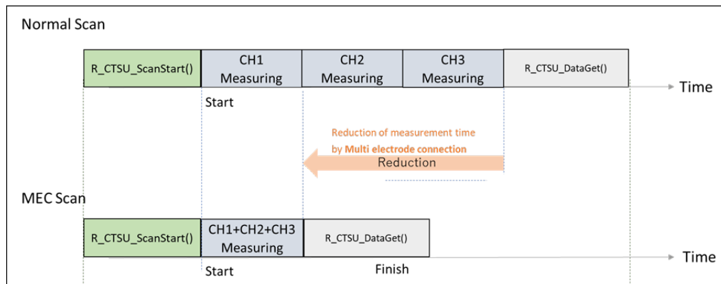
Figure 198: Comparison of time between normal measurement and MEC measurement
