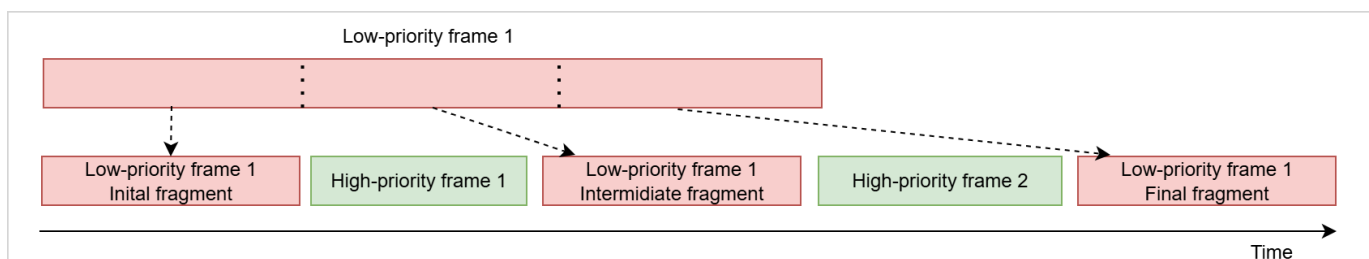
Figure 338: Frame preemption behavior
