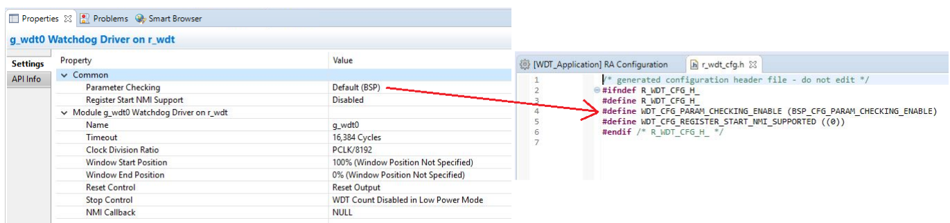
Figure 120: r_wdt_cfg.h contents
