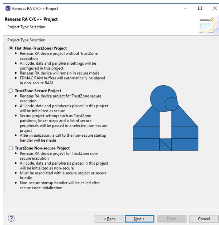
Figure 128: Flat Project
