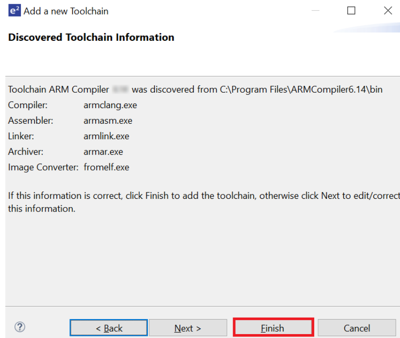
Figure 62: Toolchain Information
