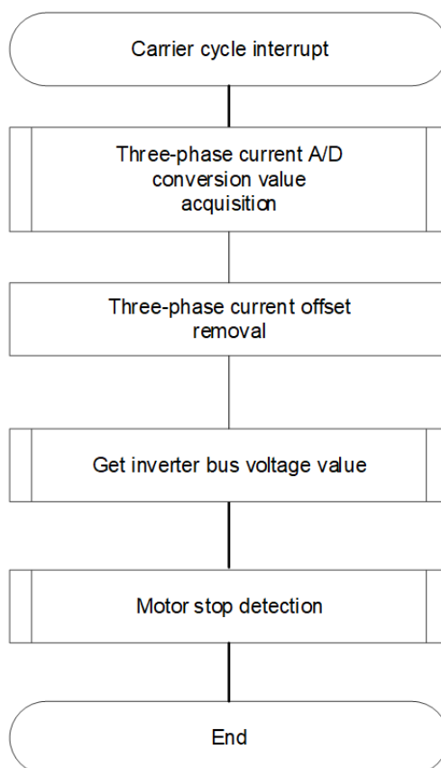
Figure 280: Current control process of 120-degree with hall sensor
