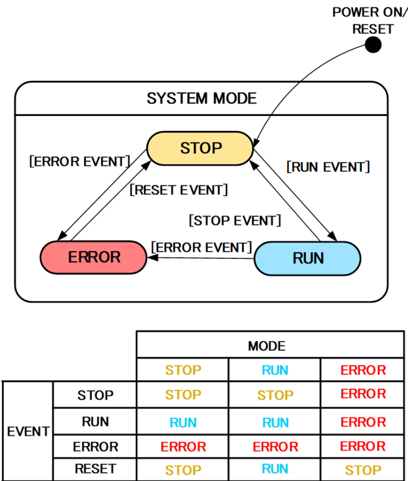
Figure 298: State transition diagram
