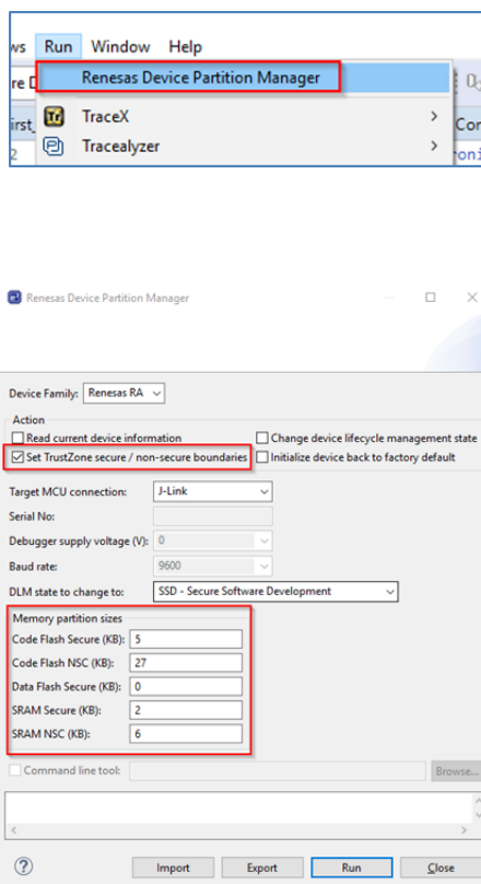
Figure 139: Renesas Device Partition Manager
