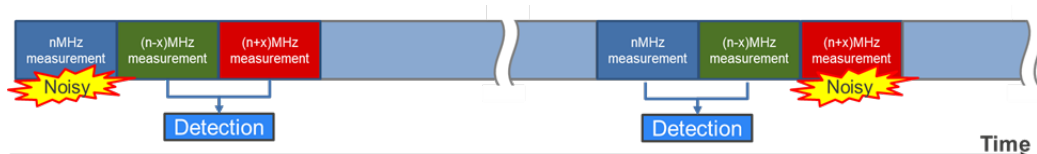
Figure 194: Multi-clock Measurements
