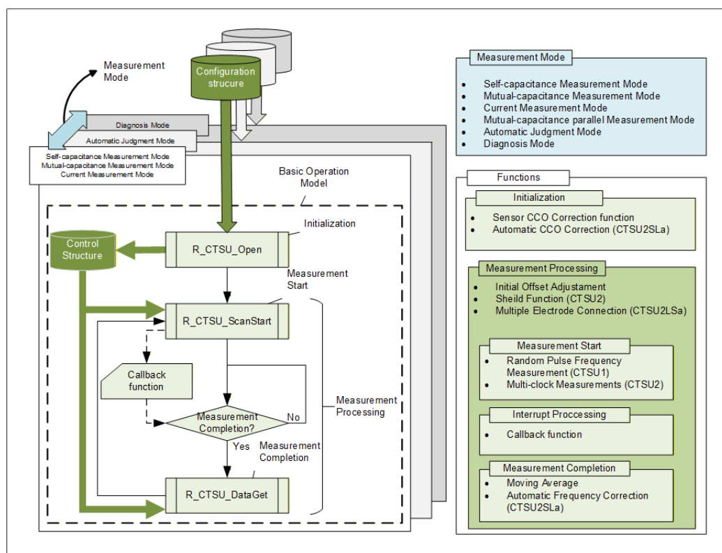
Figure 181: Overview of software system
