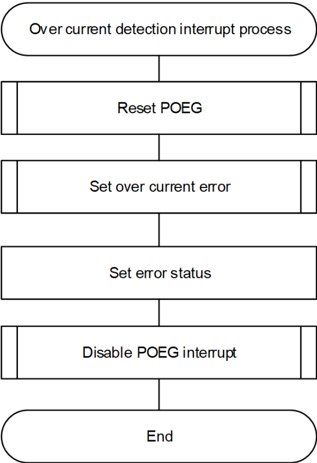
Figure 320: Over current detection interrupt process
