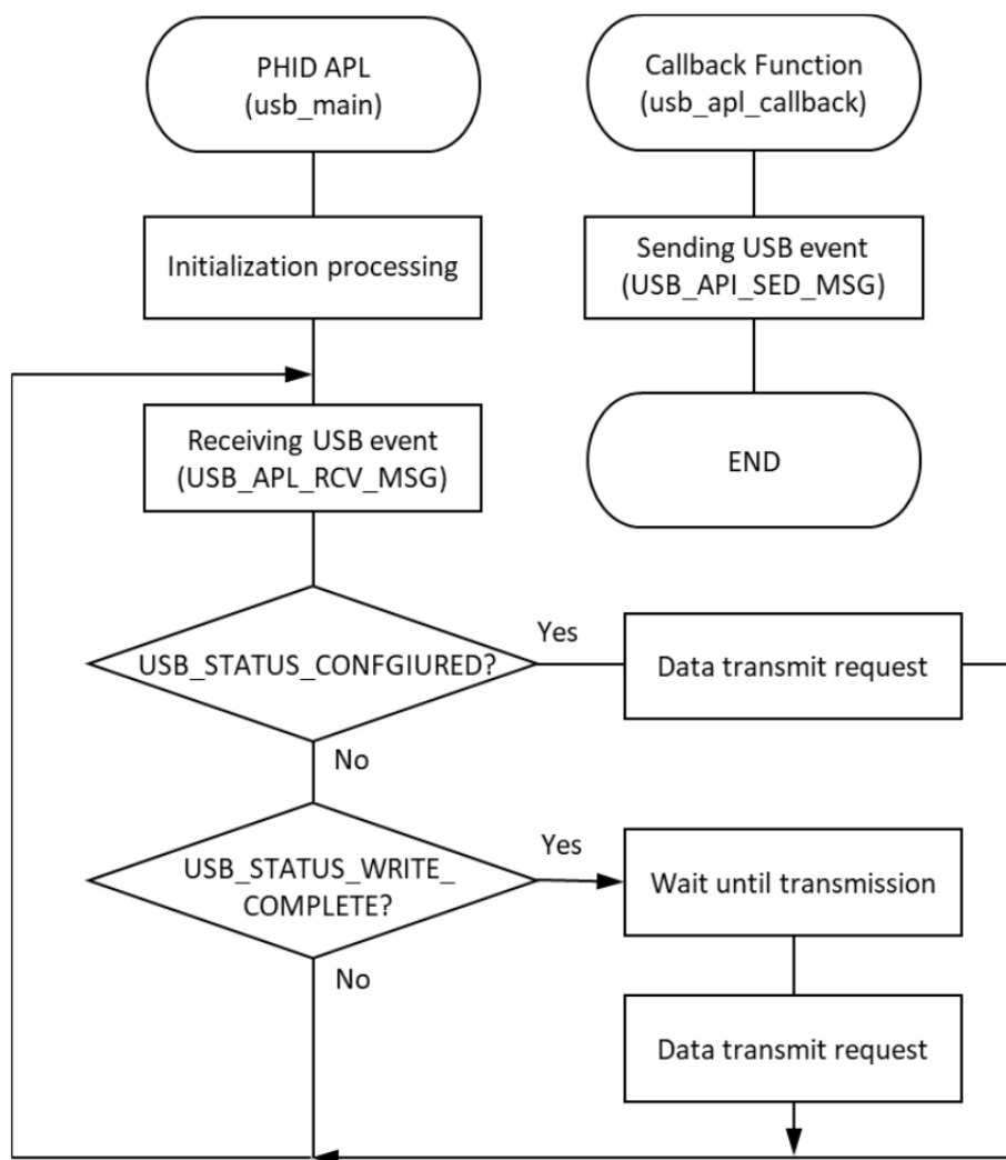
Figure 260: Main Loop processing for RTOS example
