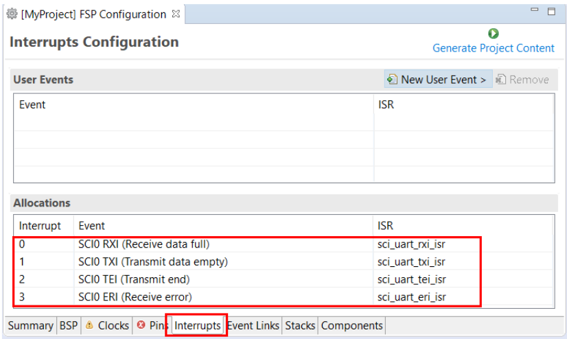
Figure 29: Configuring interrupt in Interrupt Tab
