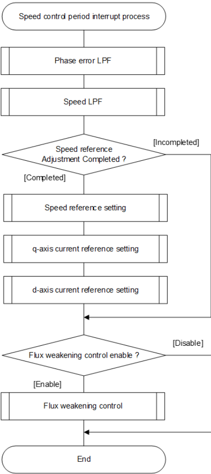
Figure 310: Speed control process
