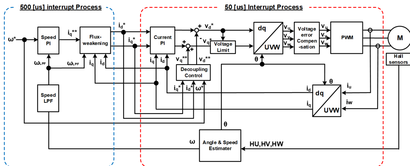
Figure 304: Block diagram of vector control with hall sensors
