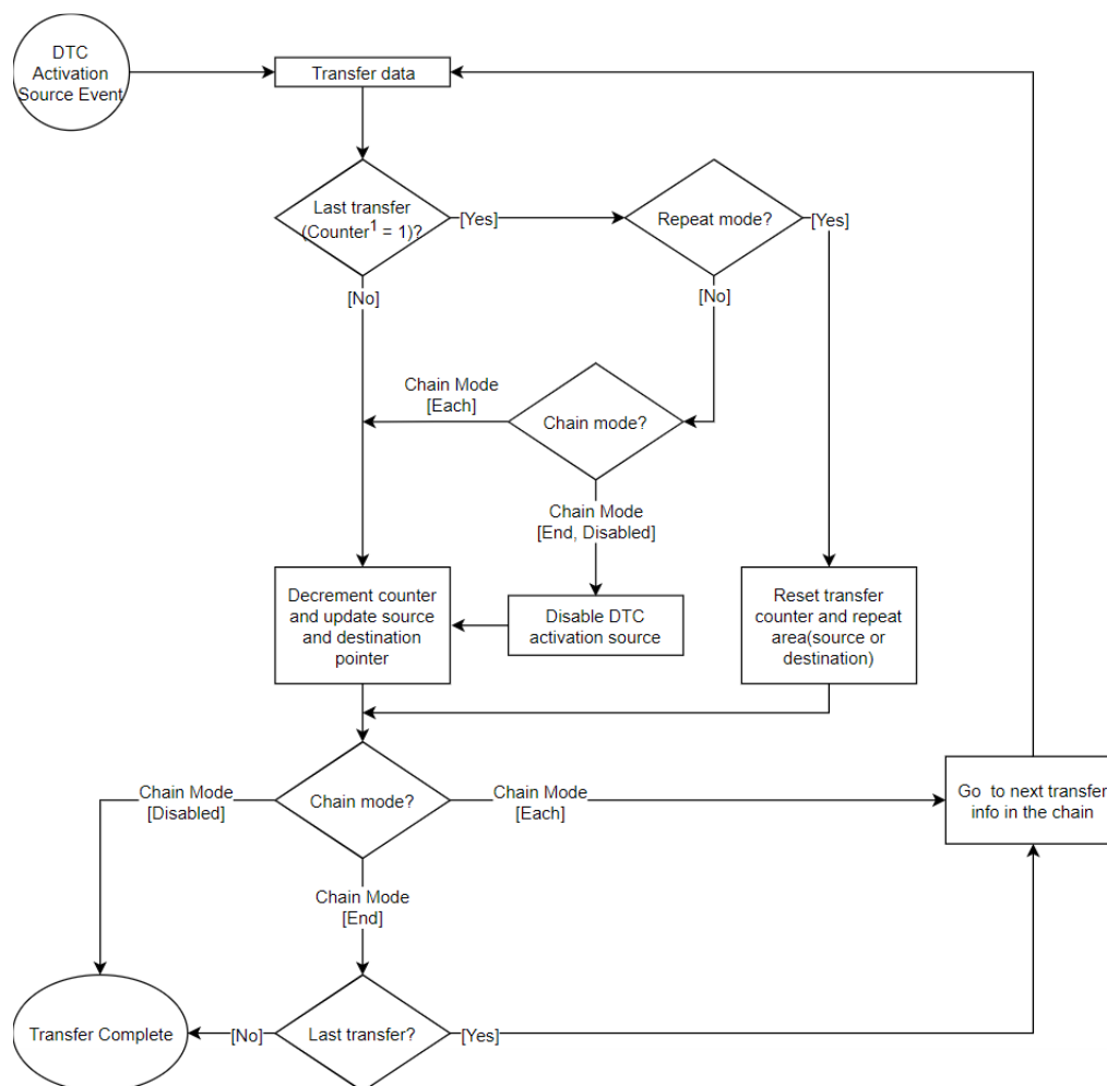
Figure 369: DTC Transfer Flowchart
