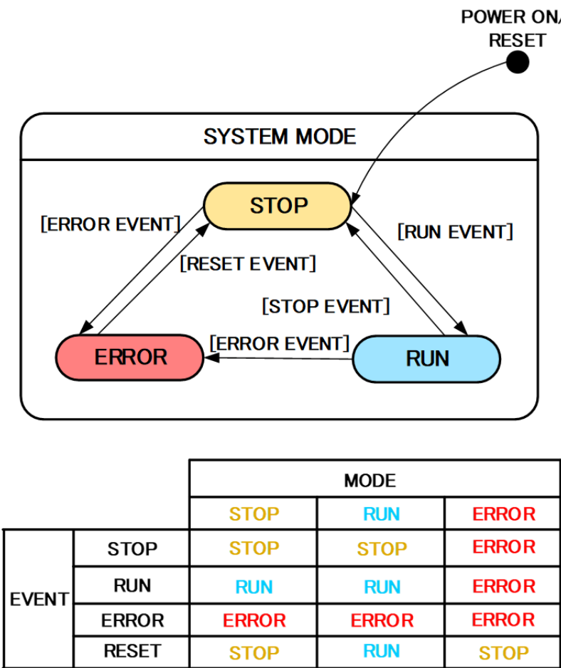
Figure 287: State transition diagram
