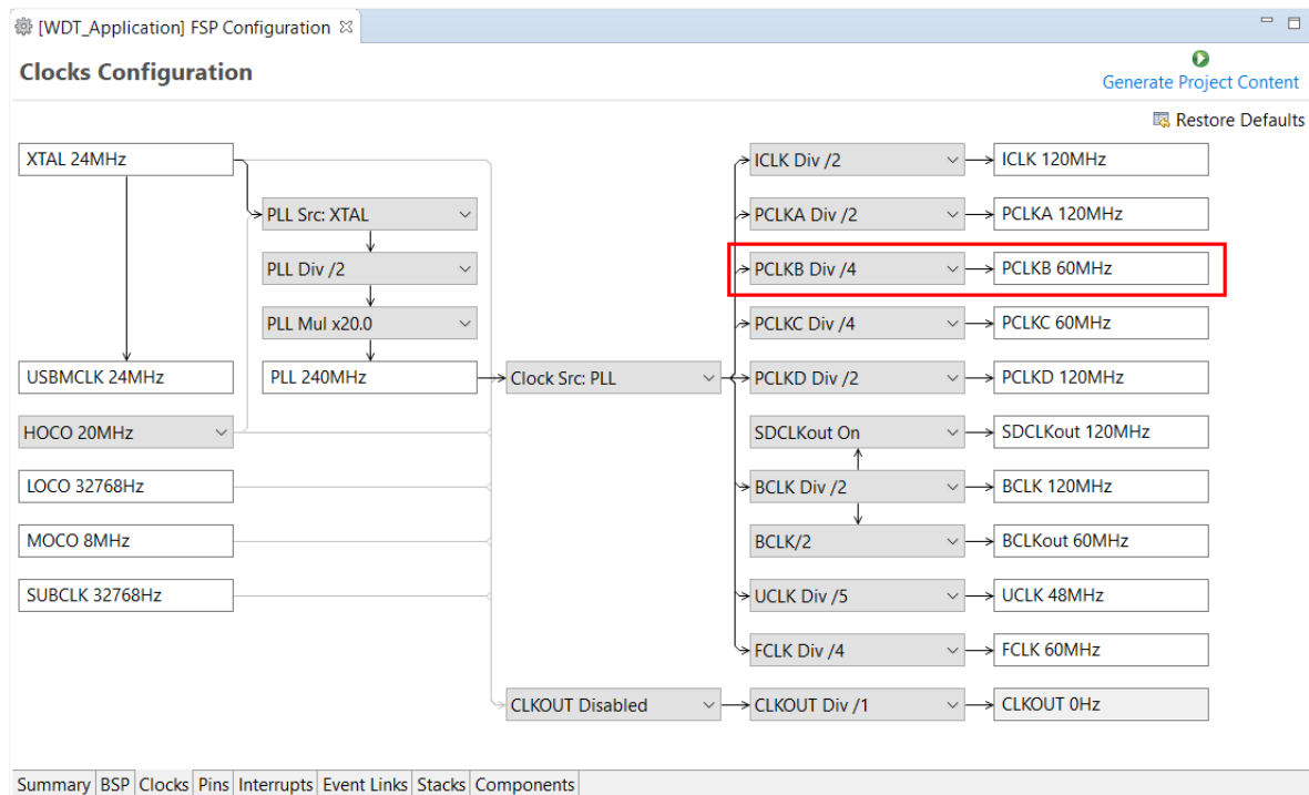
Figure 113: Clock configuration
