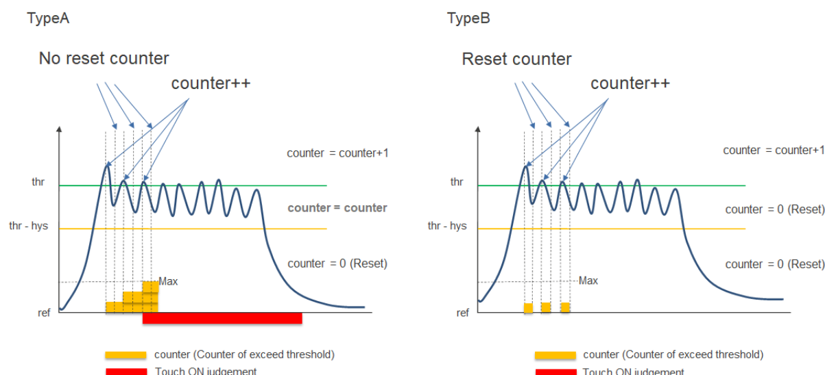
Figure 202: Chattering suppression type
