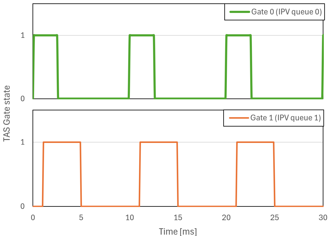
Figure 336: TAS operation image
