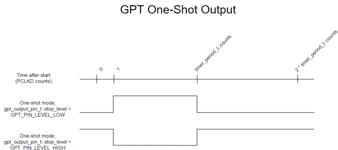
Figure 357: GPT One-Shot Output
