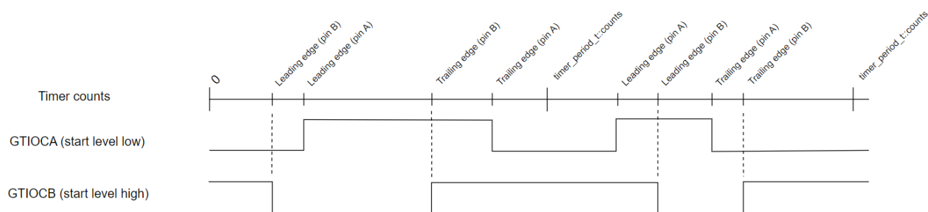
Figure 358: GPT One-Shot Pulse Output (without dead time)
