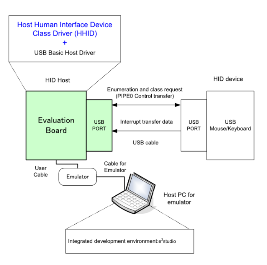
Figure 247: Example Operating Environment
