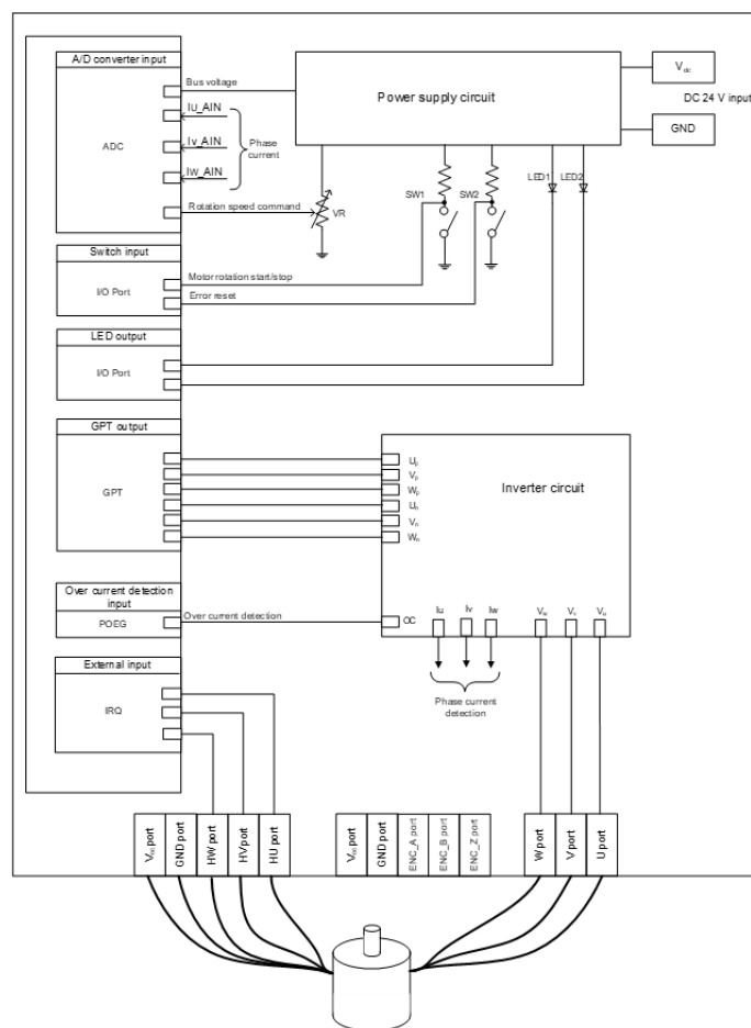
Figure 274: Example of target hardware of motor 120-degree with hall sensor
