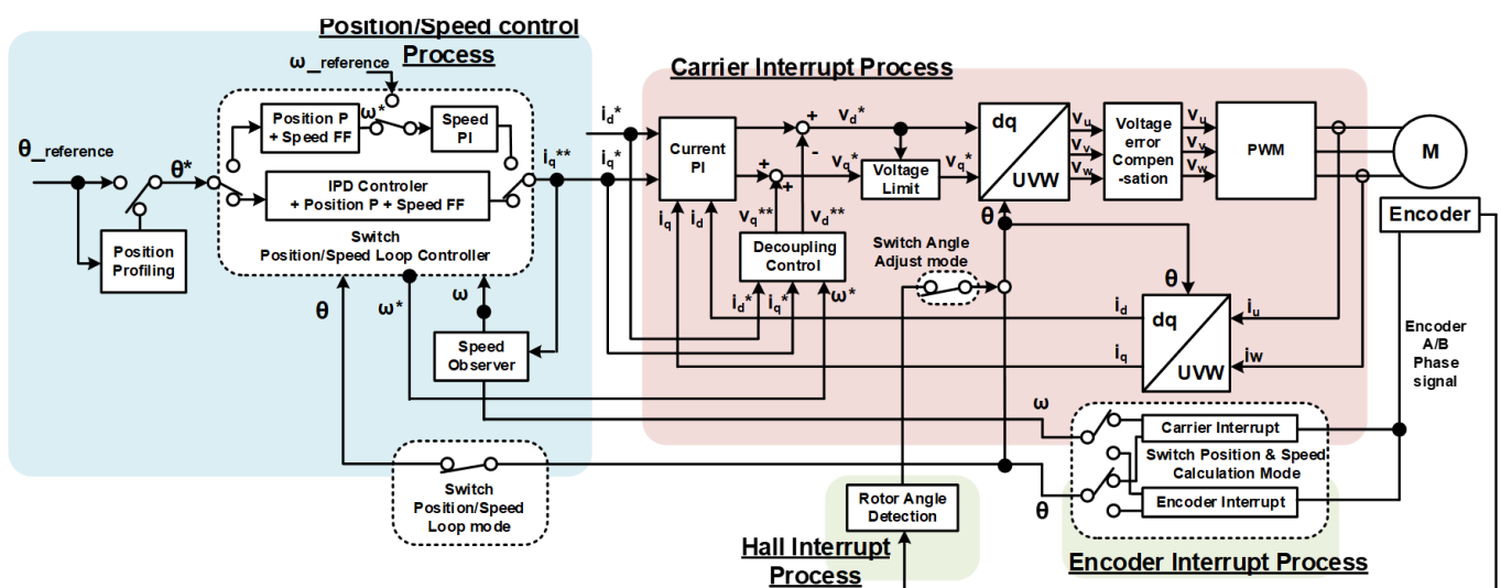
Figure 284: Block diagram of encoder vector control (PI feedback loop)
