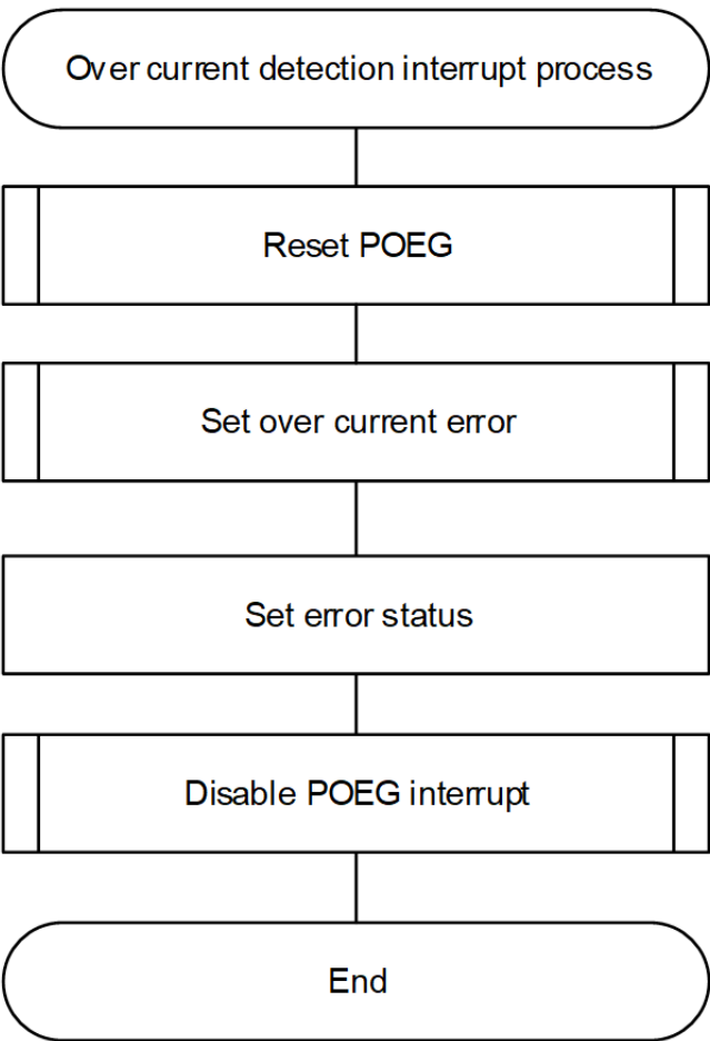
Figure 311: Over current detection interrupt process
