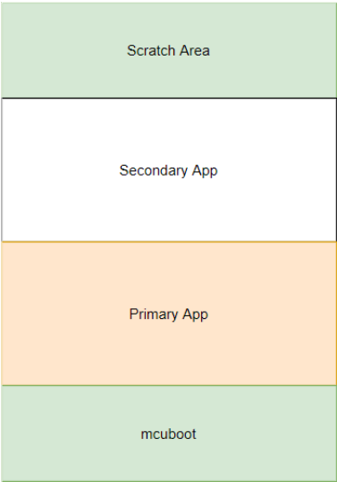
Figure 177: MCUboot Memory Map
