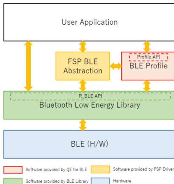
Figure 323: BLE software structure
