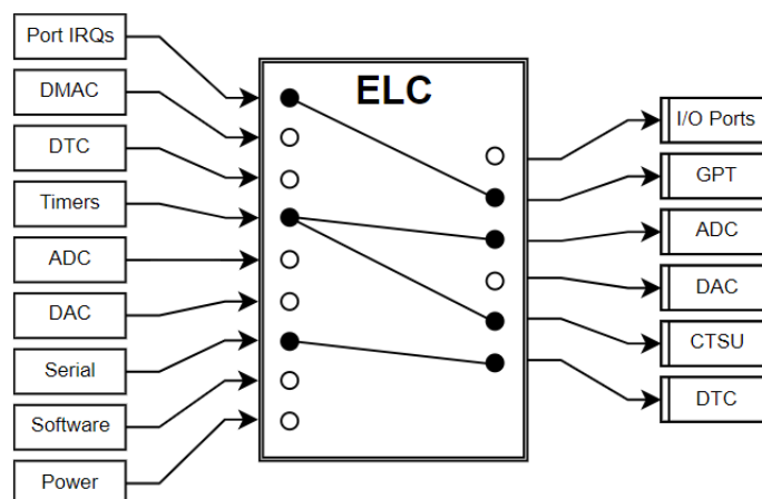
Figure 355: Event Link Controller Conceptual Diagram
