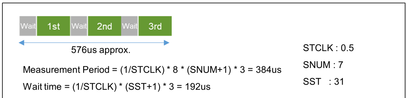
Figure 183: Self-capacitance Measurement Period (CTS2)
