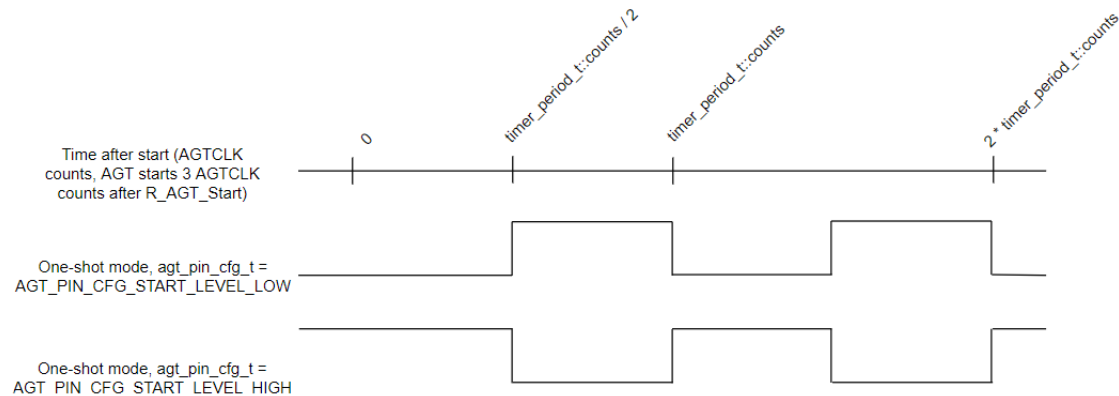
Figure 365: AGT Periodic Output
