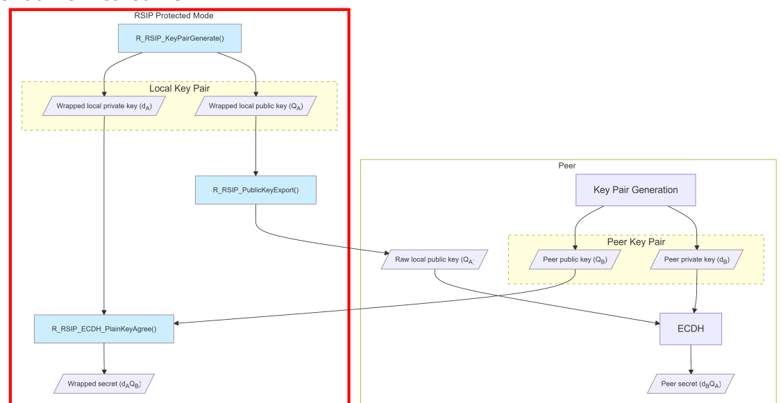
Figure 345: Unauthenticated ECDHE flow
