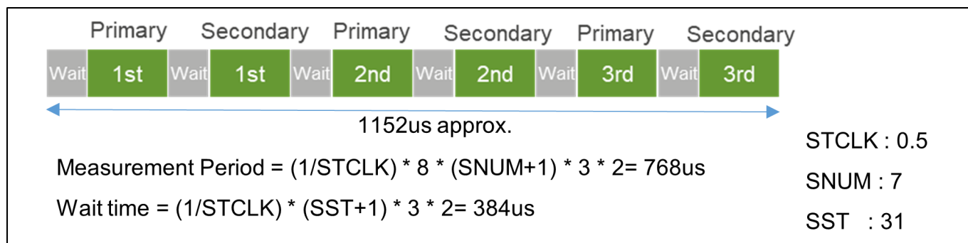
Figure 184: Mutual-capacitance Measurement Period (CTS2U2)
