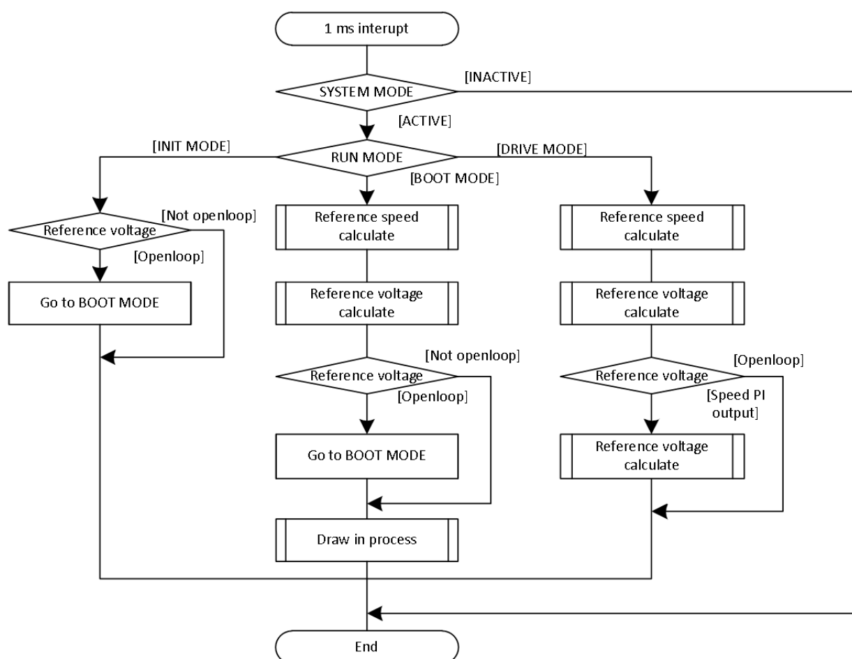
Figure 279: Speed control process of 120-degree sensorless
