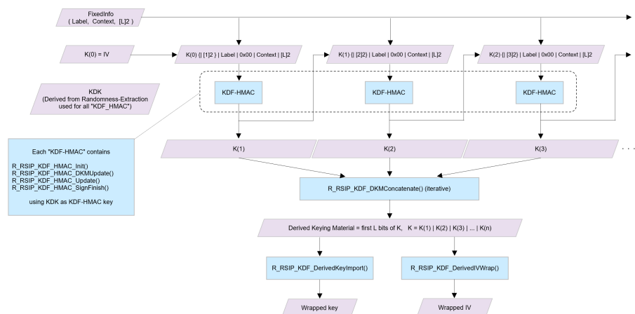
Figure 348: Two-Step Key Derivation Key Expansion flow
