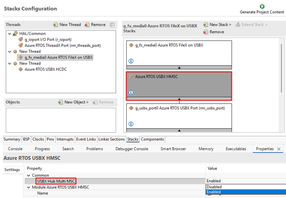
Figure 226: Enable Hub Multi MSC
