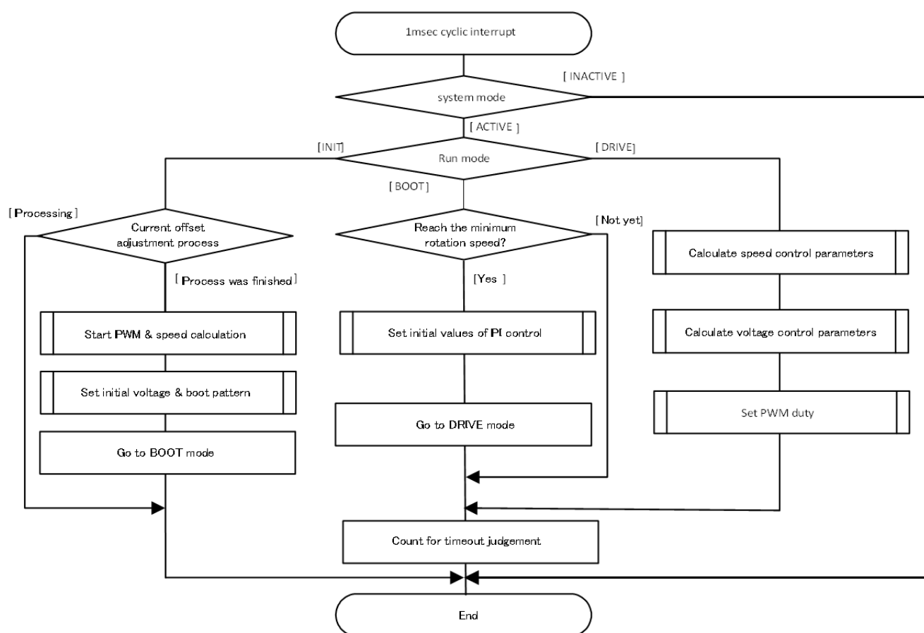
Figure 281: Speed control process of 120-degree with hall sensor
