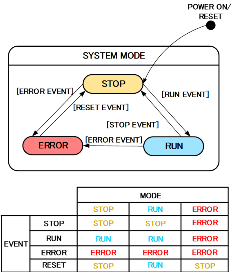
Figure 276: State transition diagram
