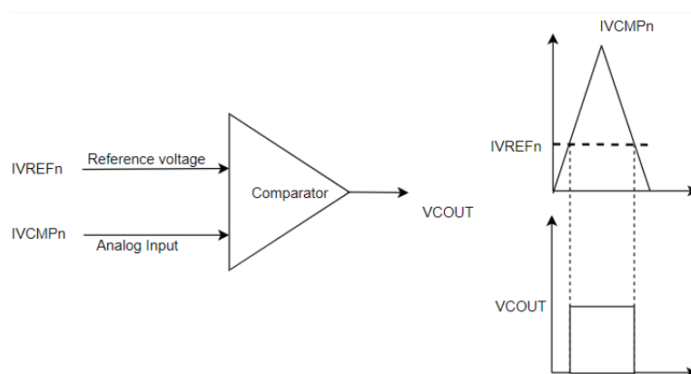
Figure 167: ACMPLP Standard Mode Operation
