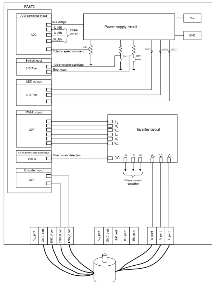
Figure 283: Example of target hardware of motor encoder module
