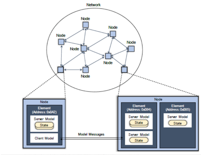
Figure 324: Overview Of Bluetooth Mesh
