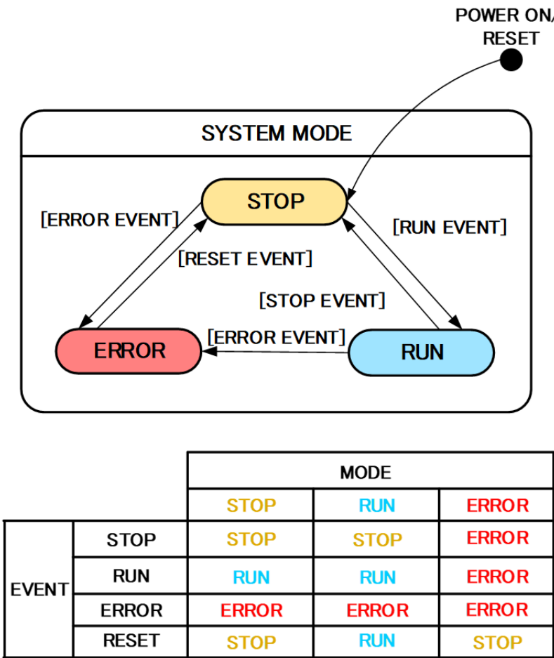
Figure 307: State transition diagram
