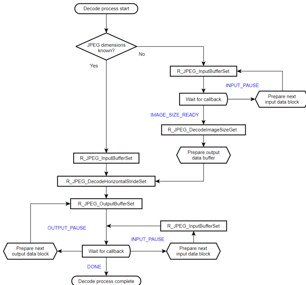
Figure 267: JPEG Decode Operational Flow
