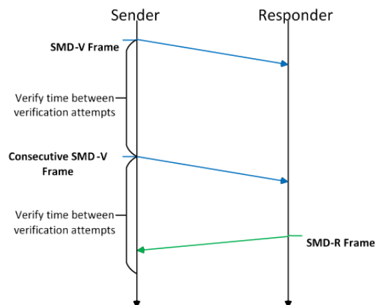
Figure 337: Frame preemption verification
