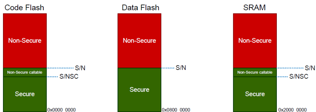
Figure 123: Secure and Non-Secure Regions
