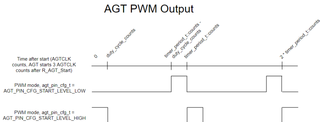
Figure 366: AGT PWM Output
