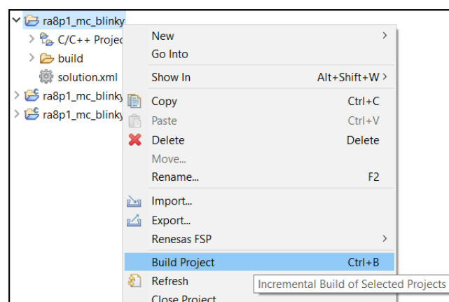
Figure 94: Solution Build
