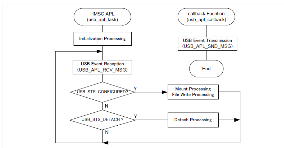
Figure 253: usb_apl_task
