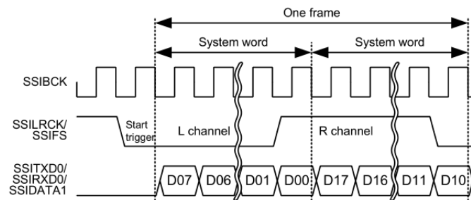
Figure 232: SSI Frame Diagram (8-bit word, 8-bit samples)
