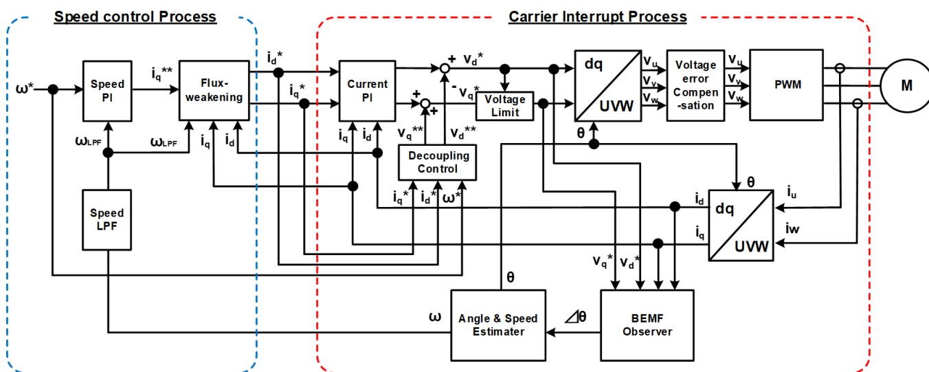
Figure 295: Block diagram of sensorless vector control (PI feedback loop)
