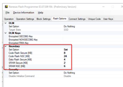
Figure 149: RFP Partition Boundaries
