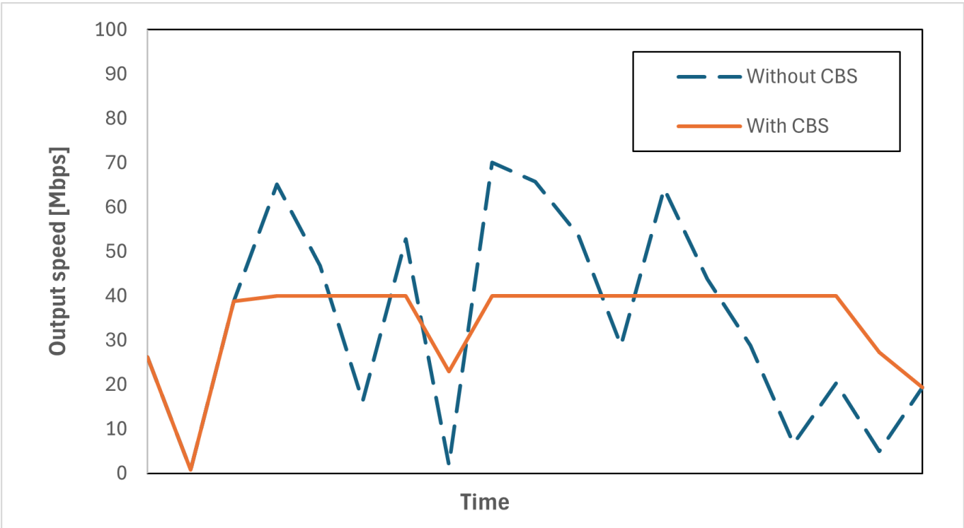
Figure 335: CBS operation image
