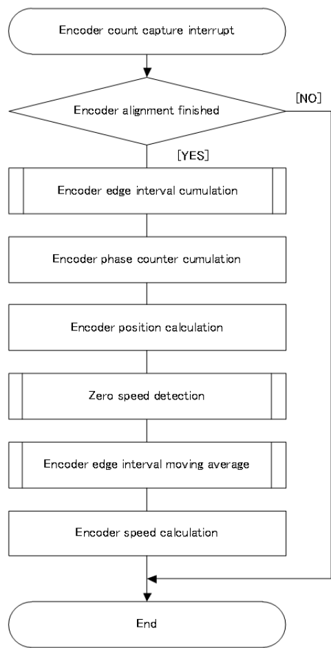
Figure 291: Encoder interrupt process
