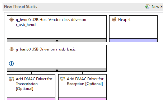
Figure 255: USB Host Vendor Class Stack
