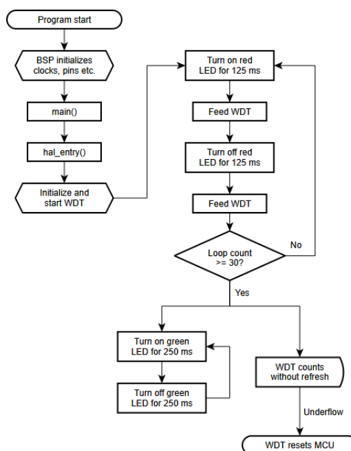
Figure 105: WDT Application flow diagram
