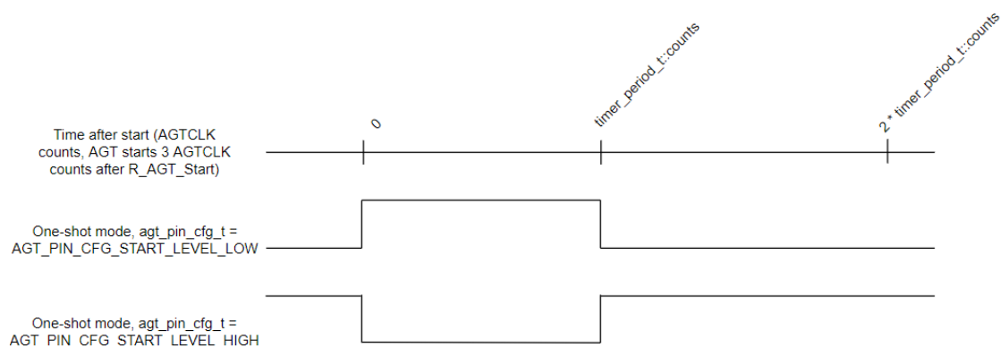
Figure 364: AGT One-Shot Output
