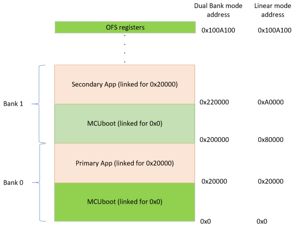
Figure 173: MCUboot Dual Bank layout of Flash HP for 1 MB Memory
