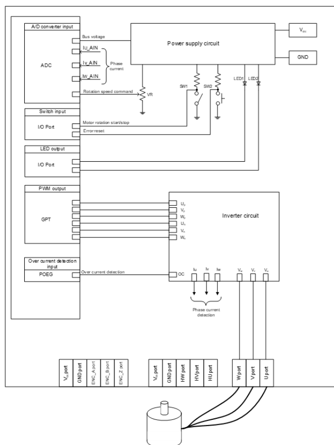
Figure 293: Example of target hardware of motor sensorless module
