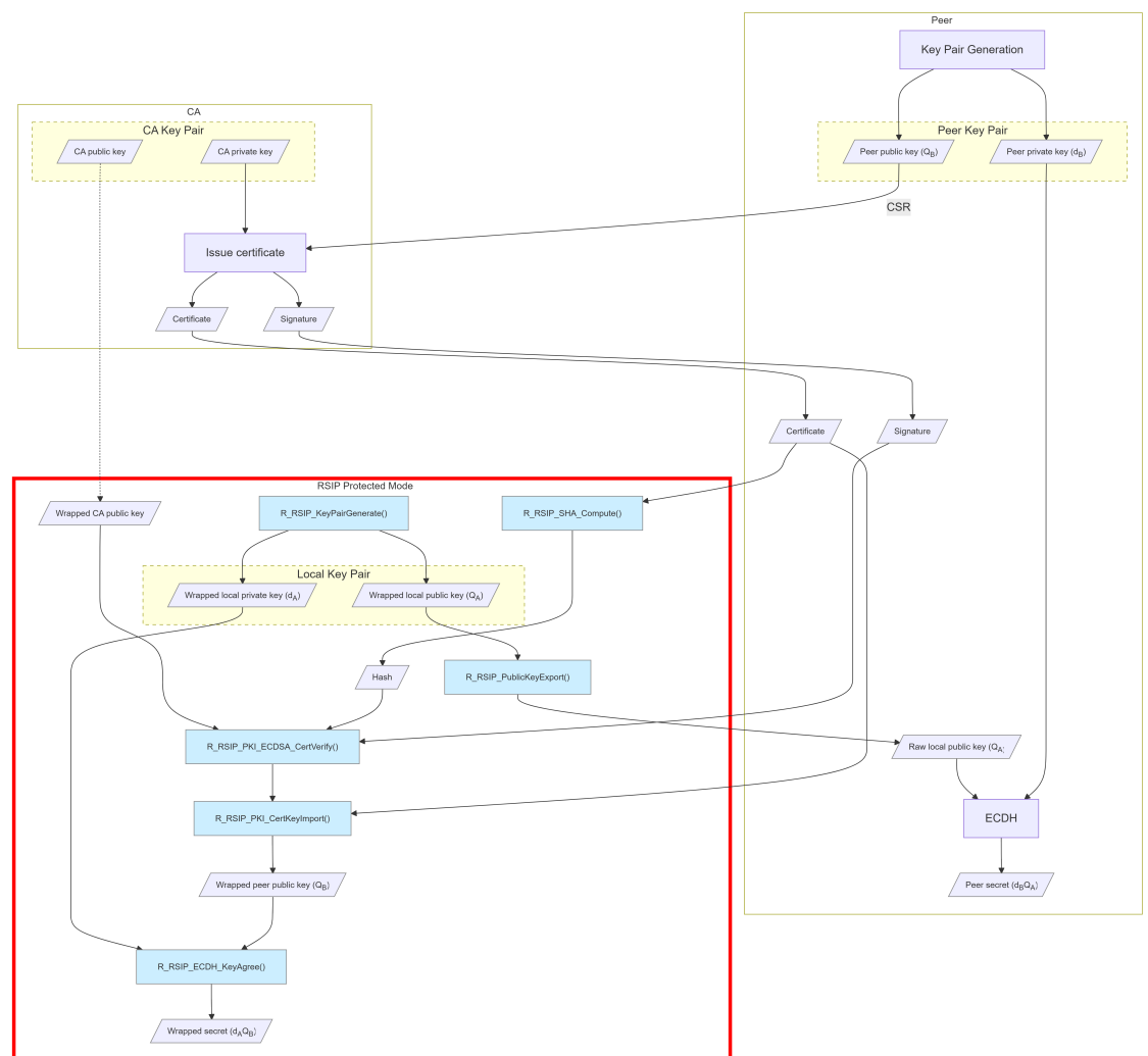
Figure 344: Authenticated ECDH flow
