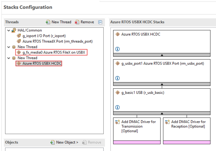
Figure 222: Add HMSC & HCDC Stack
