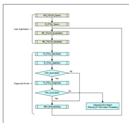
Figure 190: Example flow when using diagnosis mode (CTSU1)
