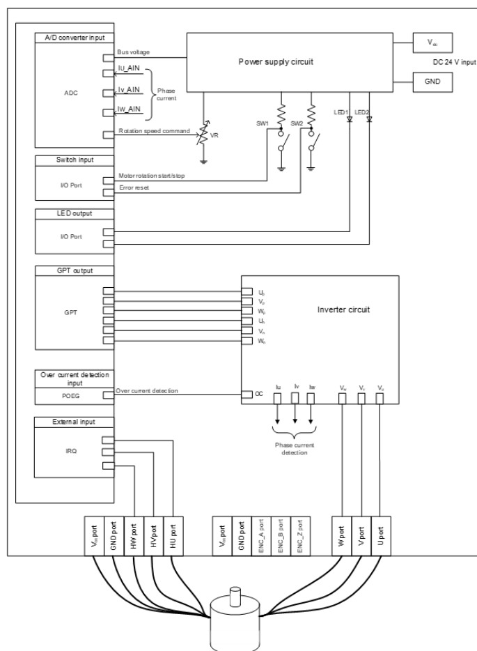
Figure 303: Example of target hardware of motor hall module
