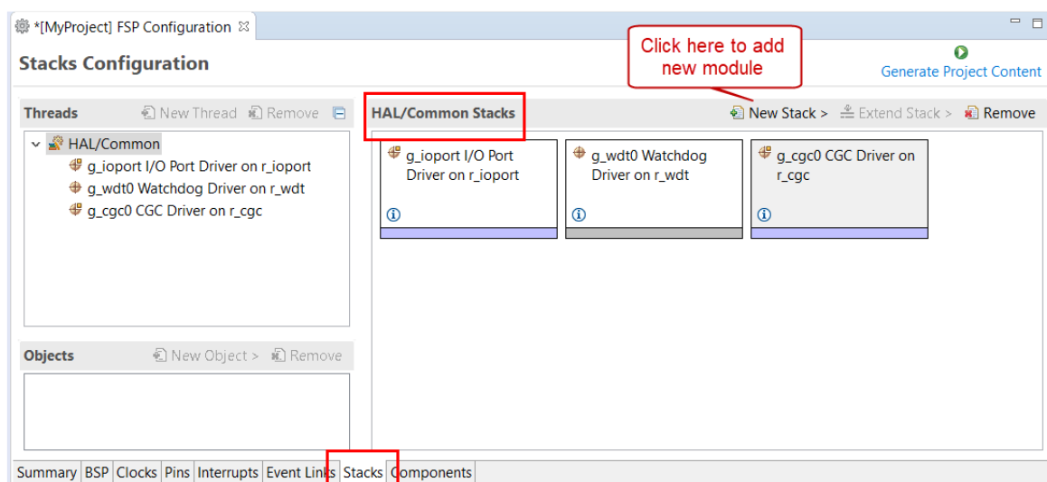
Figure 34: e² studio Project configurator - Adding drivers
