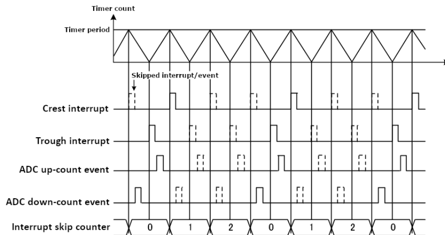
Figure 363: Crest interrupt skipping in triangle-wave PWM modes (skip count 2)
