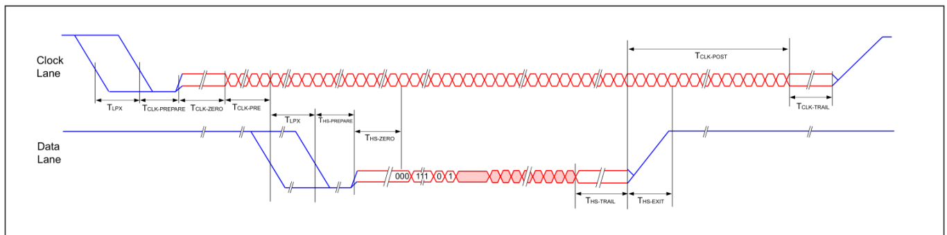
Figure 269: High-Speed data transmission in normal mode
