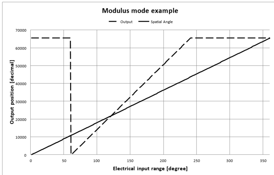
Figure 6. Modulus Output Example with Slope = 2, Offset = 60°
