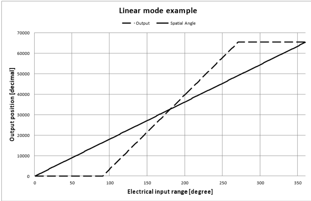
Figure 5. Linear Output Mode Example with Slope = 2, Offset = 90°
