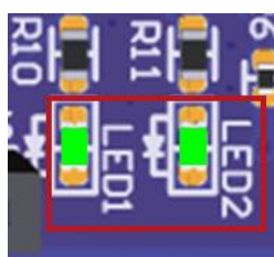
Figure 15. User LEDs (FPB-RA2T1 Top View)
