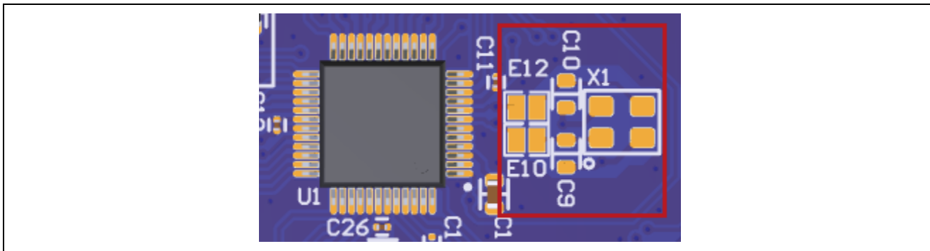
Figure 21. Main-clock Oscillation Circuit (FPB-RA2T1 Top View)
