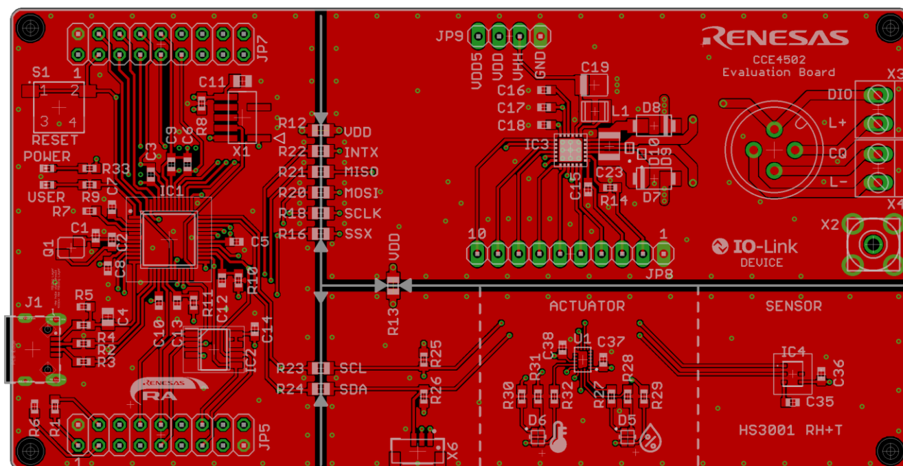
Figure 8. Top Layer
