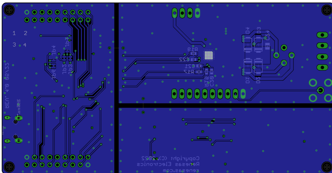
Figure 11. Bottom Layer
