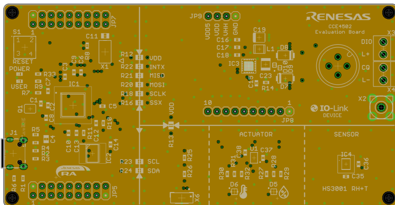
Figure 9. Second Layer (GND)
