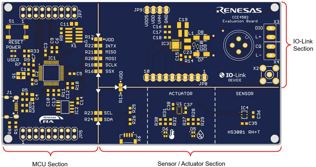
Figure 3. Sections Overview
