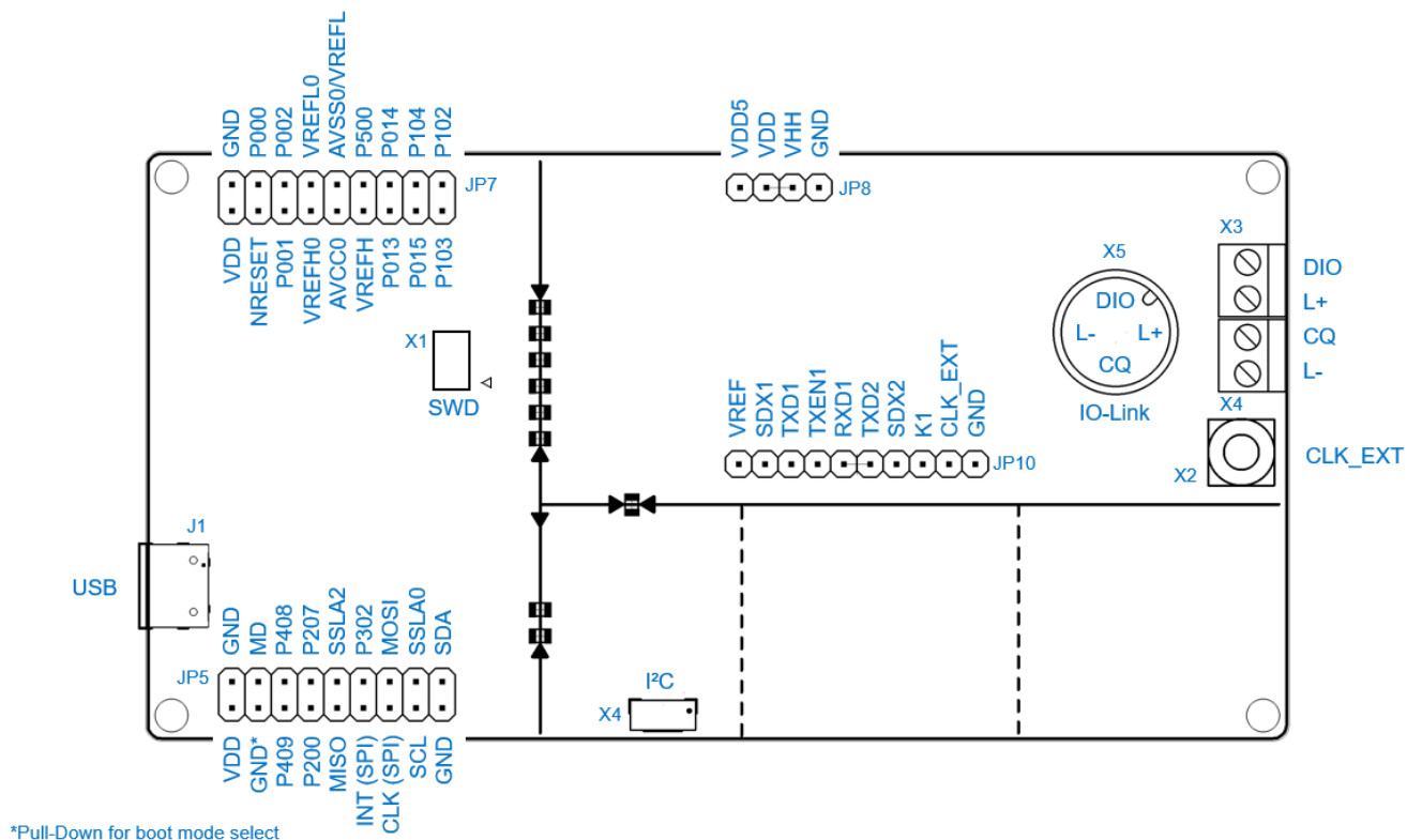
Figure 4. Connectors
