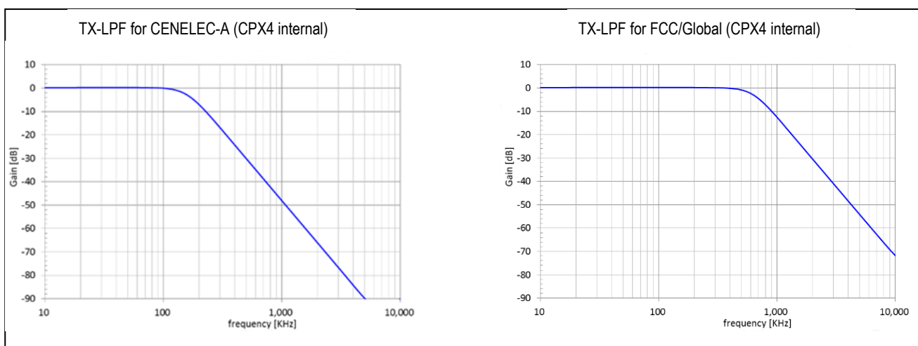
Figure 2-4 TX-PLF (CPX4 internal)
