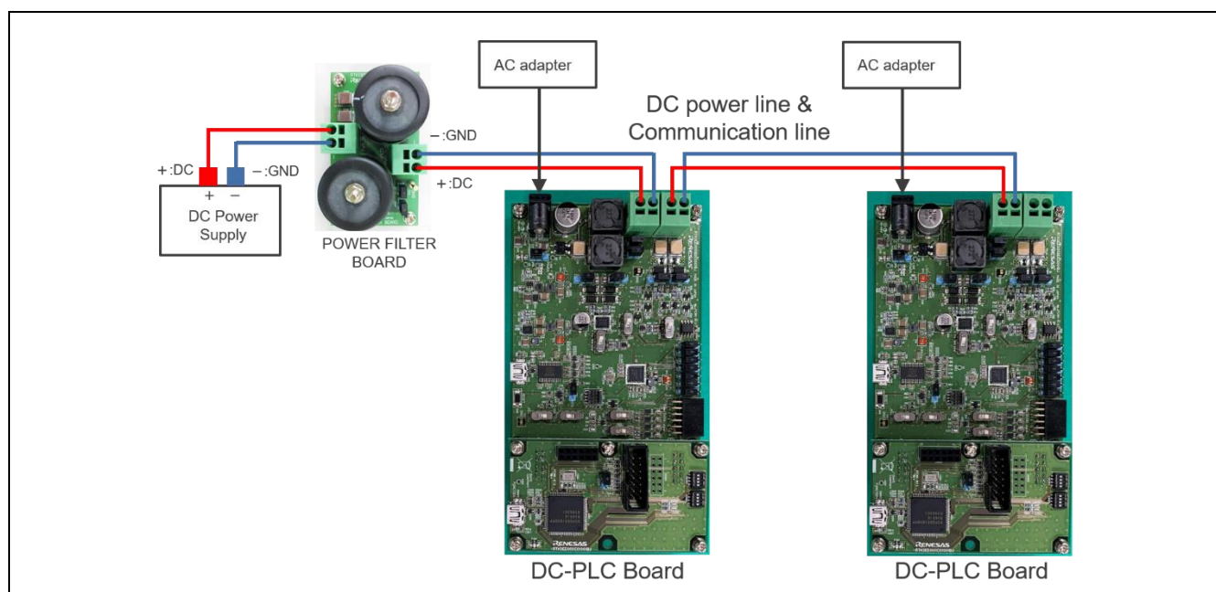
Figure 2-3 Connection example when voltage is applied to communication line (Board power is supplied from AC adapter)
