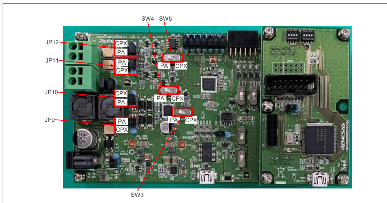
Figure 2-6 Drive method setting points
