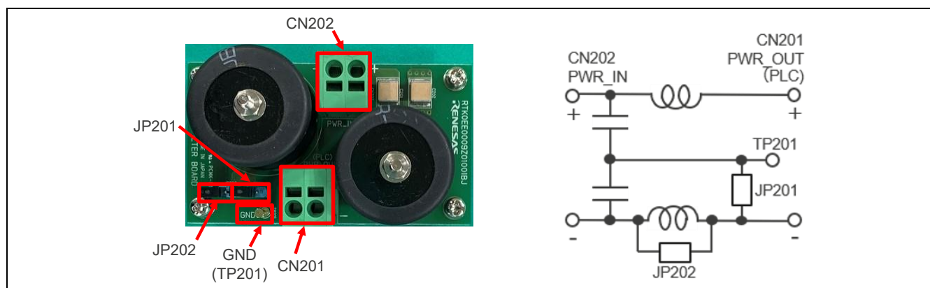
Figure 3-4 Connectors, JPs, and TP of Power filter board
