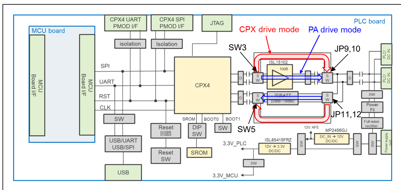
Figure 2-5 CPX drive and PA drive
