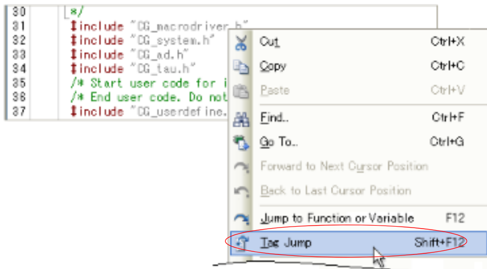
Figure 2.15 Tag Jump
