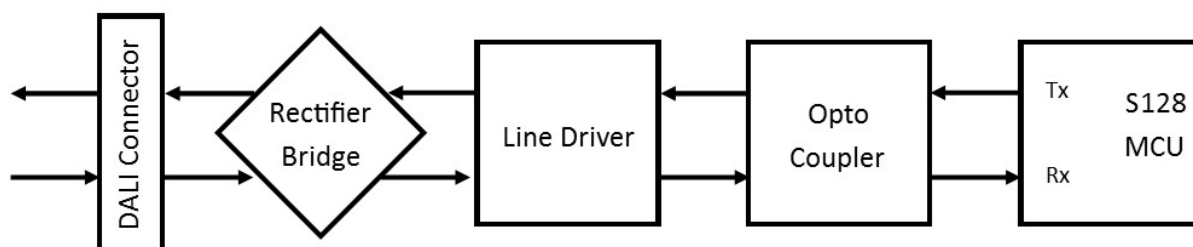
Figure 22. DALI Interface Circuit Block Diagram
