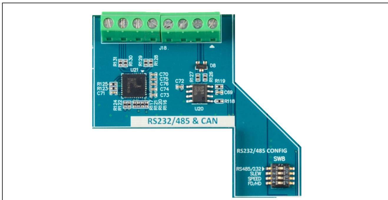
Figure 12. RS232/485 and CAN Interface
