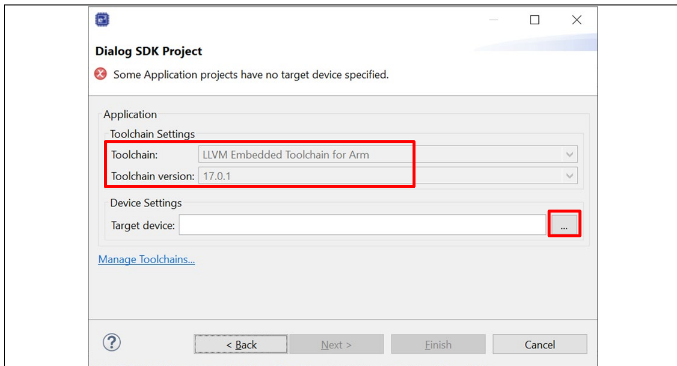
Figure 3-35 Selecting the Toolchain, Its Version, and the Target Device
