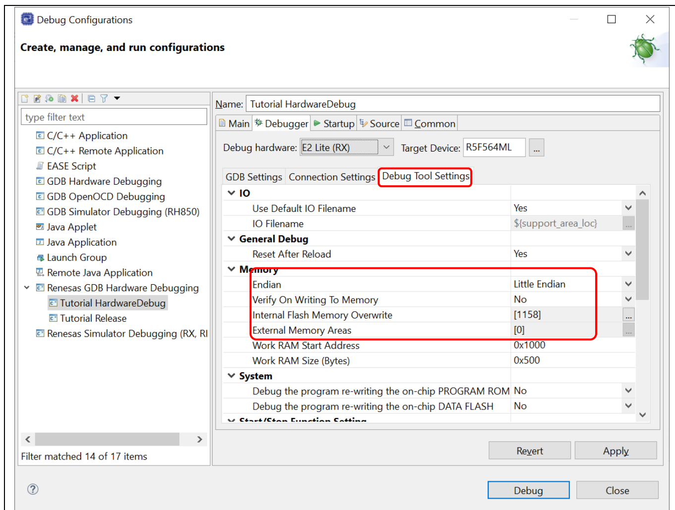
Figure 5-6 Change Debug Tool Settings
