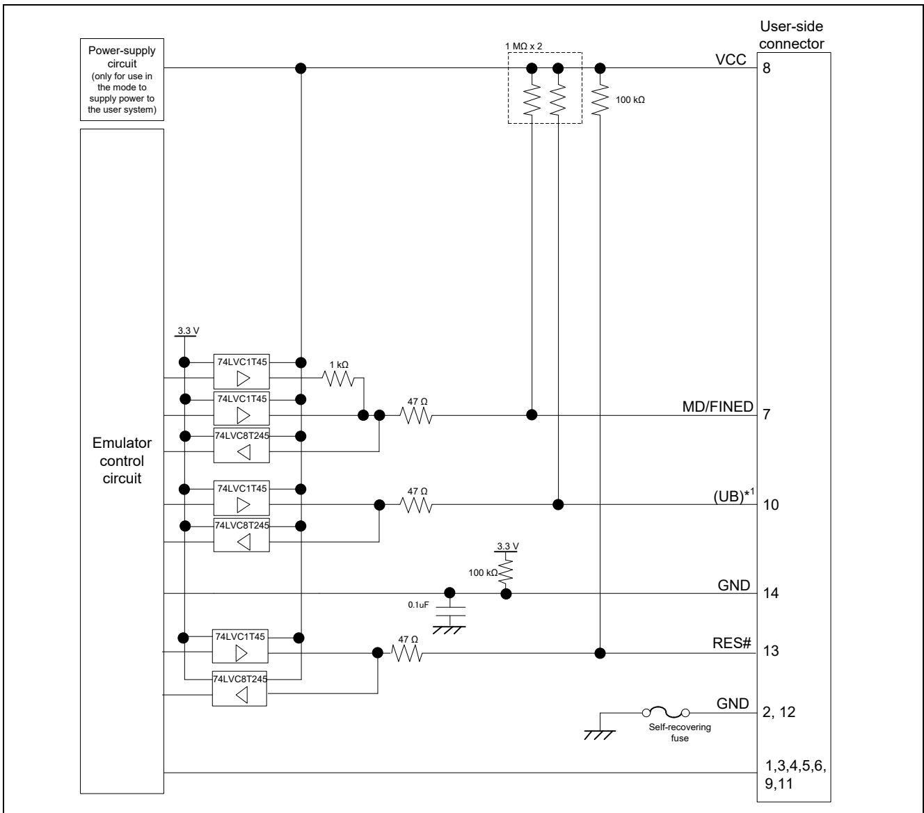
Figure 2.34 Internal Circuits of the E2 with MCUs of the RX200 Series and RX100 Series Connected via the FINE Interface
