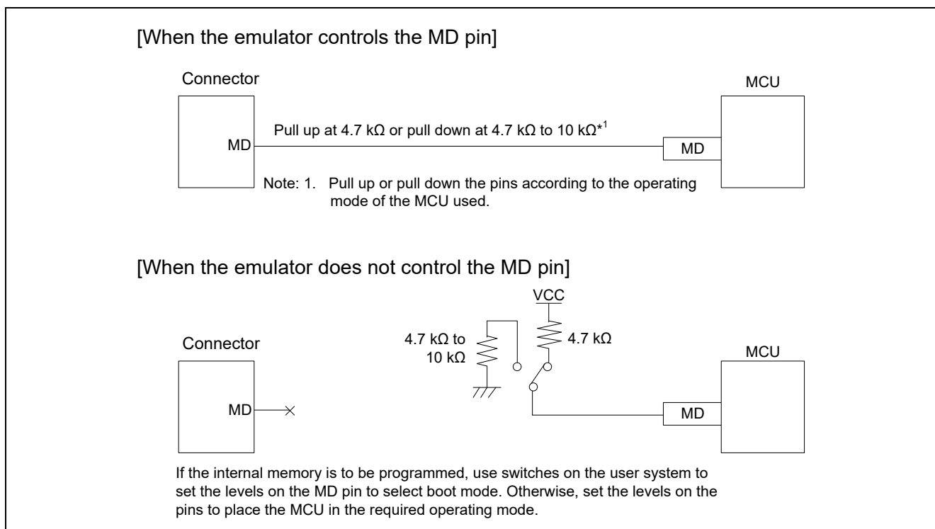
Figure 2.21 Connection of the MODE Pin (JTAG Interface Connection for the RX63x, RX64x, RX65x, RX66x, RX67x, RX71x, and RX72x Groups)
