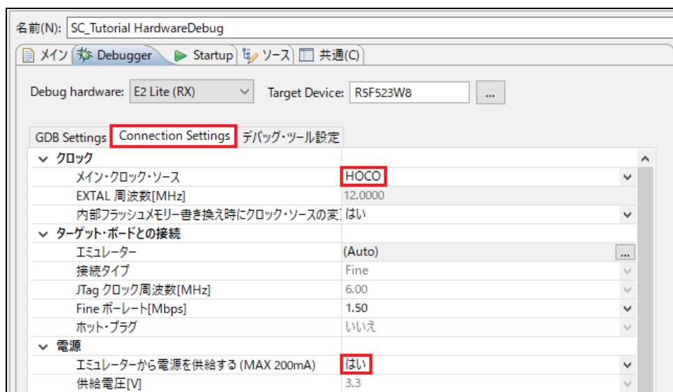
図 6-2 Connection Settings
