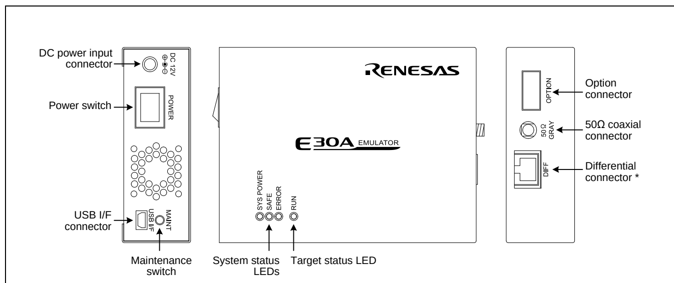
Figure 1.2 Names and Functions of Each Part of the Emulator
