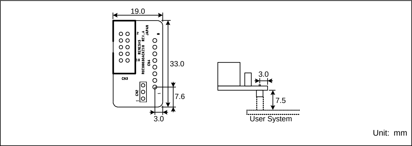
Figure F.3 External Dimensions of the Option Board
