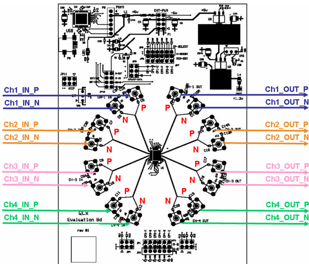
FIGURE 3. OLx4270 EVALUATION BOARD RF-I/O INTERFACE
