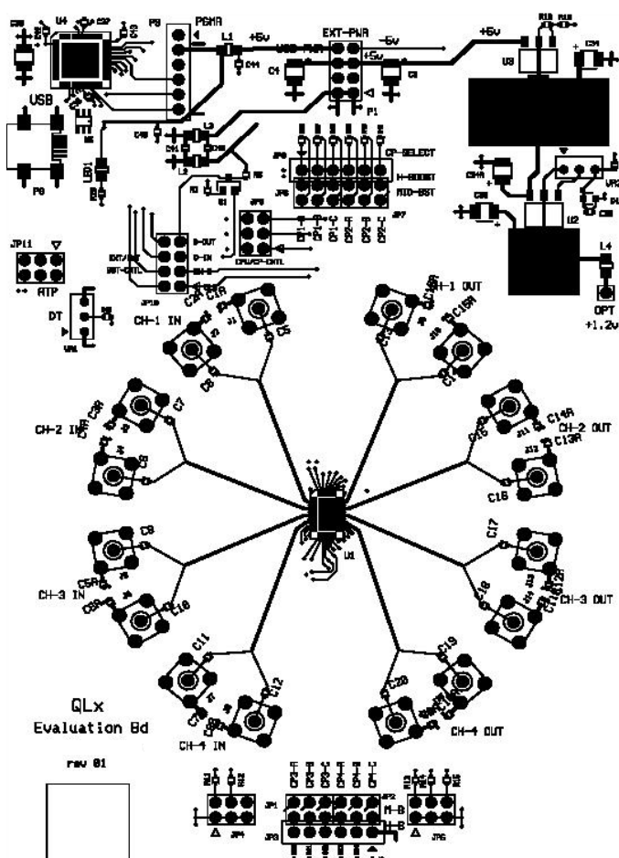
FIGURE 1. QLx4270 EVALUATION BOARD PCB OUTLINE
