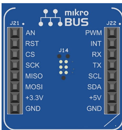
Figure 17. mikroBUS Connector
