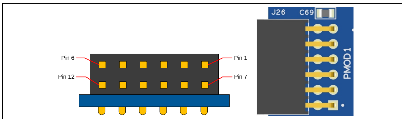
Figure 11. Pmod 1 Connector
