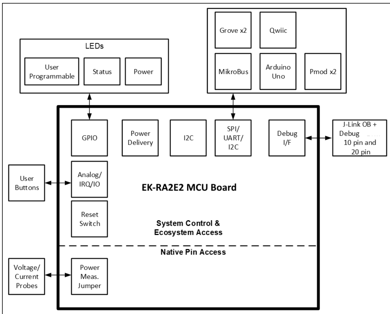
Figure 5. EK-RA2E2 Board Block Diagram
