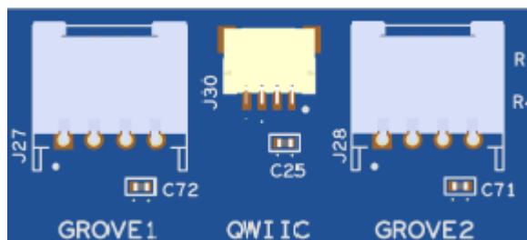
Figure 10. Seeded Grove and Qwiic Connectors
