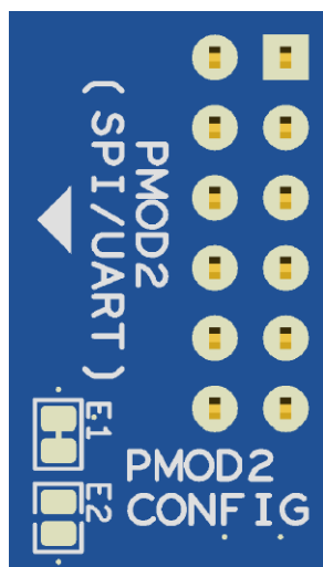
Figure 15. Pmod 2 Trace Cut Jumpers
