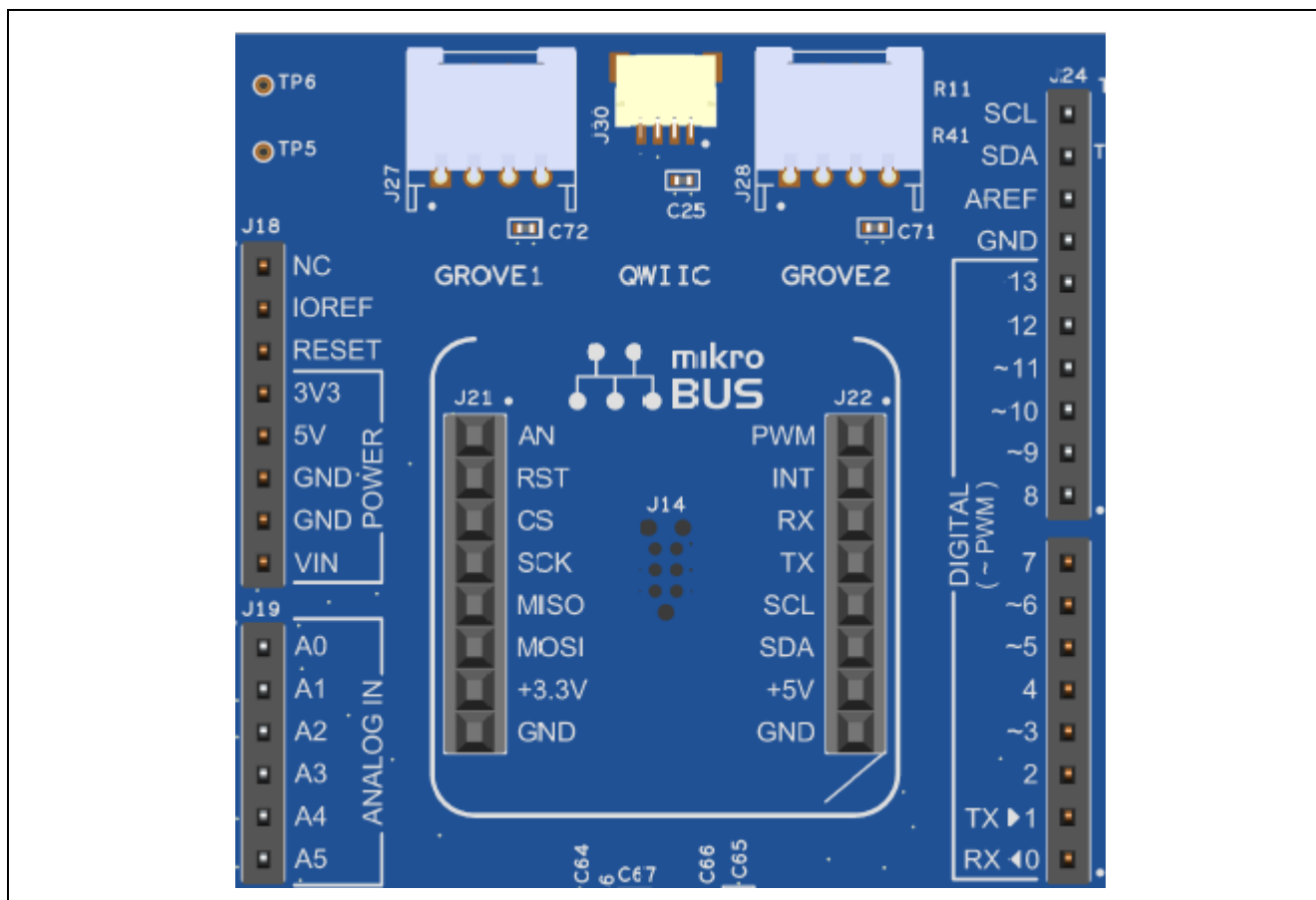
Figure 16. Arduino Uno Connector
