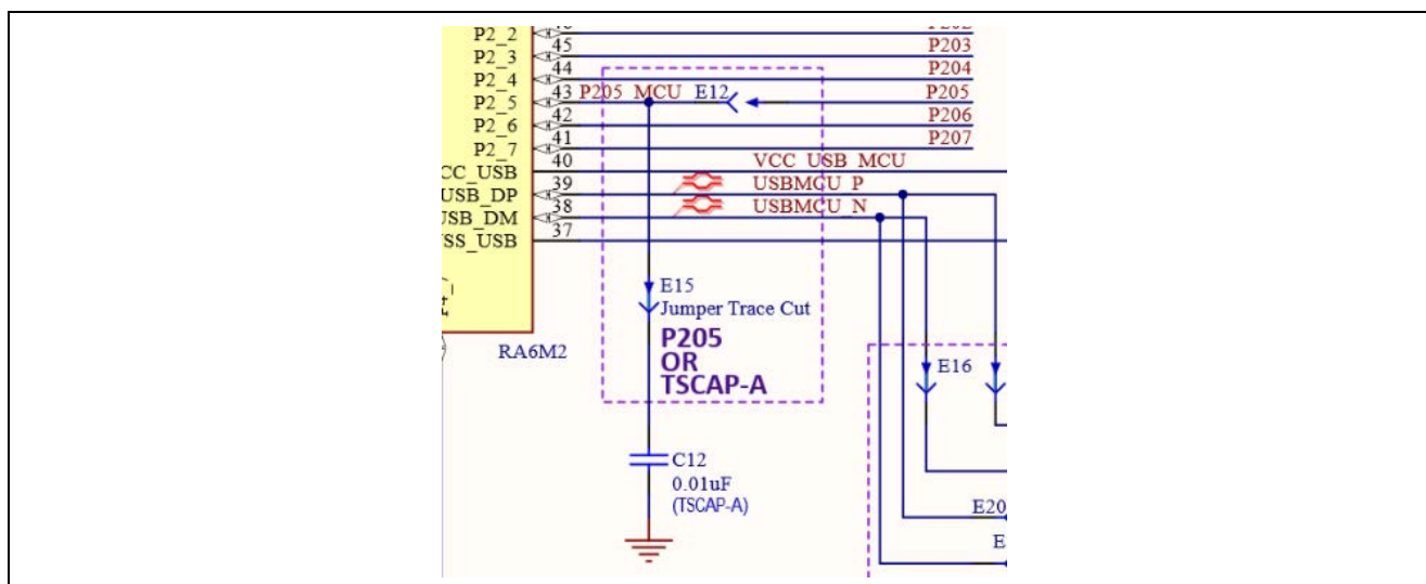
Figure 35. P205 Circuit
