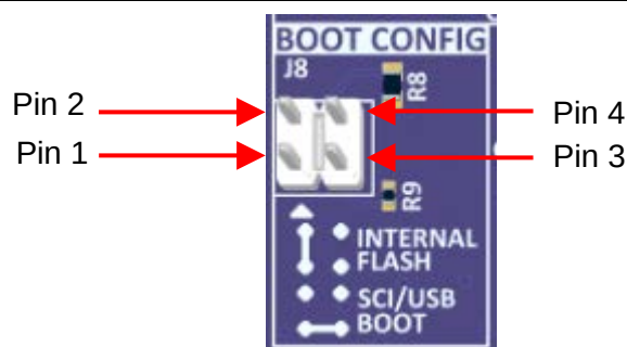
Figure 29. Boot Configuration Header
