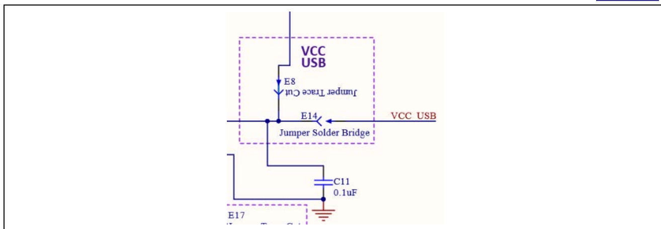
Figure 34. VCC_USB Circuit
