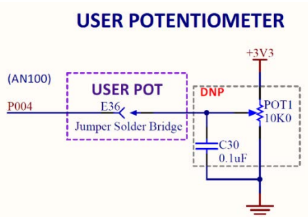
Figure 27. User Potentiometer Circuit
