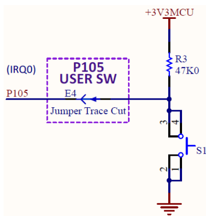
Figure 17. User Switch Circuit
