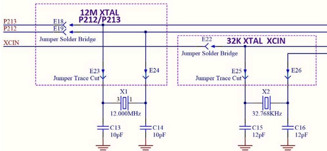
Figure 26. Crystal Clock Sources
