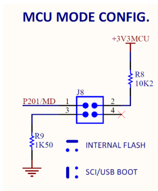
Figure 30. Boot Mode Configuration Circuit
