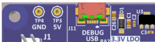
Figure 7. USB Debug Connector (J11), TP3, and TP4 on the Evaluation Kit Board
