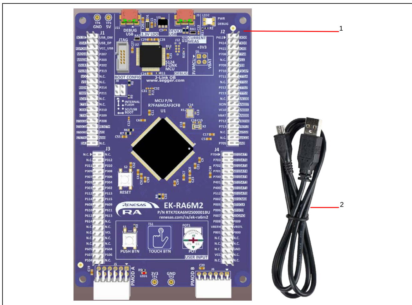
Figure 3. EK-RA6M2 v1 Kit Contents
