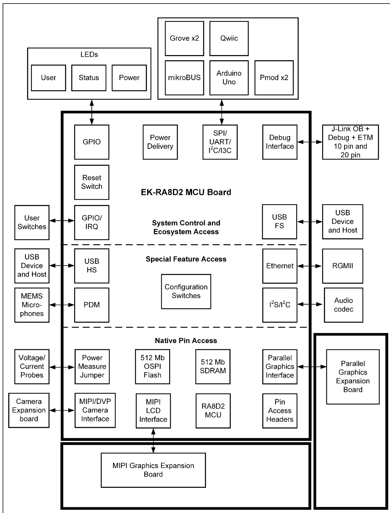
Figure 5. EK-RA8D2 Board Block Diagram
