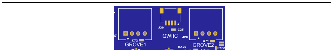
Figure 12. Seeed Grove ® and SparkFun ® Qwiic ® Connector Footprints
