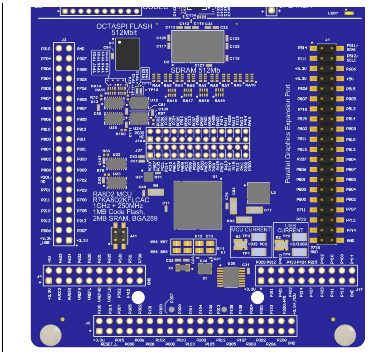
Figure 31. Native Pin Access Area
