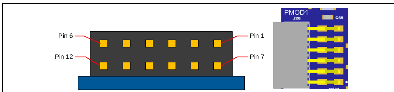
Figure 13. Pmod 1 Connector
