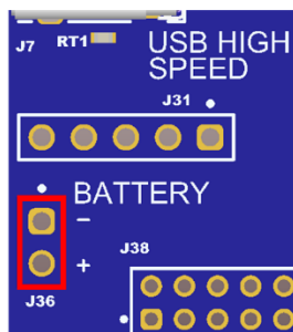
Figure 10. VBATT supply (J36) location
