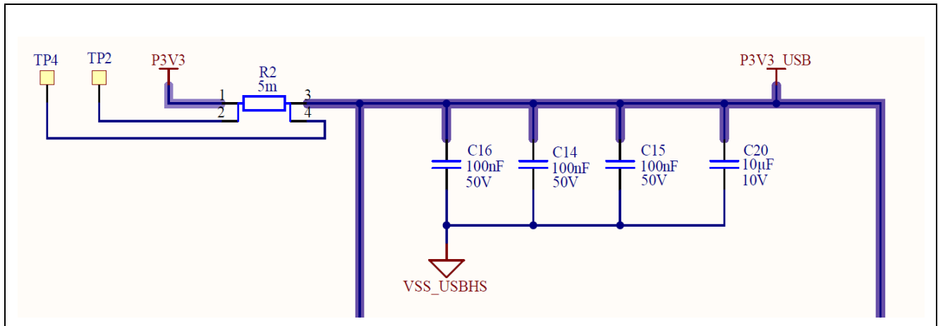
Figure 32. RA USB Current Measurement Circuit
