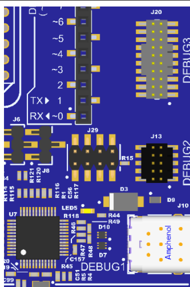
Figure 11. EK-RA8D2 Debug Interface
