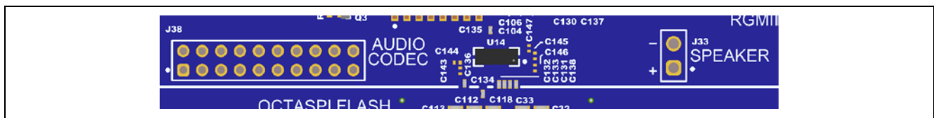
Figure 30. Audio CODEC (U14), Speaker Connector (J33) and Pin Header (J38)
