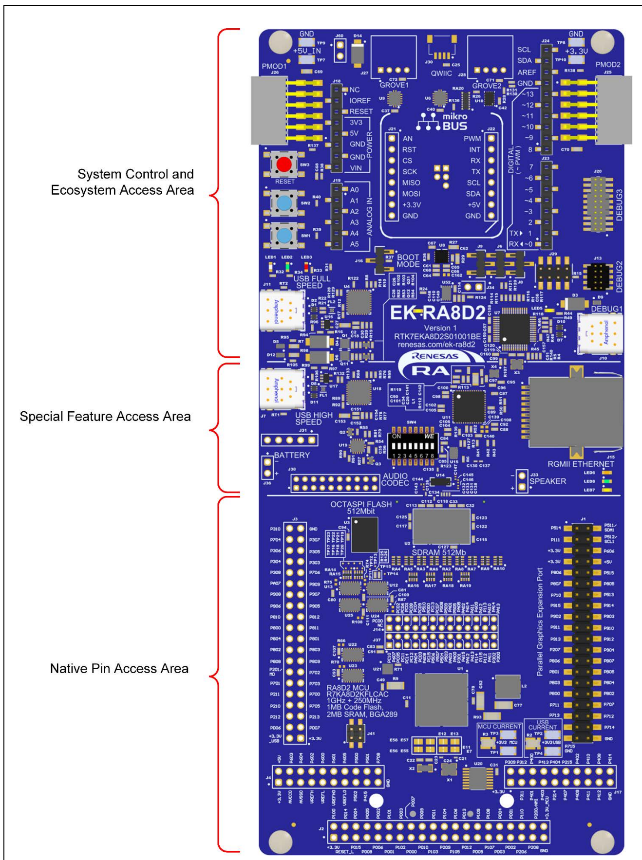
Figure 4. EK-RA8D2 Board Functional Area Definitions
