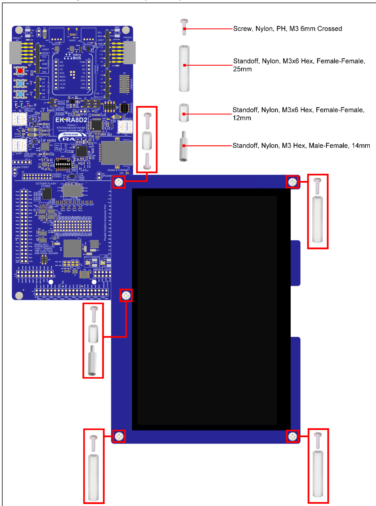
Figure 36. Parallel Graphics Expansion Board 1 connected to EK-RA8D2 Board
