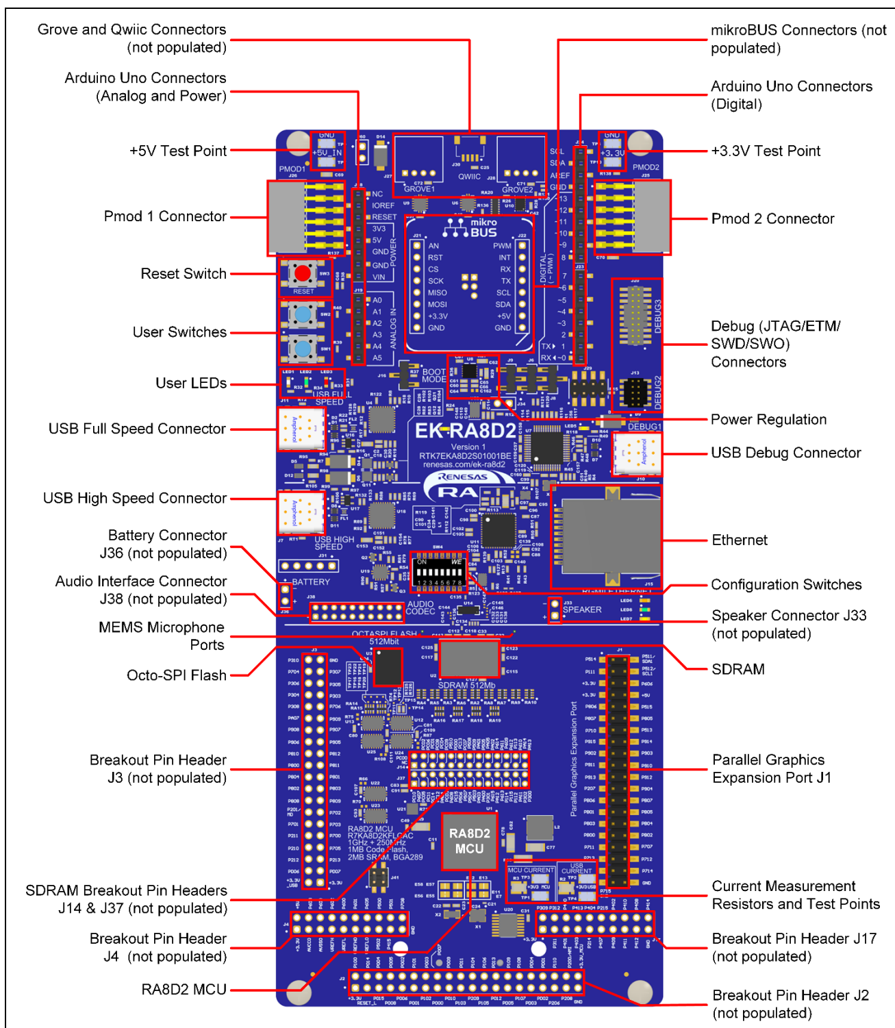
Figure 1. EK-RA8D2 Board Top Side
