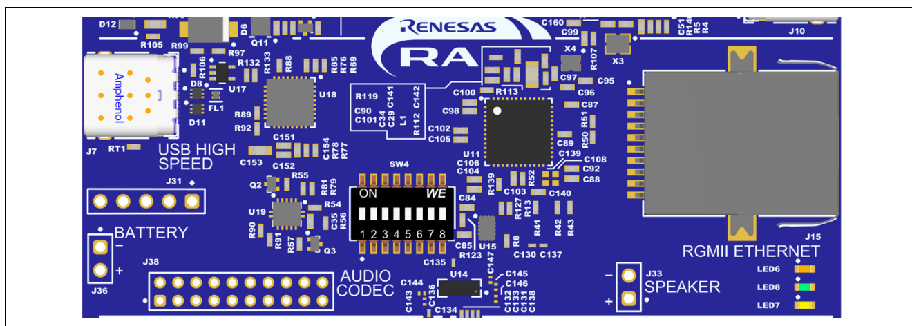
Figure 24. Special Feature Access Area
