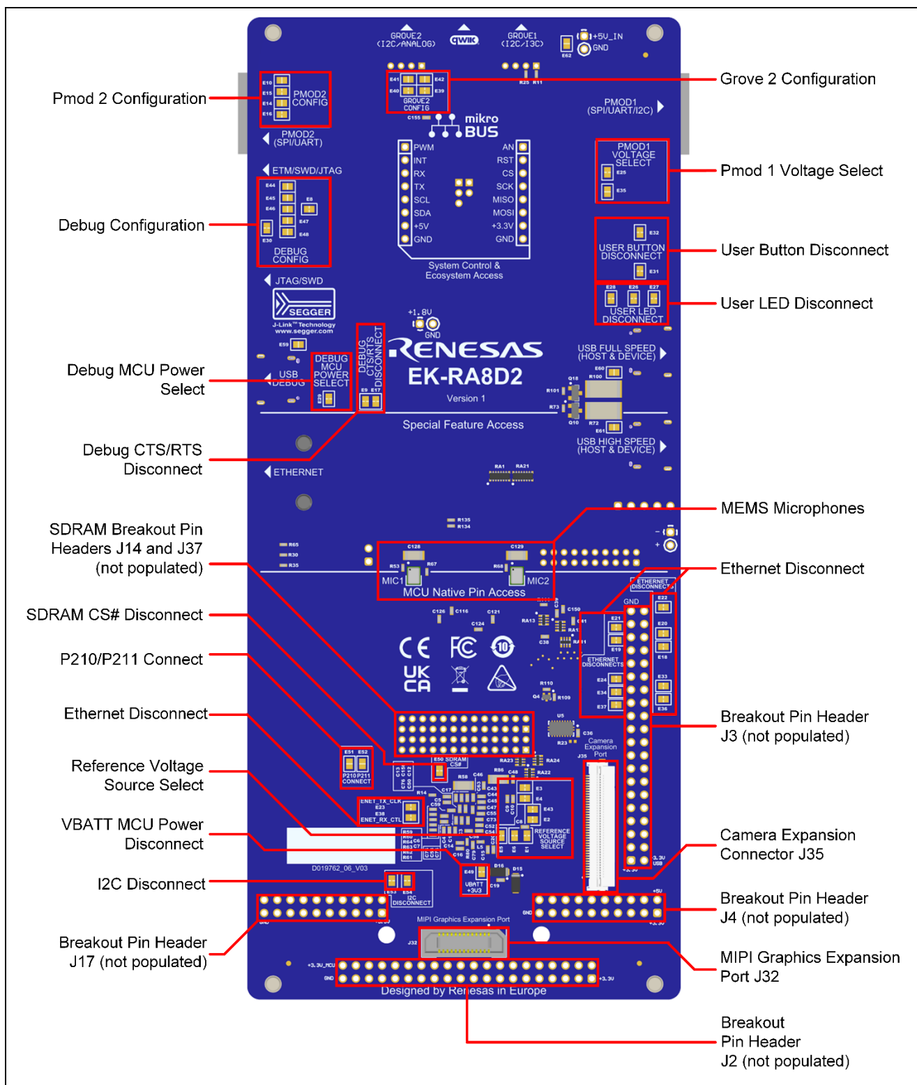
Figure 2. EK-RA8D2 Board Bottom Side
