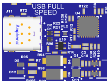
Figure 17. USB Full Speed Connector
