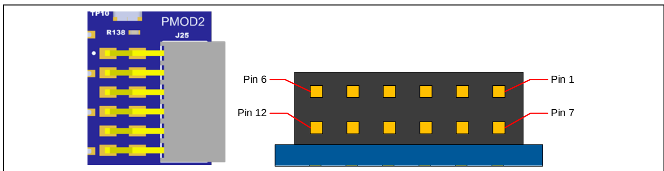
Figure 14. Pmod 2 Connector
