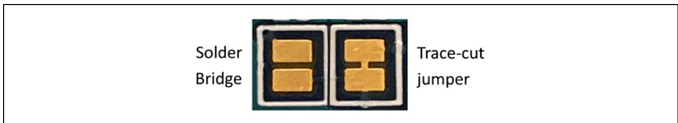
Figure 6. Copper Jumpers
