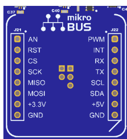
Figure 16. mikroBUS™ Connector
