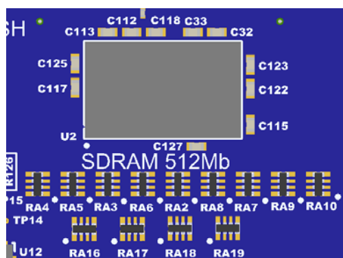
Figure 28. SDRAM
