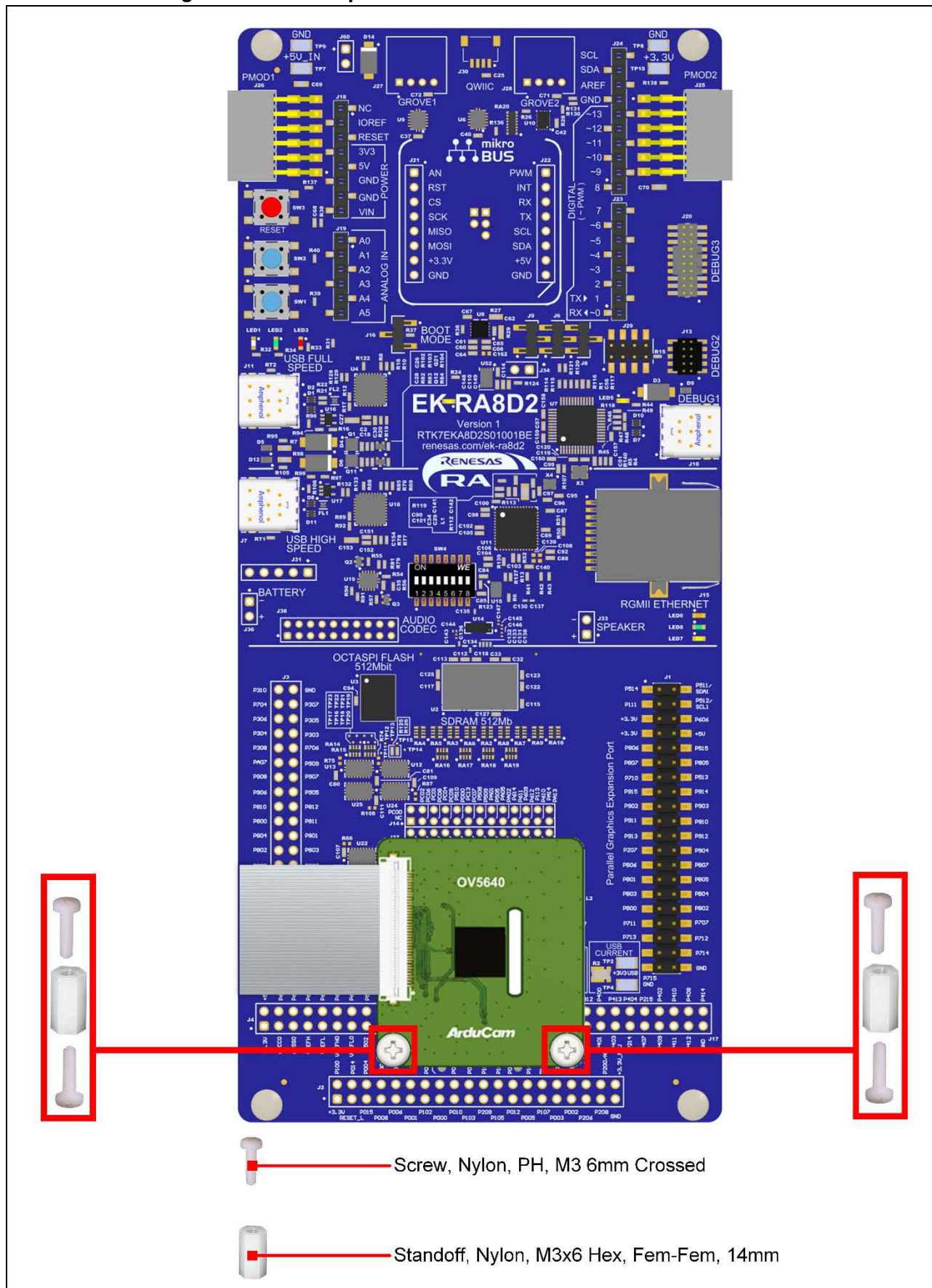
Figure 40. Camera Expansion Board connected to the EK-RA8D2
