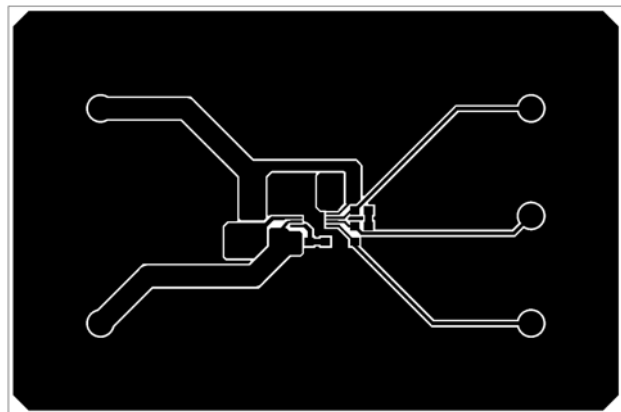
FIGURE 3. TOP LAYER
