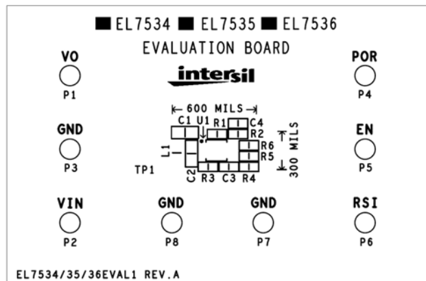
FIGURE 2. SILKSCREEN
