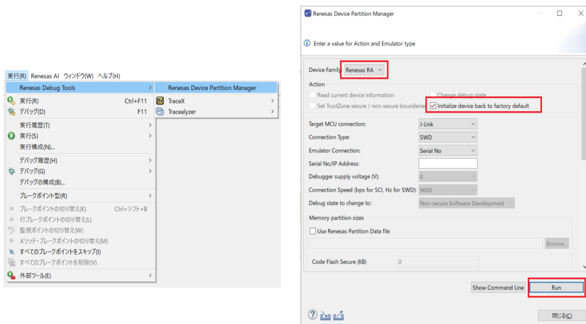
図 3-1 RA TrustZone® Secure用のRenesas Device Partition Manager設定
