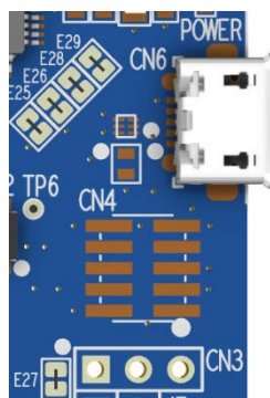
Figure 7. FPB-RA2E1 Debug Interface
