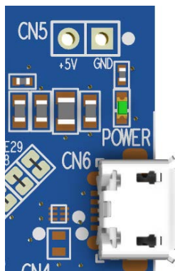
Figure 14. Power LED
