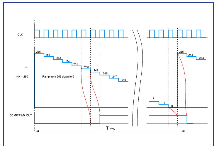
DCMP/PWM in PWM mode
