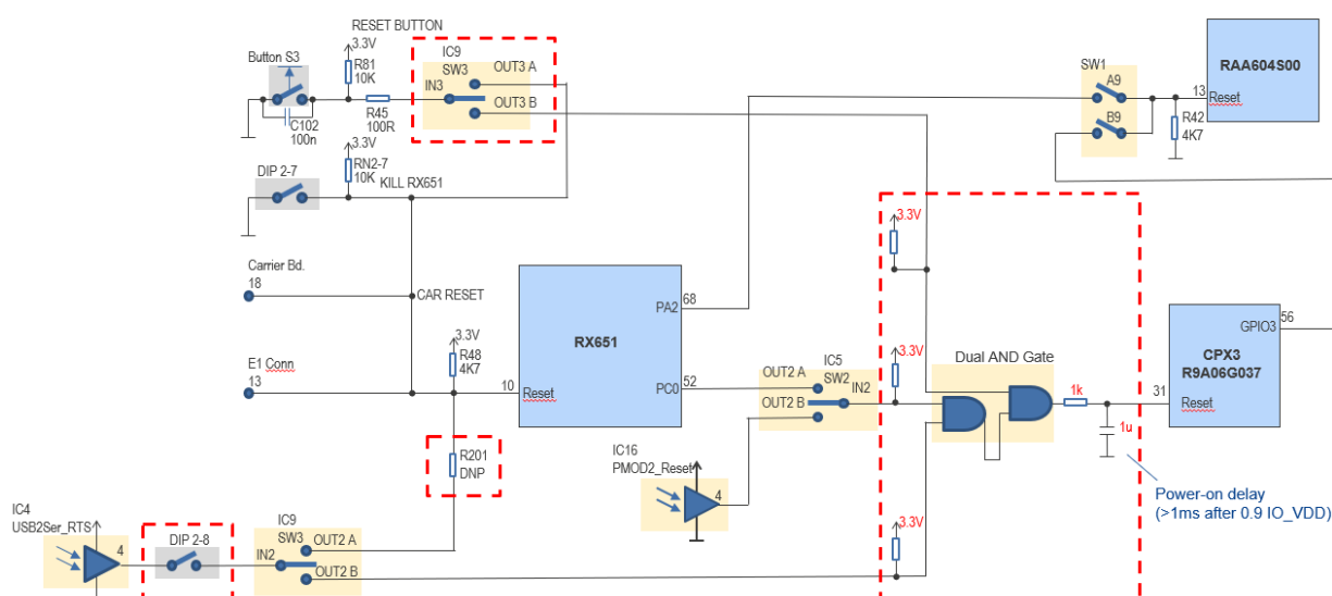
Figure 10. Reset Circuitry
