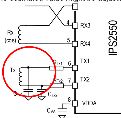
Figure 18. Transmitter current configuration for LC Tank
