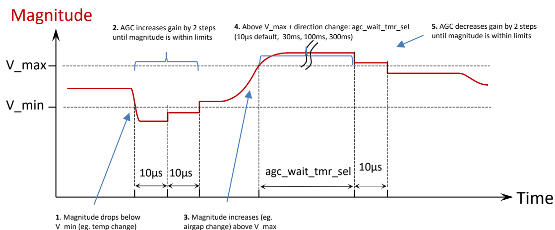
Figure 6. AGC Effect on Change in Magnitude
