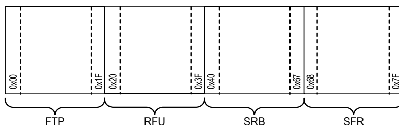
Figure 15. Memory Architecture
