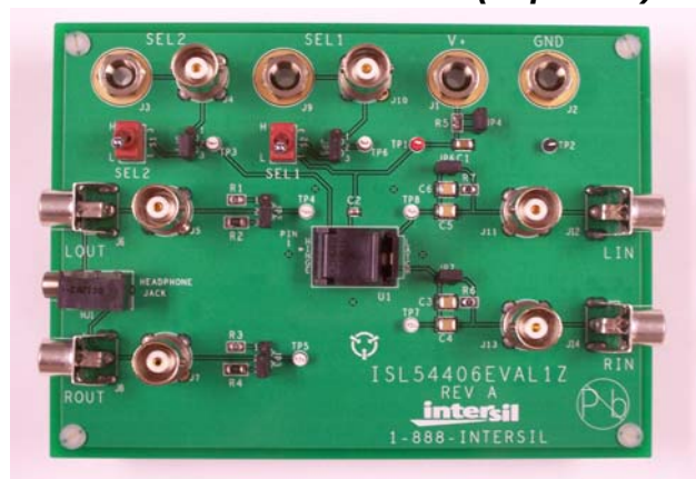
FIGURE 1. ISL54406EVAL1Z EVALUATION BOARD
