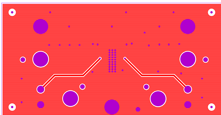
Figure 7. Bottom Layer
