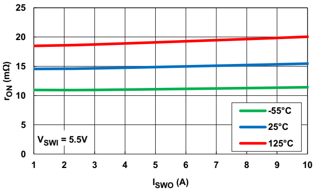
Figure 10. r_{ON} vs I_{SWO} vs Temperature
