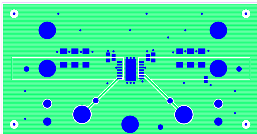
Figure 6. Top Layer
