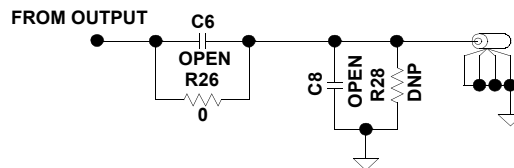
FIGURE 4. OUTPUT STAGE (1/2)
