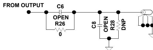
FIGURE 4. OUTPUT STAGE (1/2)
