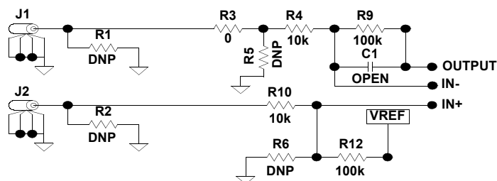
FIGURE 3. INPUT STAGE (1/2)
