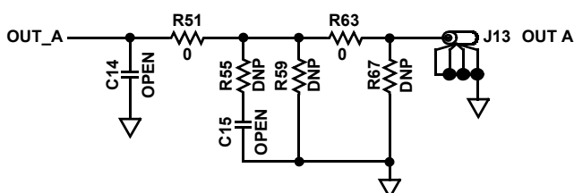
FIGURE 4. OUTPUT STAGE
