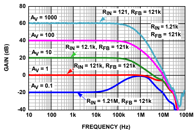
FIGURE 9. CLOSED LOOP GAIN ( R_{FB} = 121k ) vs FREQUENCY
