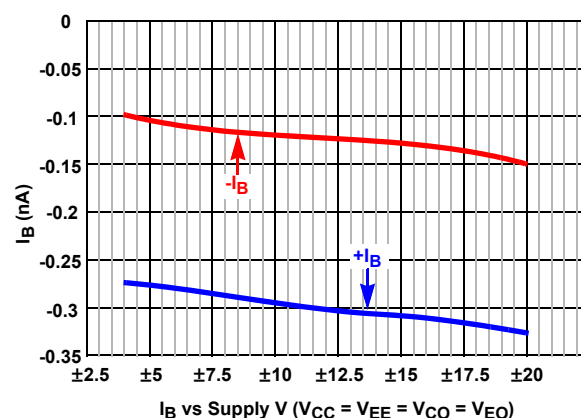
FIGURE 3. I_B vs SUPPLY VOLTAGE ( V_{CC} - V_{EE} )
