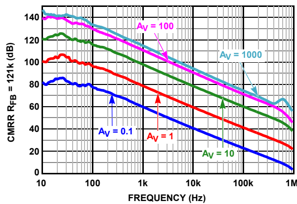
FIGURE 7. CMRR (RTI) R_F = 121k
