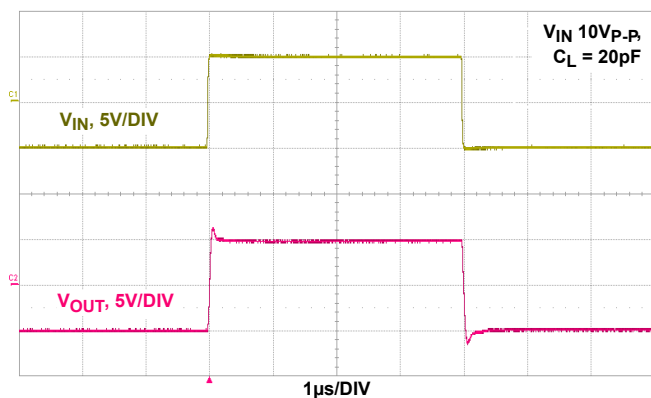
FIGURE 12. LARGE SIGNAL STEP RESPONSE ( \pm 18V )
