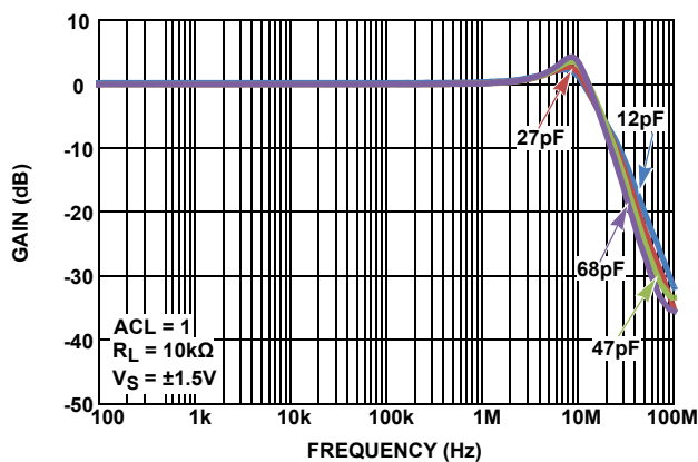
FIGURE 17. ( V_S = \pm 1.5V ) UNITY GAIN RESPONSE vs CL
