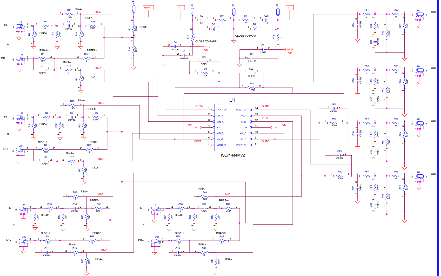
FIGURE 7. ISL71444MEVAL1Z SCHEMATIC
