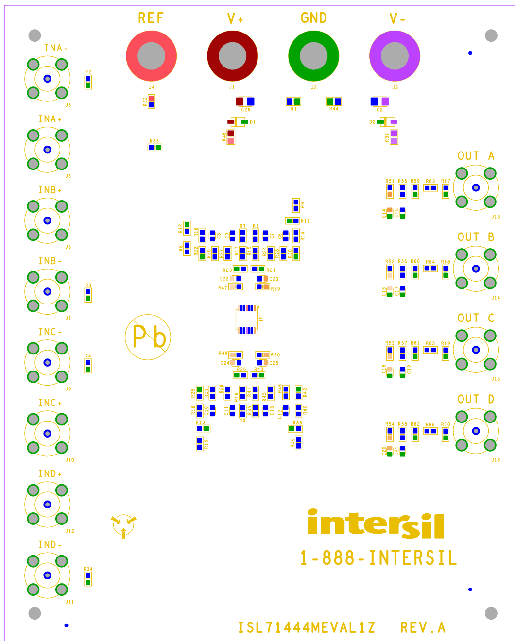
FIGURE 8. TOP VIEW
