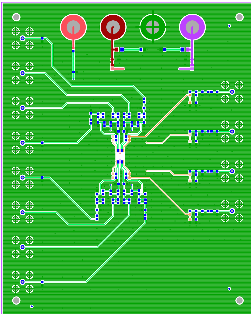
FIGURE 9. TOP LAYER
