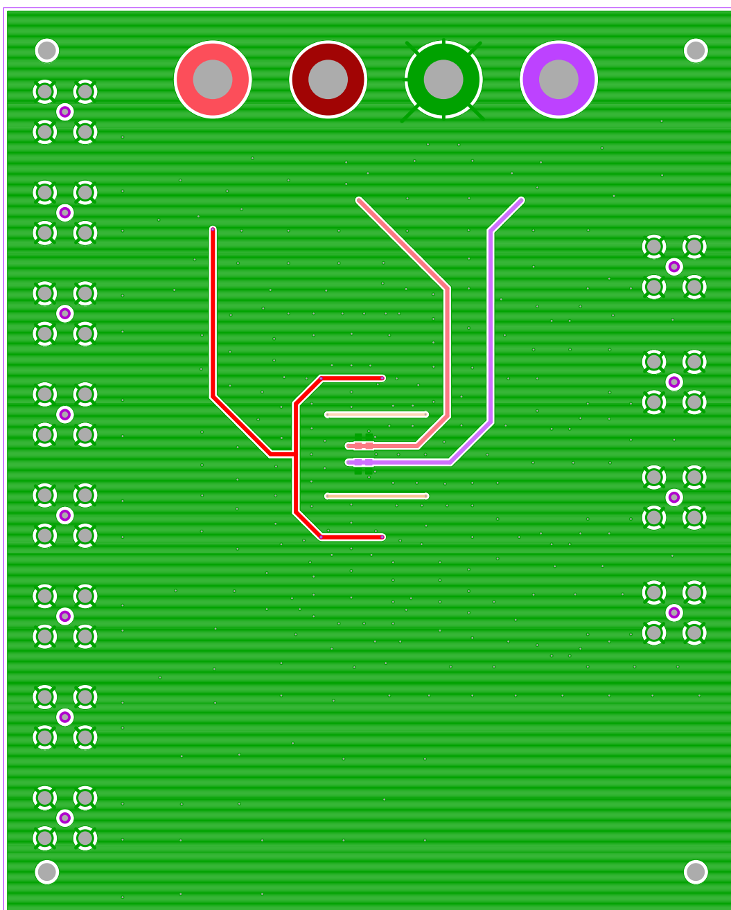
FIGURE 10. BOTTOM LAYER
