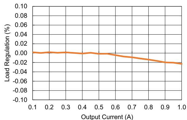
Figure 13. Load Regulation vs Output Current
