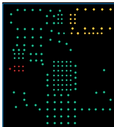
Figure 7. Layer 2
