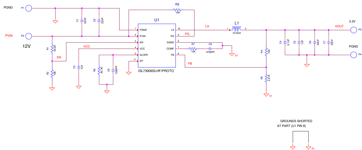
Figure 5. Schematic
