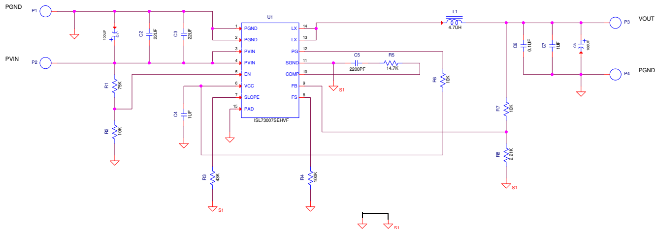
Figure 5. Schematic
