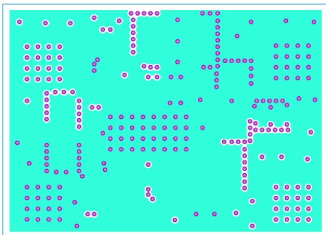
Figure 8. Layer 3
