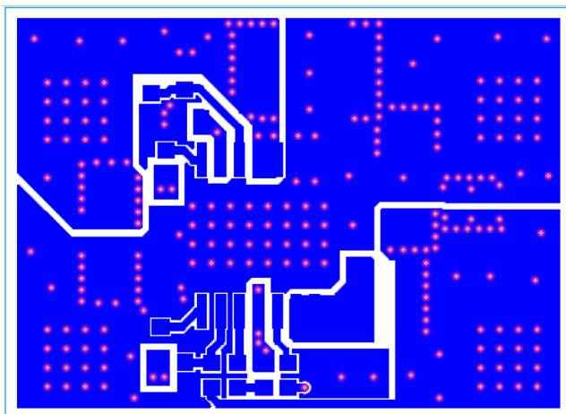
Figure 6. Top Layer
