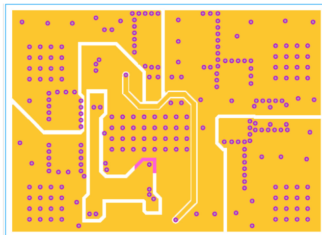
Figure 9. Bottom Layer
