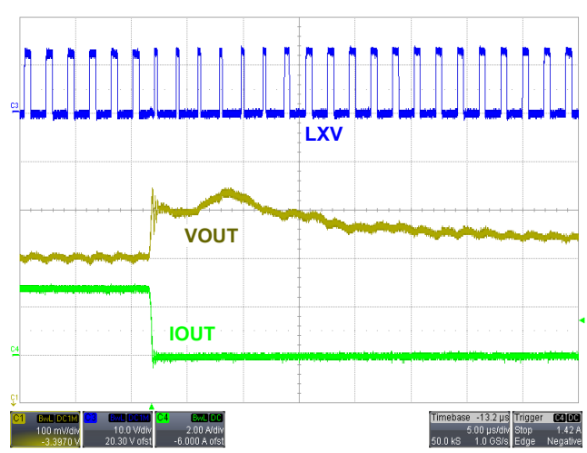
Figure 17. -2.8A Output Current Transient
