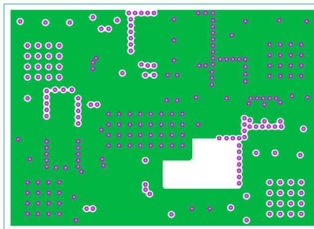
Figure 7. Layer 2
