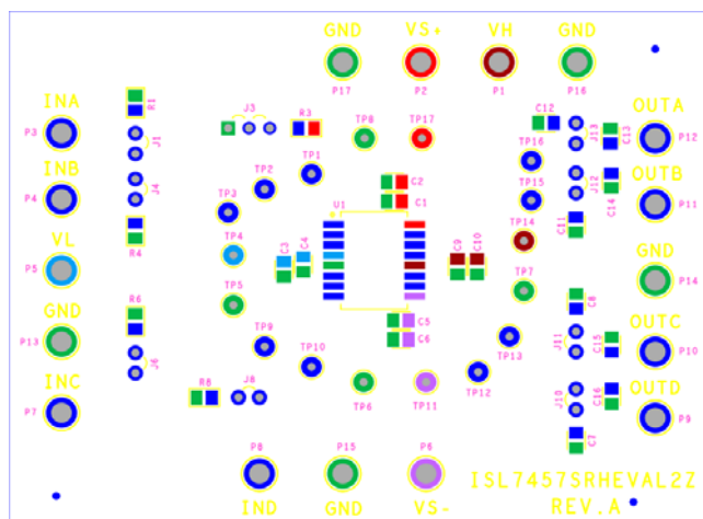
Figure 5. Top Silkscreen
