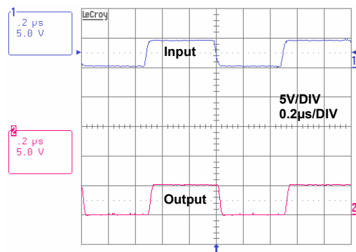
Figure 9. V_H = V_{S+} = 5V , 1MHz
