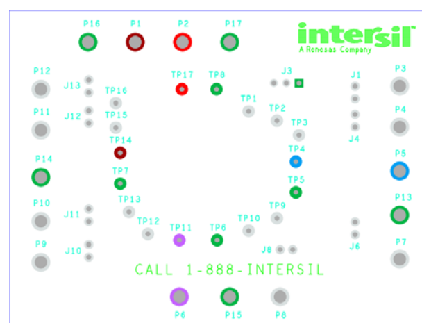
Figure 6. Top Layer
