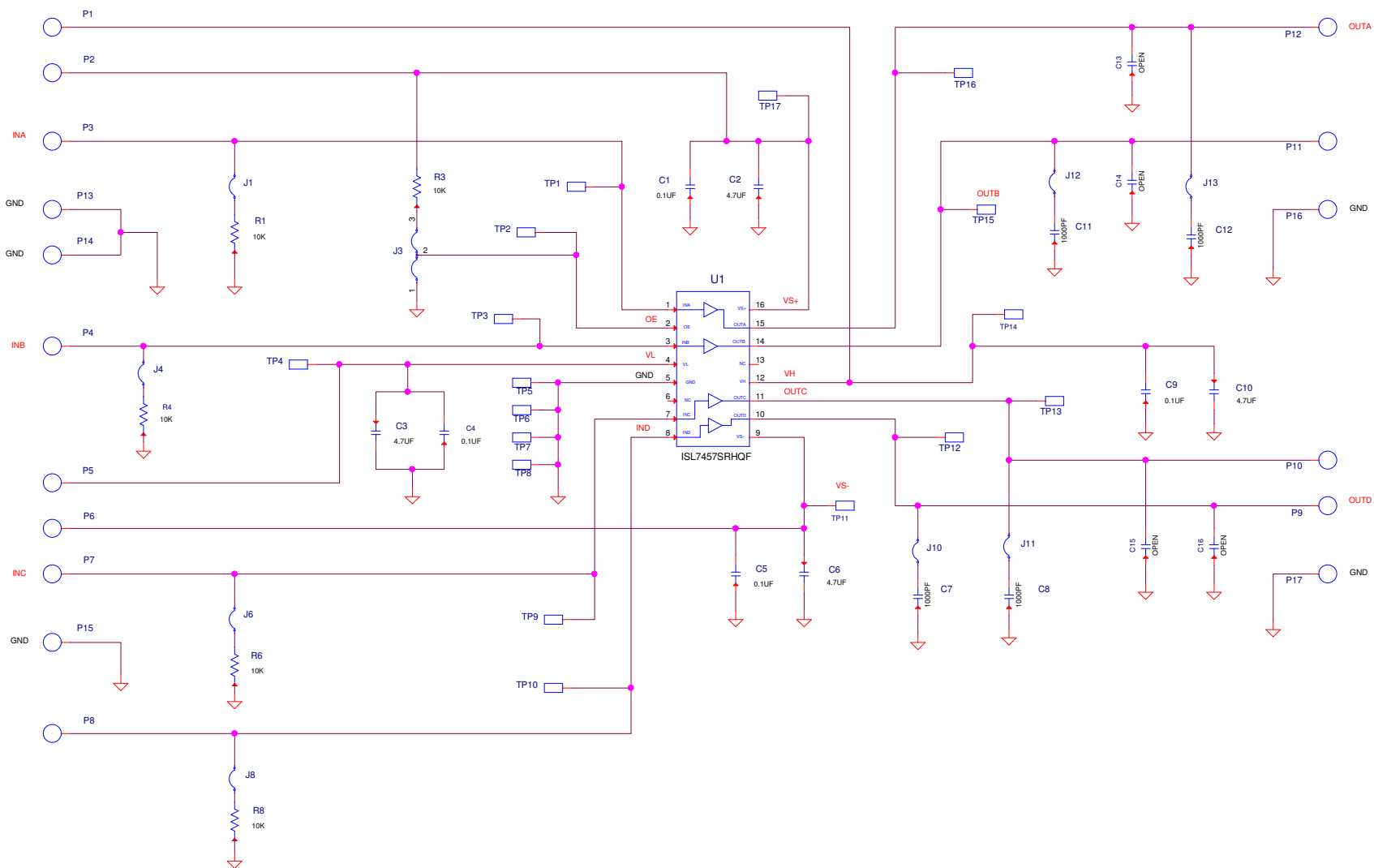
Figure 4. ISL7457SRHEVAL2Z Schematic
