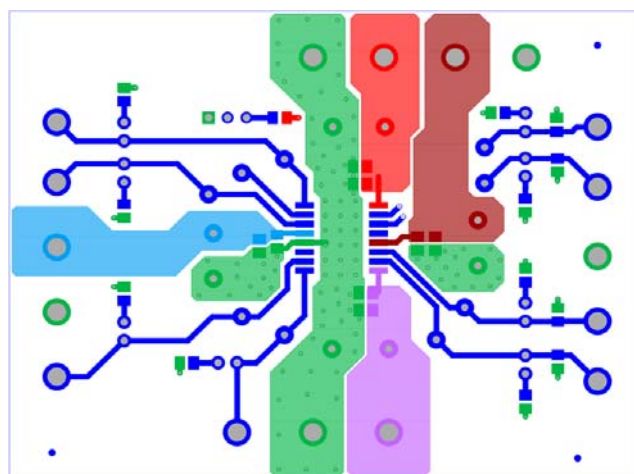
Figure 6. Top Layer
