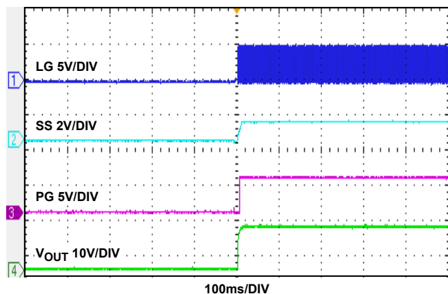
FIGURE 19. START-UP WAVEFORMS, I_0 = 3A
