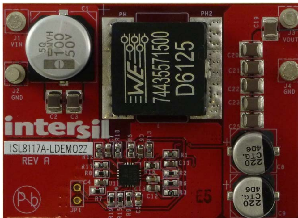
FIGURE 4. TOP VIEW
