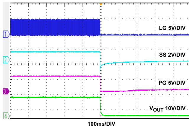
FIGURE 20. SHUT-DOWN WAVEFORMS, I_0 = 3A
