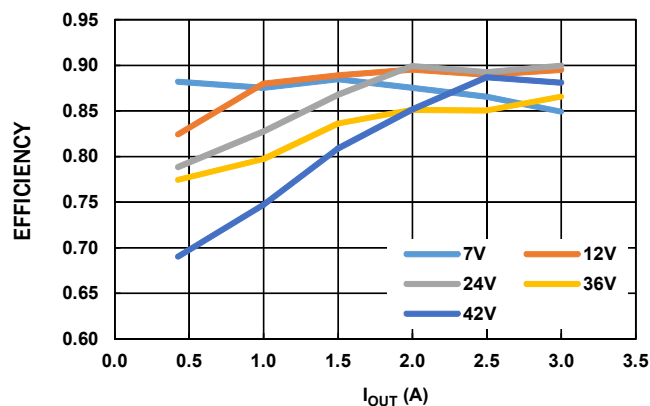
FIGURE 13. EFFICIENCY
