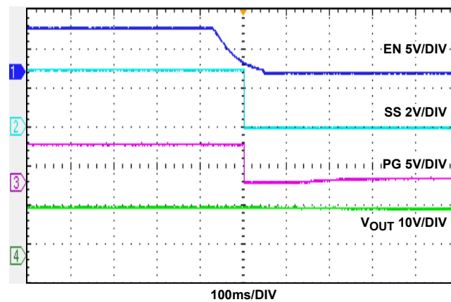
FIGURE 18. SHUT-DOWN WAVEFORMS, I_0 = 0A
