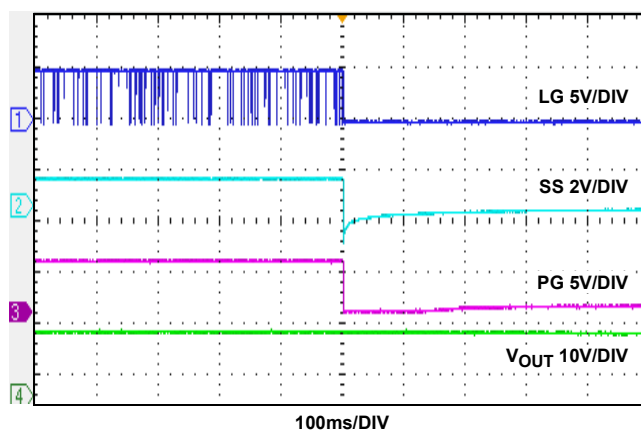
FIGURE 16. SHUT-DOWN WAVEFORMS, I_0 = 0A
