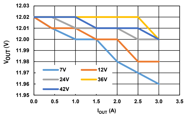
FIGURE 14. LOAD REGULATION
