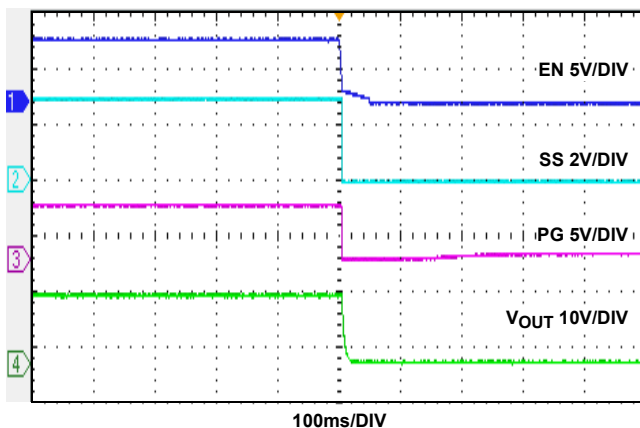
FIGURE 22. SHUT-DOWN WAVEFORMS, I_0 = 3A
