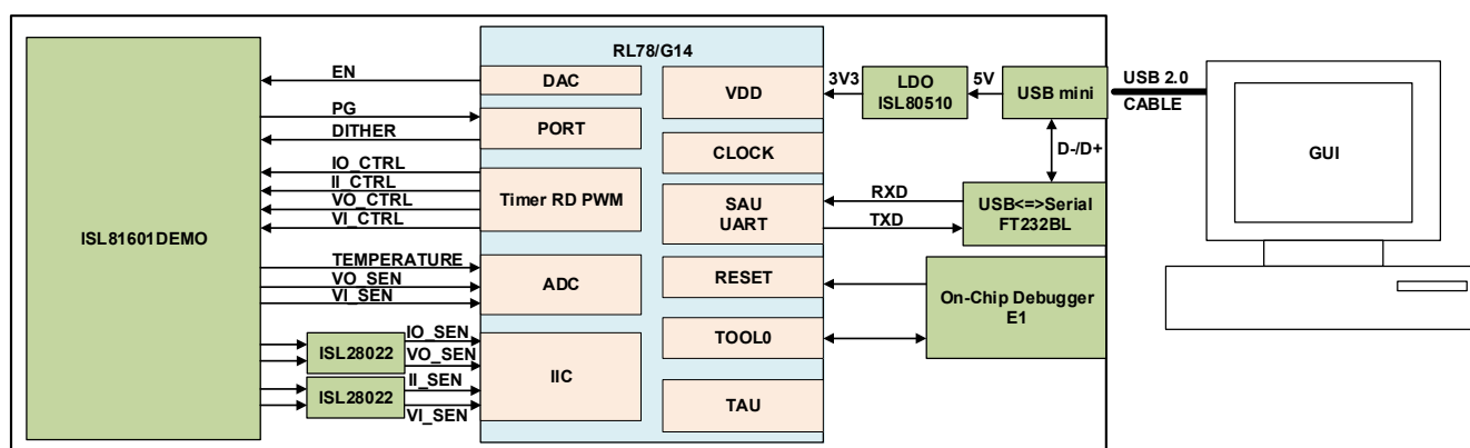
Figure 1. Block Diagram
