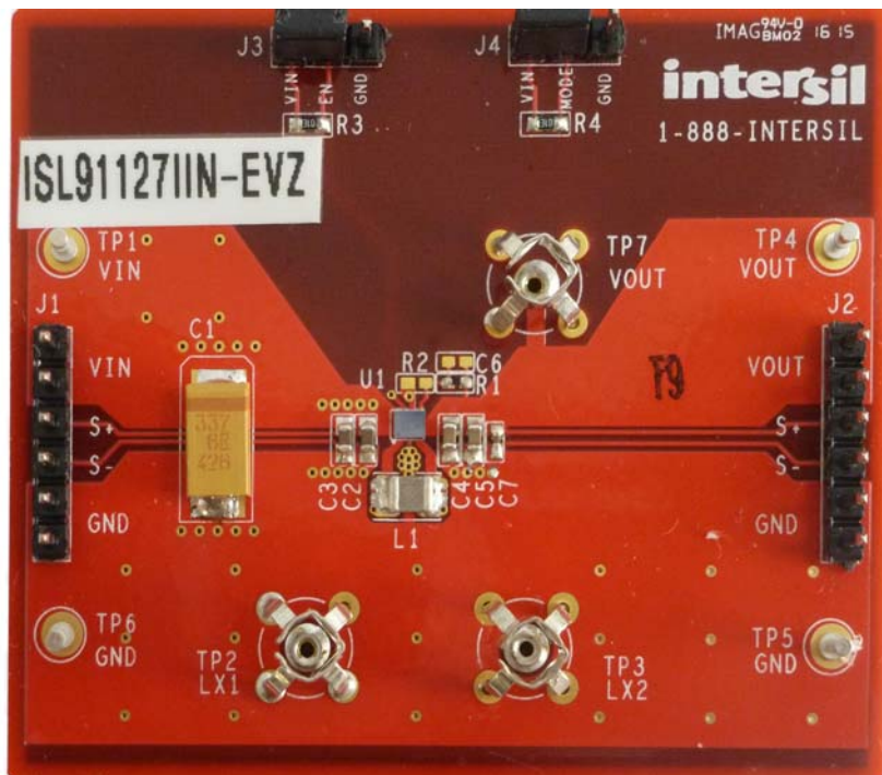
FIGURE 5. ISL91127IIN-EVZ BOARD
