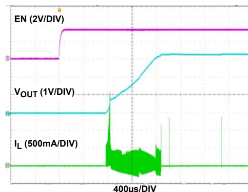
FIGURE 2. START-UP WITH V_{IN} = 3.6\text{V} and V_{OUT} = 3.3\text{V} , NO LOAD
