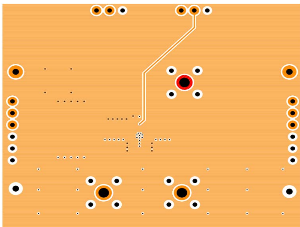
FIGURE 10. INNER LAYER 2
