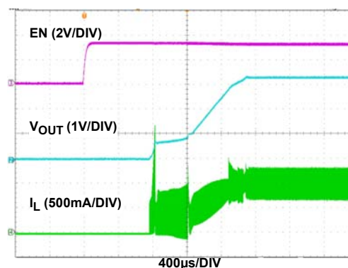
FIGURE 3. START-UP WITH V_{IN} = 3.6\text{V} , V_{OUT} = 3.3\text{V} , 1A R_{LOAD}
