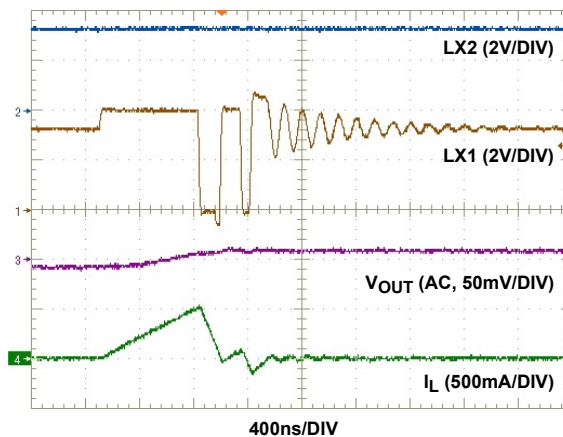
FIGURE 13. STEADY-STATE OPERATION IN PFM ( V_{IN} = 4V , V_{OUT} = 3.3V , NO LOAD)
