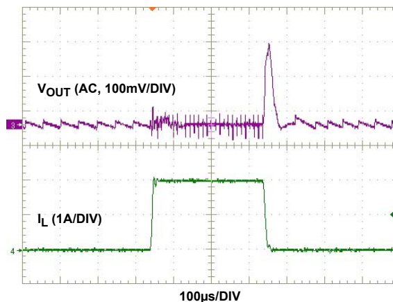
FIGURE 15. 0A TO 2A LOAD TRANSIENT ( V_{IN} = 3.6V , V_{OUT} = 3.3V )
