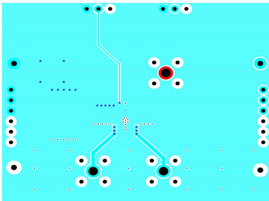
FIGURE 9. INNER LAYER 1
