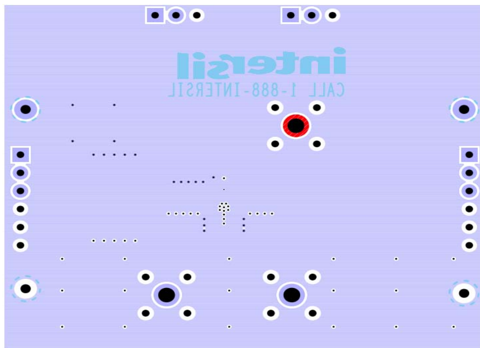
FIGURE 11. BOTTOM LAYER
