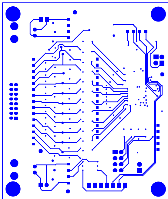
Figure 20. Middle Layer 2
