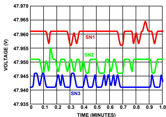
Figure 29. V_{BAT} Device to Device 48V
