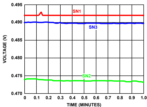
Figure 25. ETV1 Device to Device Spread 48V
