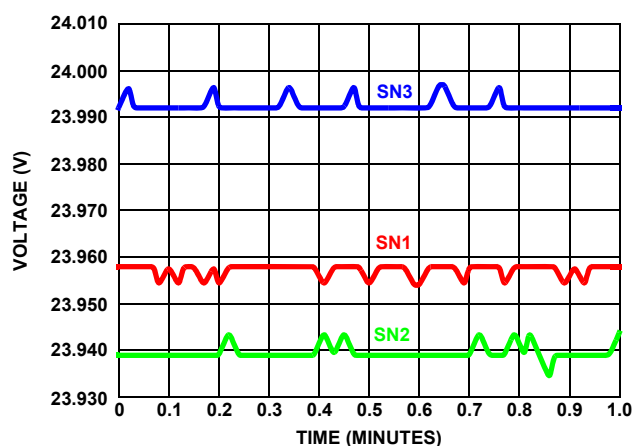
Figure 28. V_{BAT} Device to Device 24V
