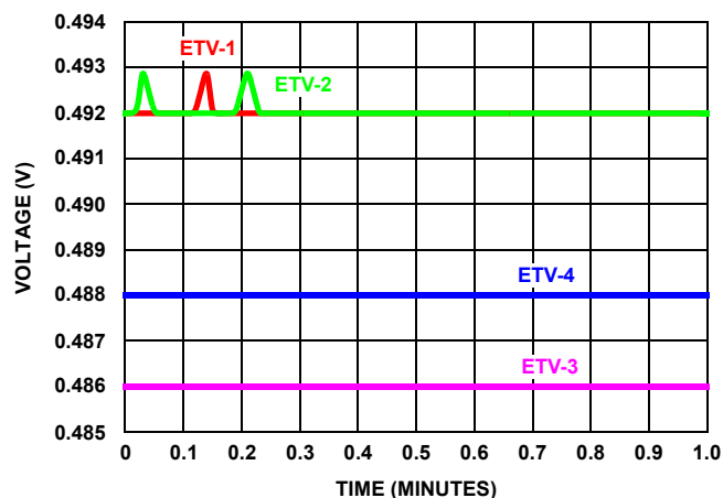
Figure 24. ETV1-4 Device 1 48V
