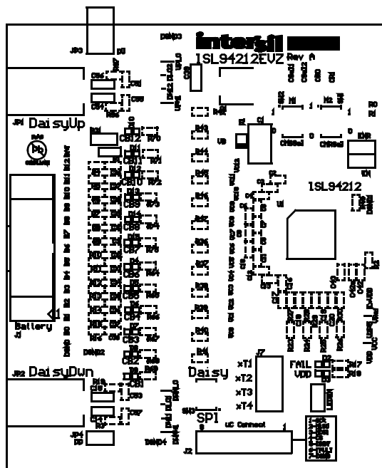
Figure 22. Silk Top Layer
