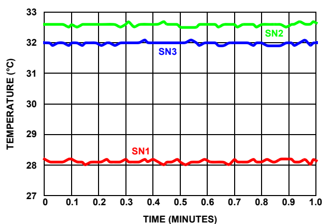
Figure 27. Internal Temperature Device to Device Spread 48V
