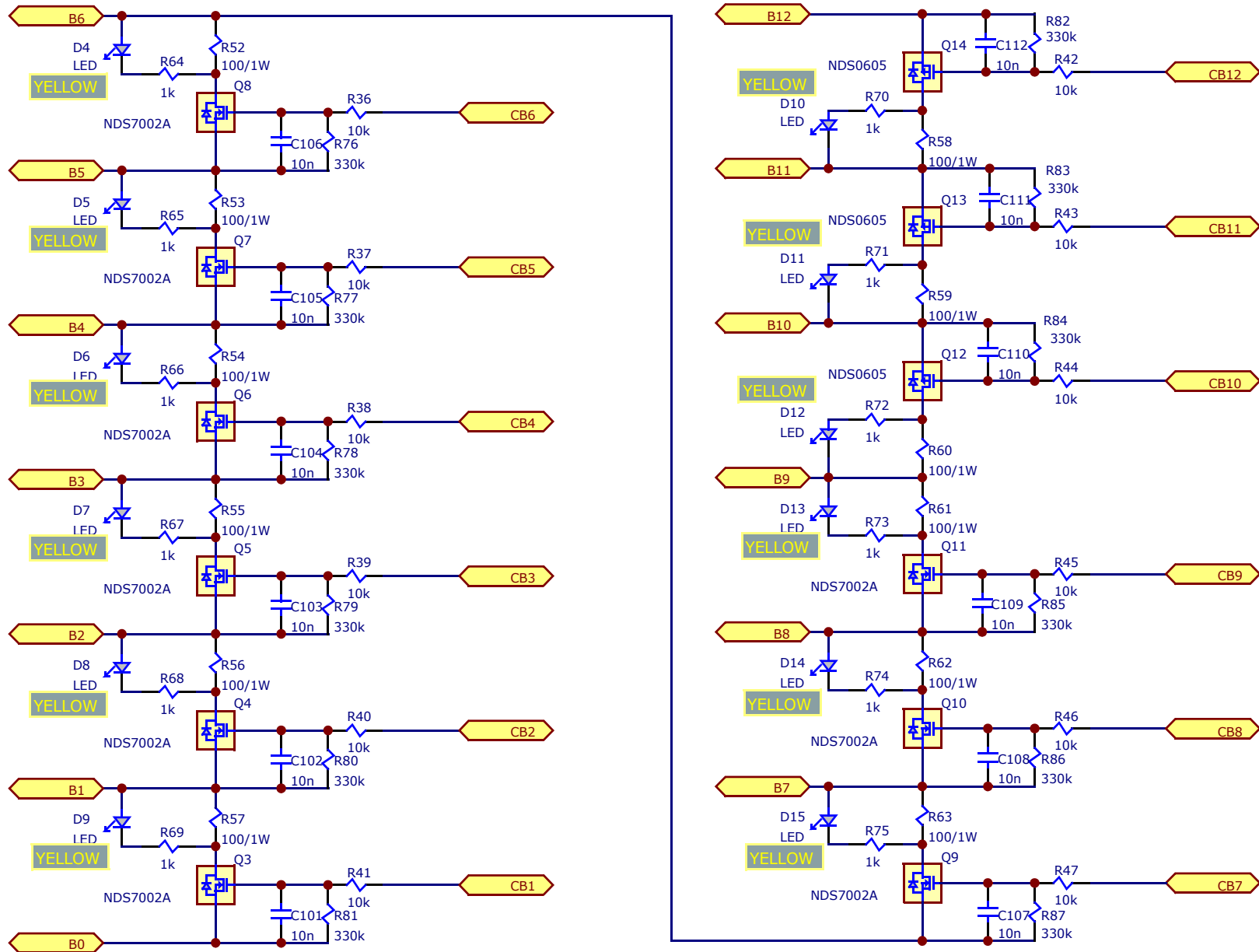
Figure 16. Schematic - Page 2
