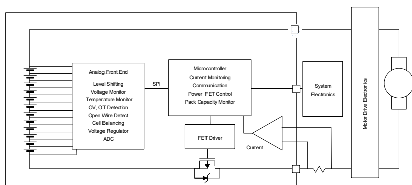
Figure 1. Single Device Configuration
