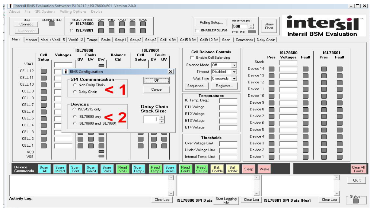
Figure 6. ISL94212EVZ Configuration Screen
