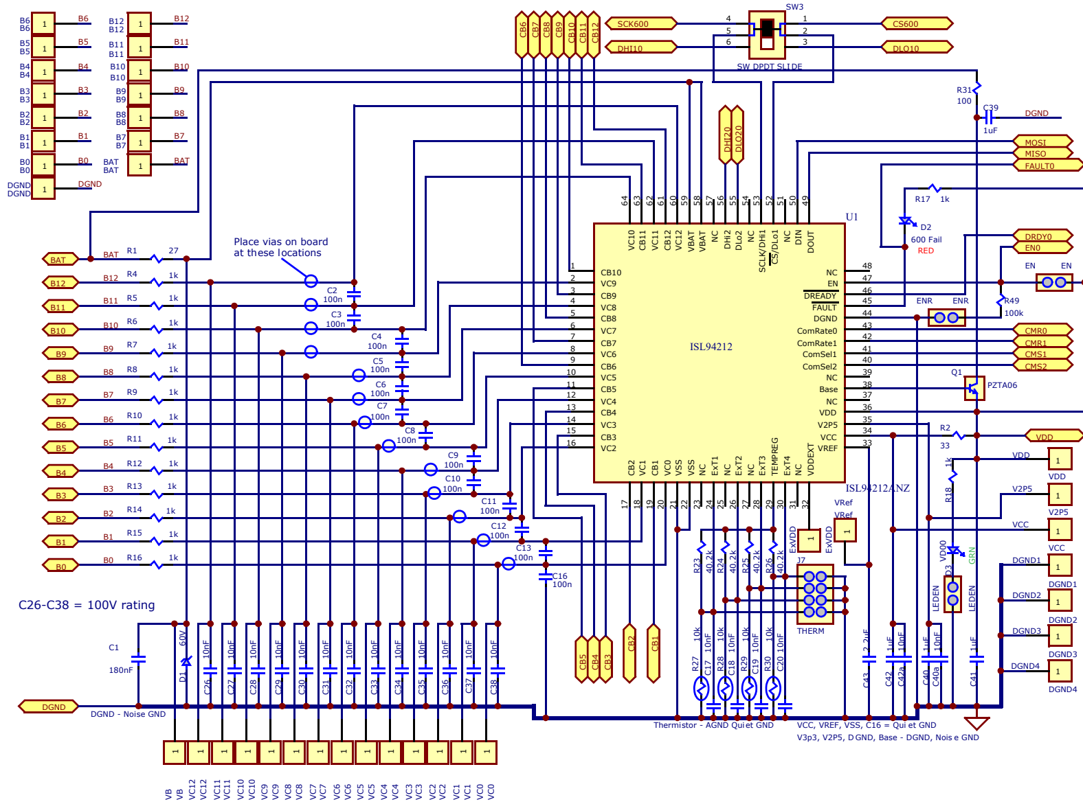
Figure 15. Schematic - Page 1
