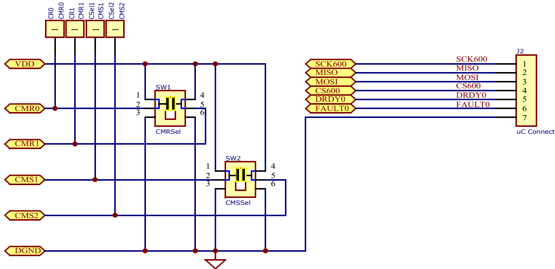
Figure 17. Schematic - Page 3
