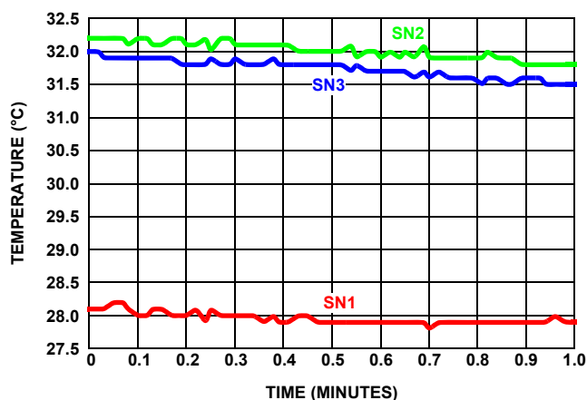
Figure 26. Internal Temperature Device to Device Spread 24V
