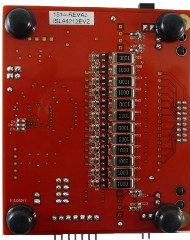
Figure 14. Bottom Side
