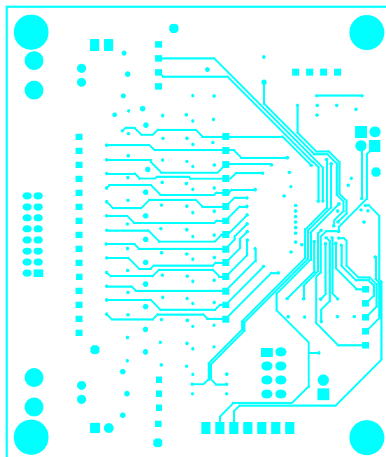
Figure 19. Middle Layer 1
