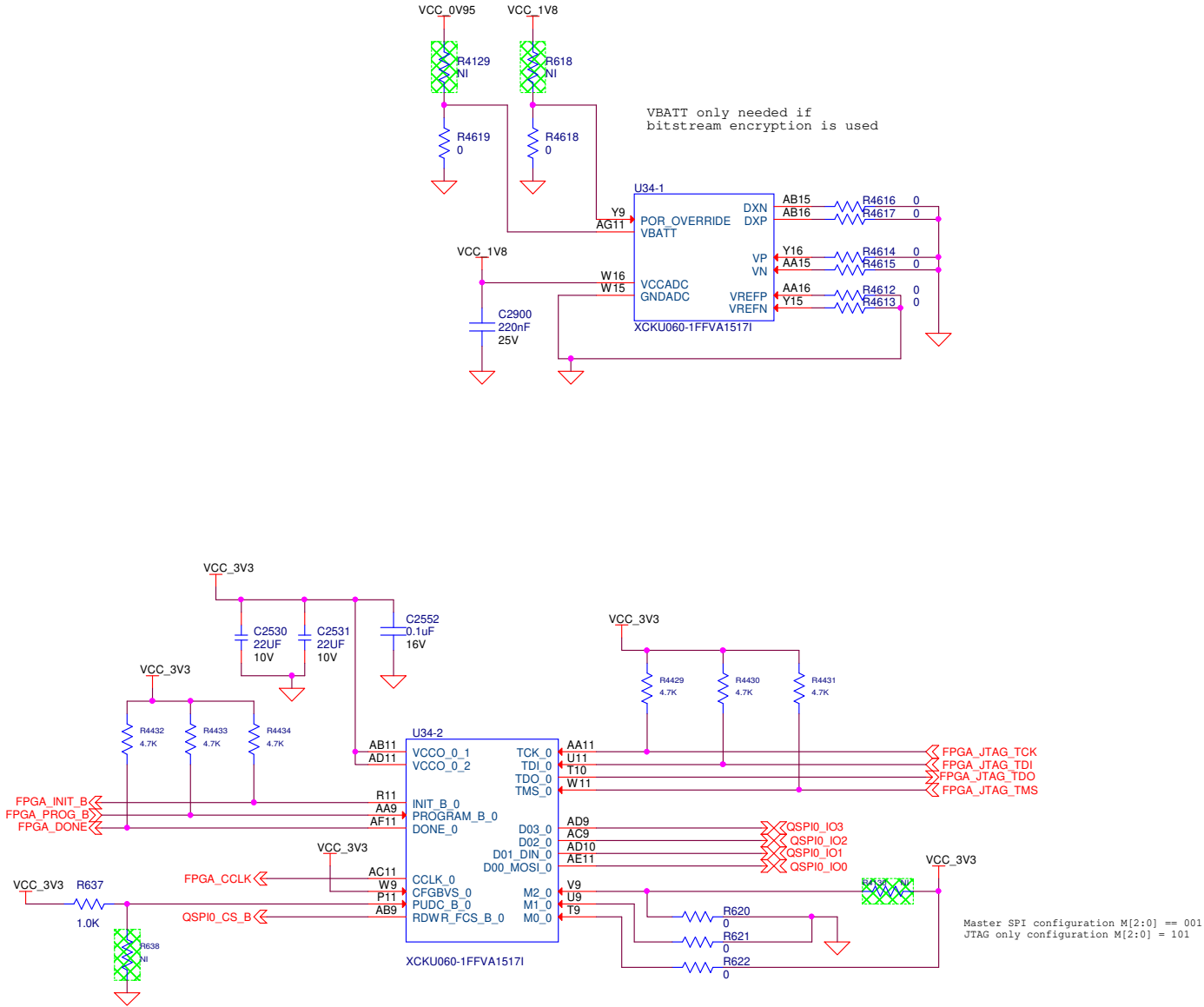
Figure 26. Schematic Page 11
