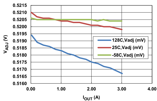
Figure 13. ISL75051ASEH Load Regulation, V_{ADJ} vs I_{OUT}
