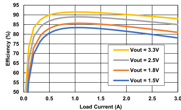
Figure 11. ISL70005SEH Buck Efficiency, V_{IN} = 5V , 1MHz
