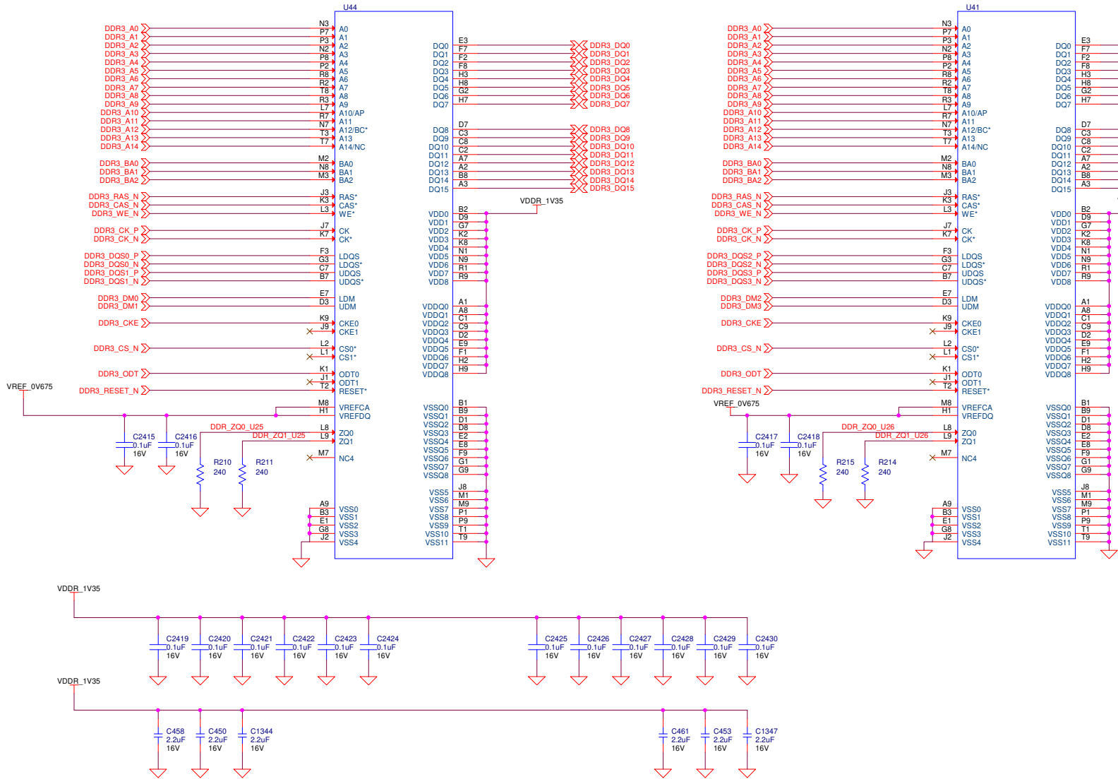
Figure 33. Schematic Page 18
