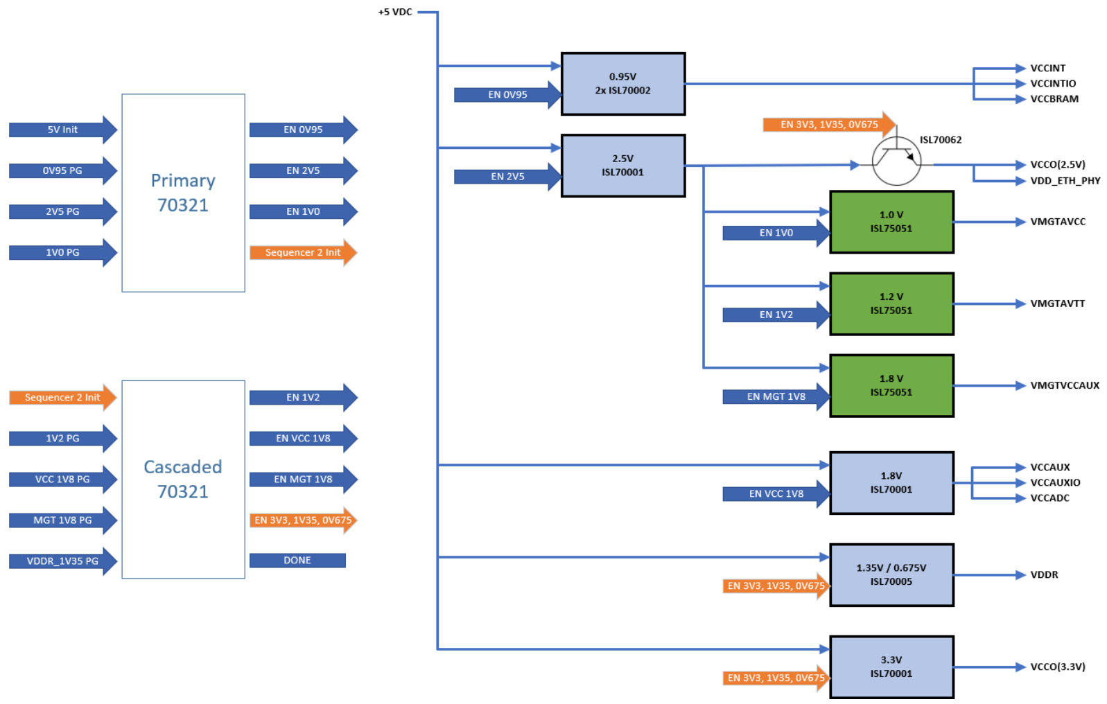
Figure 16. Schematic Page 1
