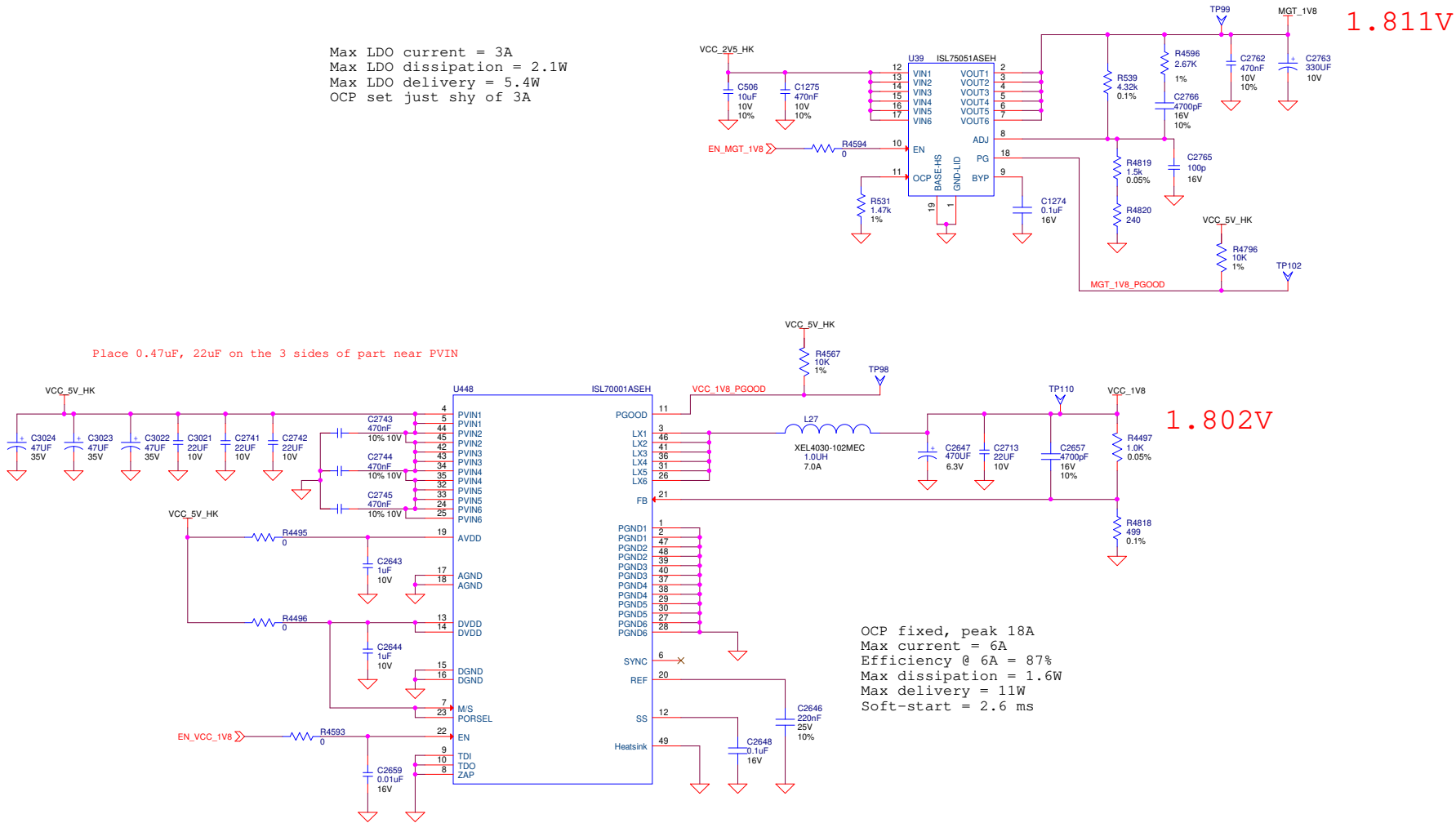
Figure 21. Schematic Page 6
