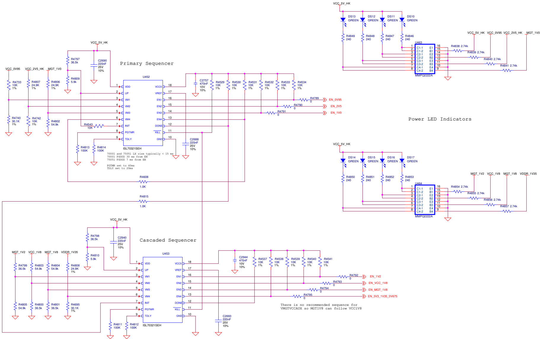
Figure 17. Schematic Page 2
