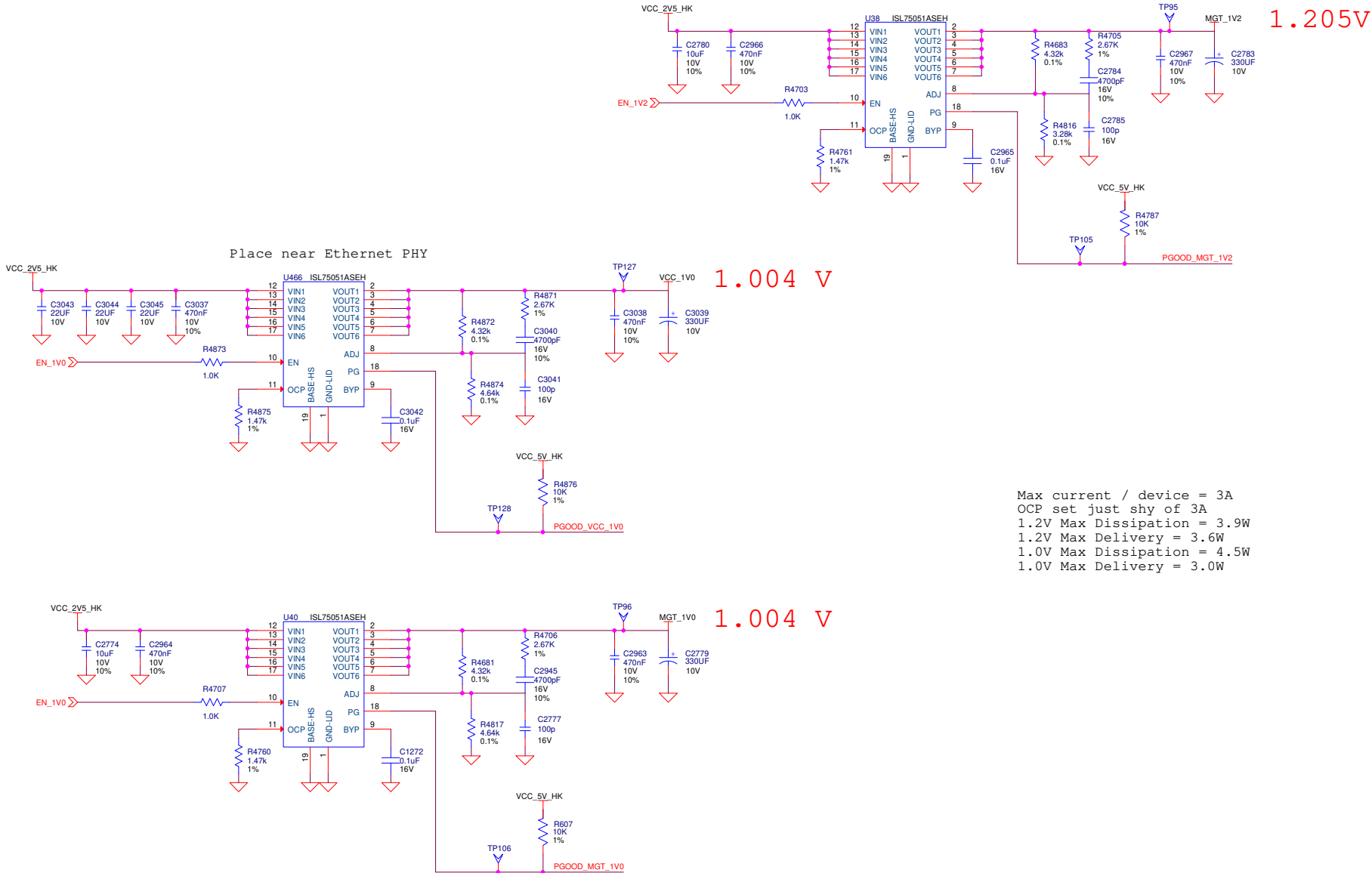
Figure 19. Schematic Page 4
