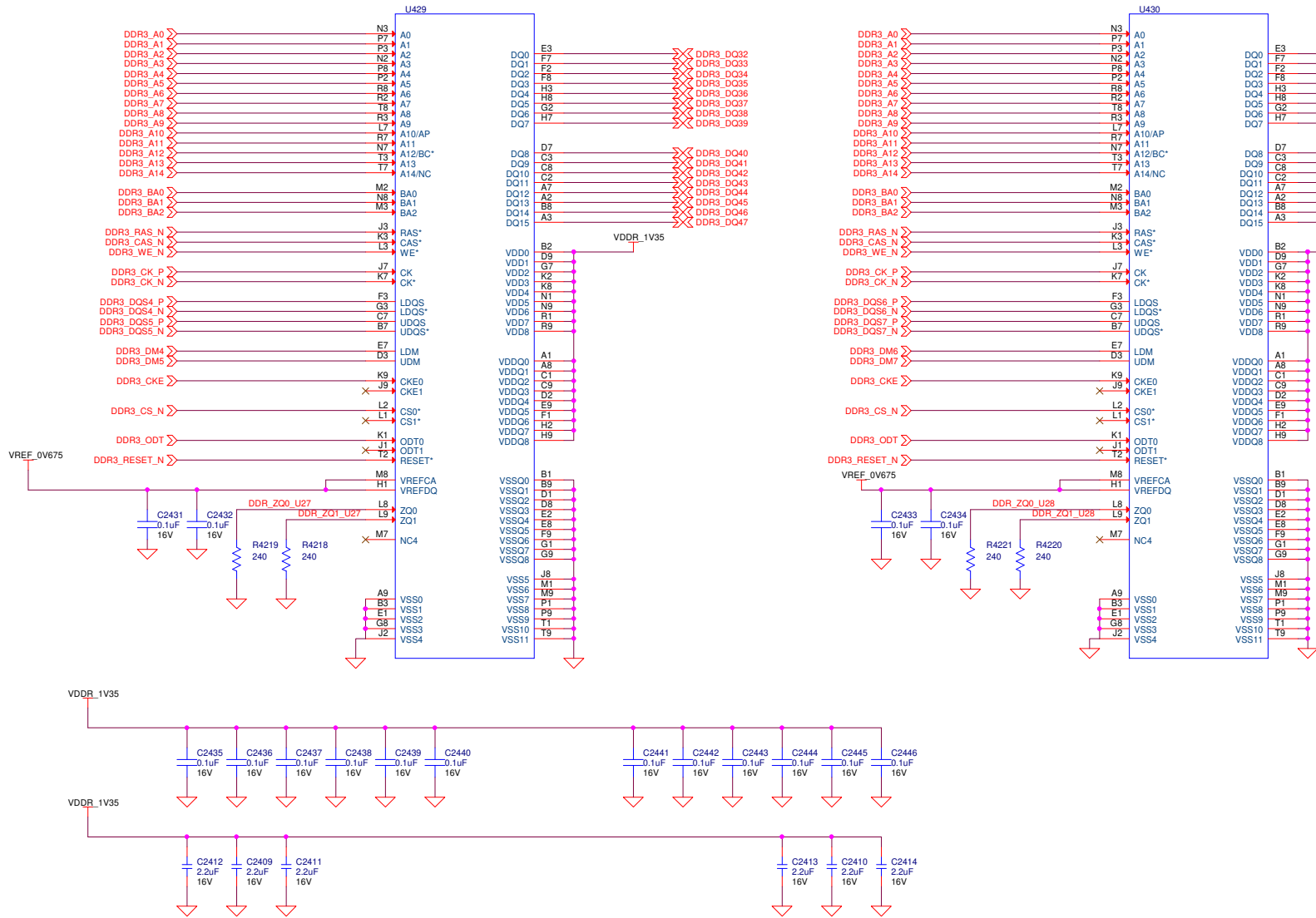
Figure 34. Schematic Page 19
