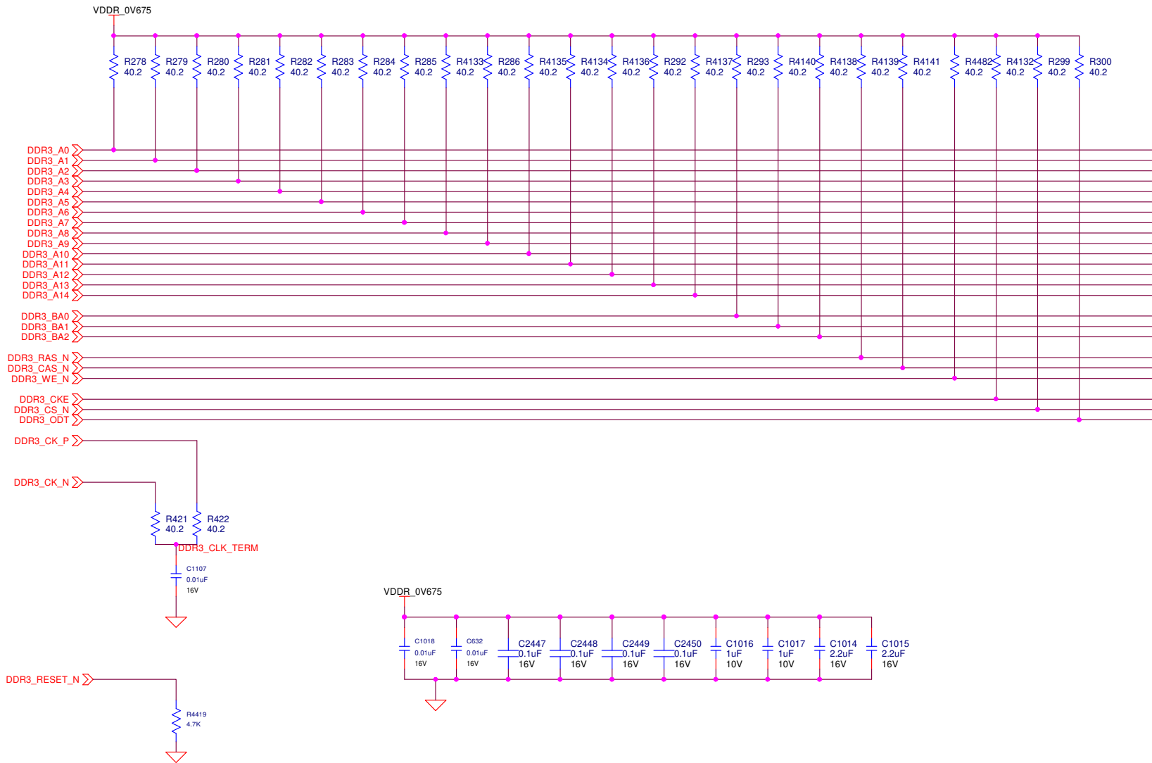
Figure 35. Schematic Page 20
