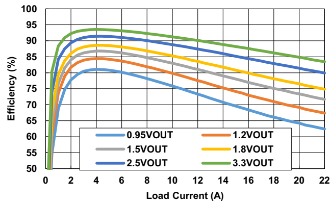
Figure 10. ISL70002SEH Efficiency, V_{IN} = 5V , 500kHz
