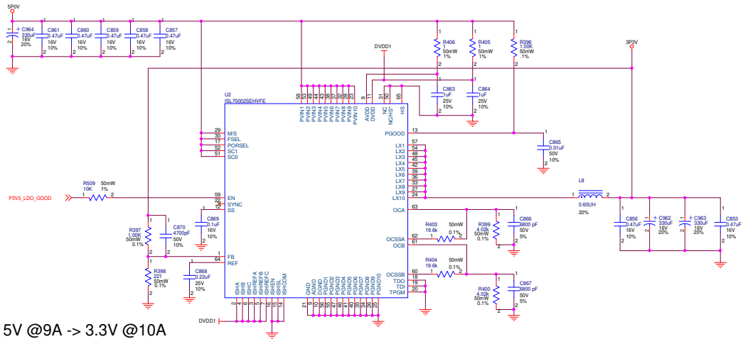
Figure 40. Schematic - Power Supplies-1
