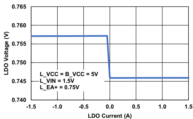
Figure 67. ISL70005SEH LDO Load Regulation
