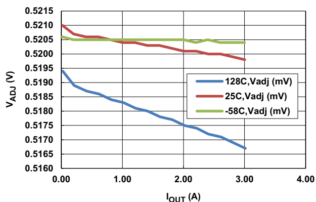
Figure 68. ISL75051ASEH Load Regulation, V_{ADJ} vs I_{OUT}
