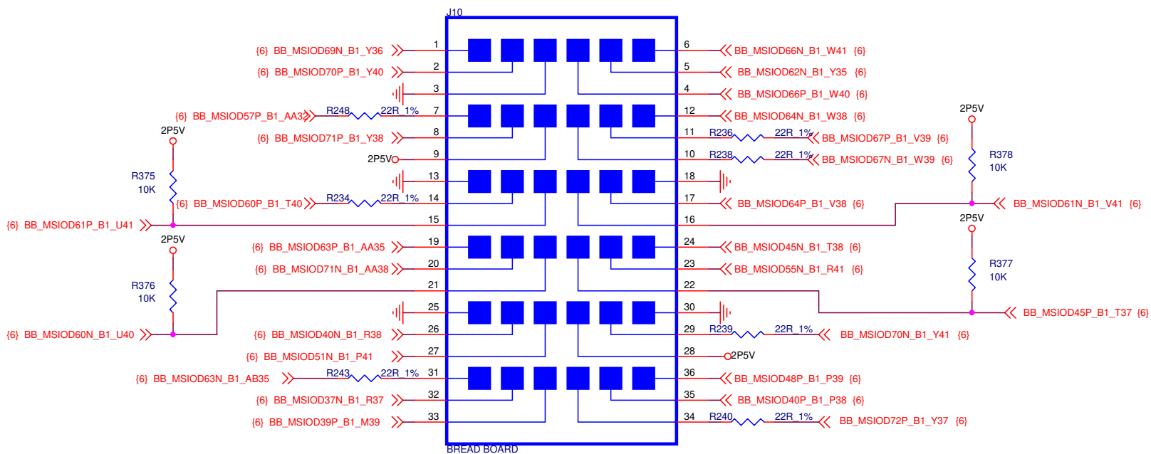
Figure 30. Schematic - Bread Board Connector
