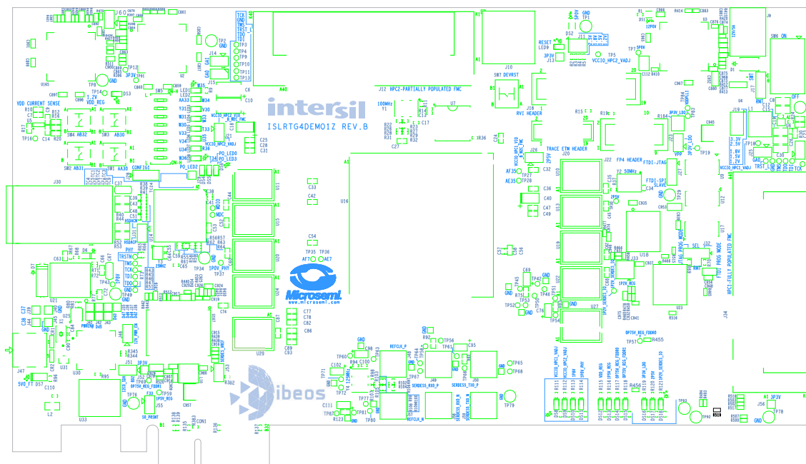
Figure 47. Silkscreen Top
