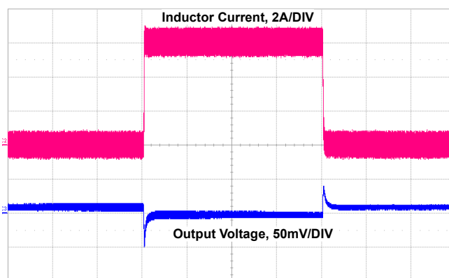
Figure 64. ISL70003ASEH 6A Load Transient Response
