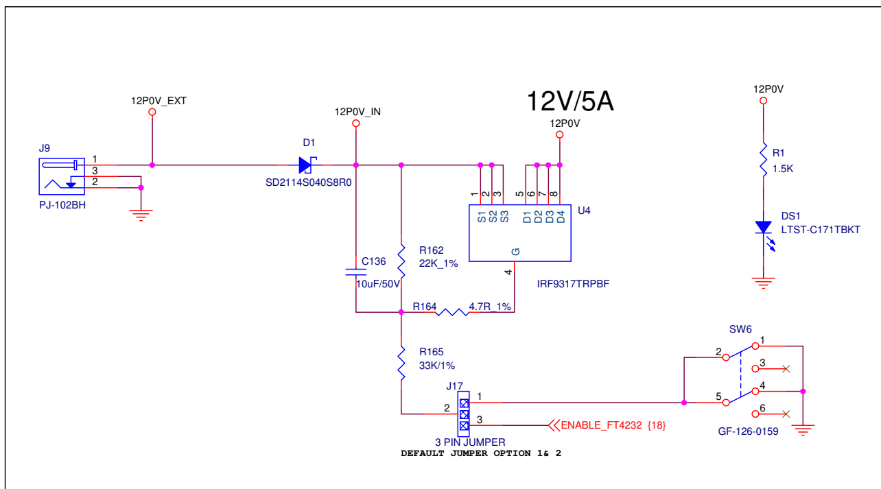
Figure 38. Schematic - 12V Power Supply Connection
