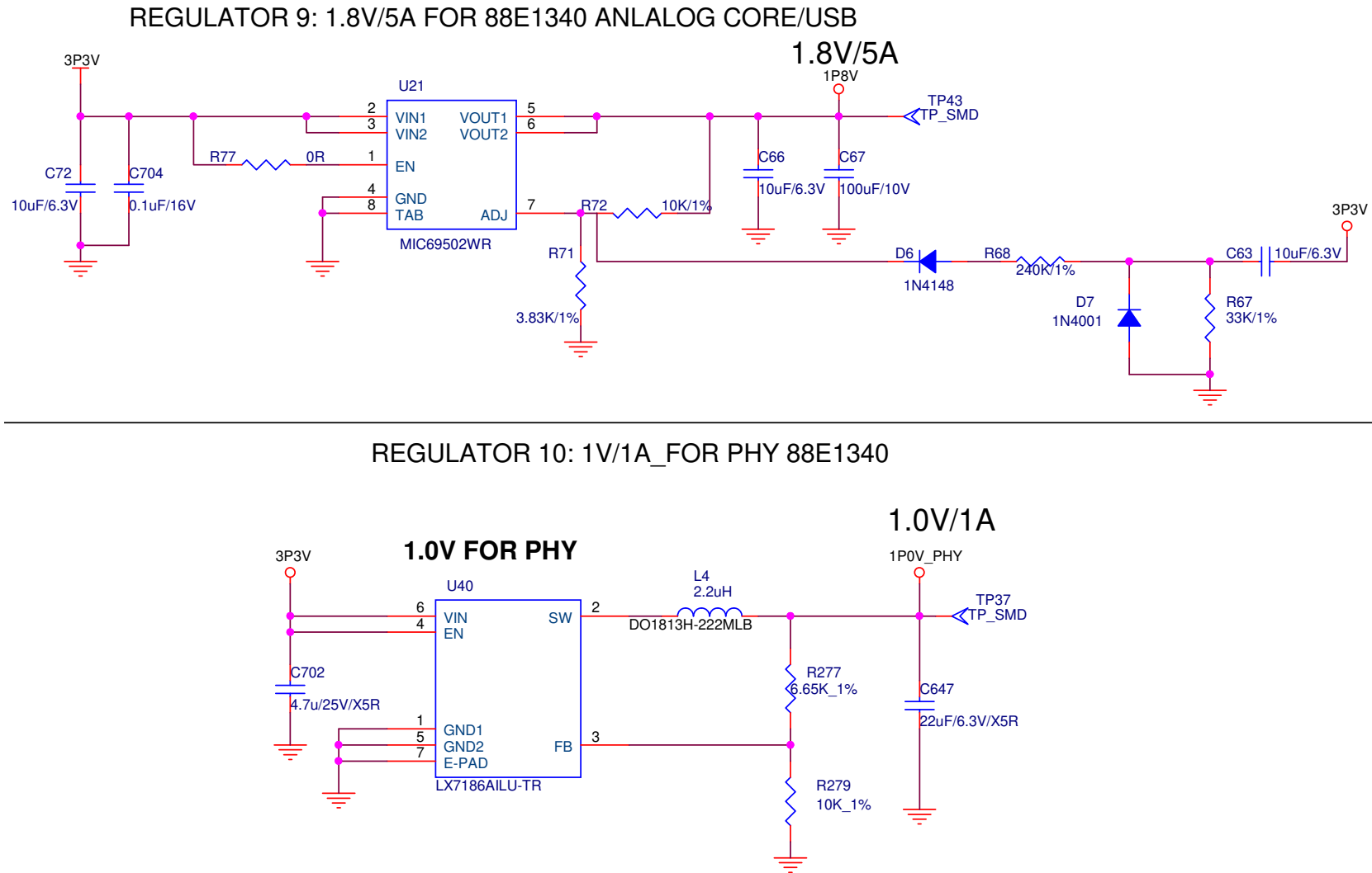
Figure 44. Schematic - Power Supplies-5
