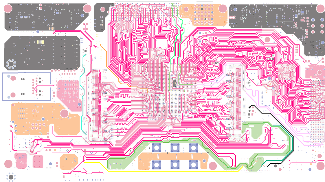
Figure 52. Layer 5
