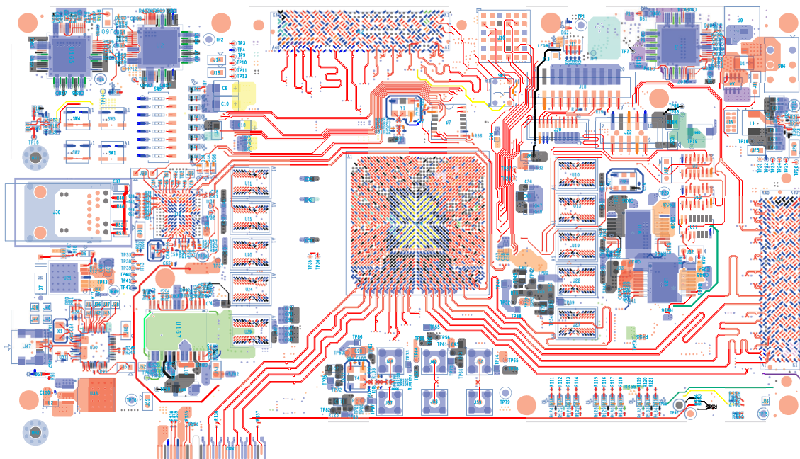
Figure 48. Top Layer
