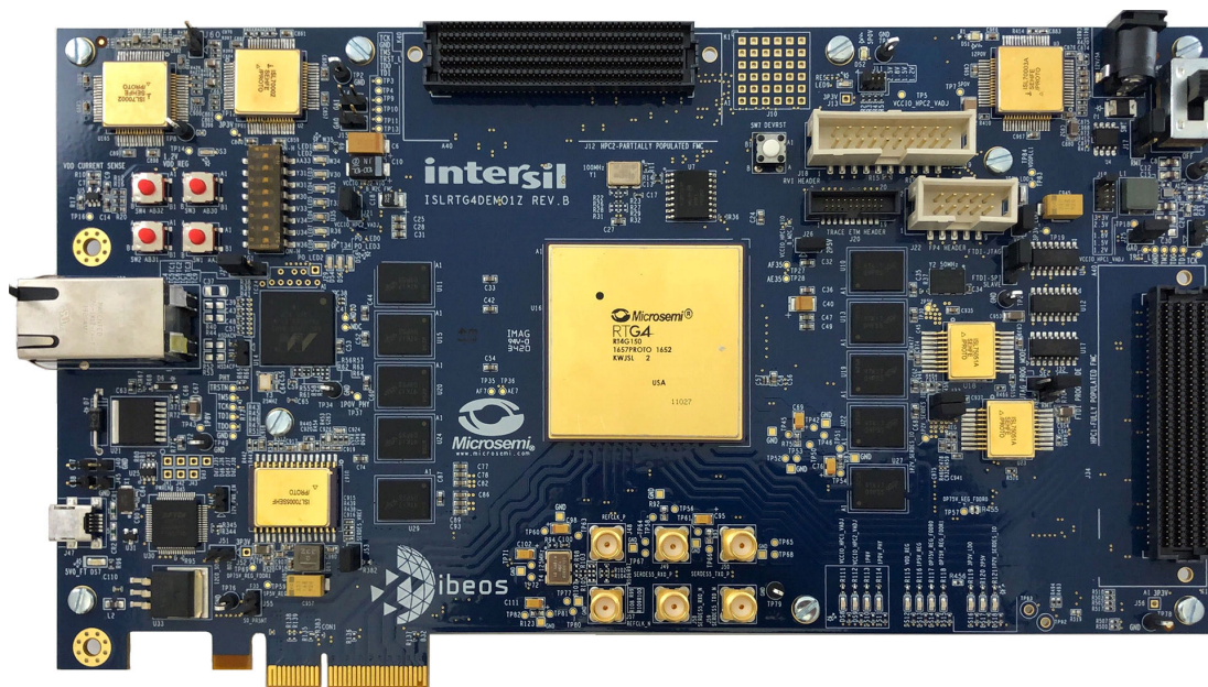
Figure 3. ISLRTG4DEMO1Z Reference Design (Top)
