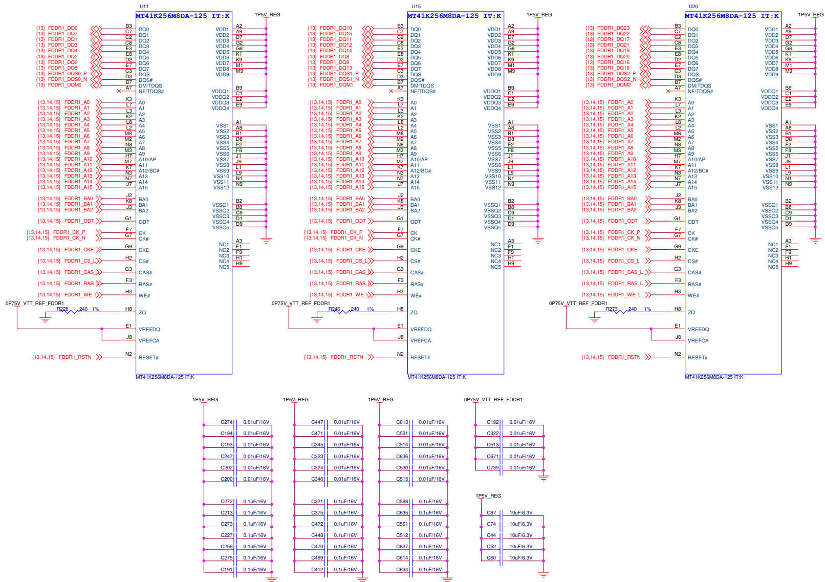
Figure 16. Schematic - DDR3-SDRAM Interface 1 - FDDR1
