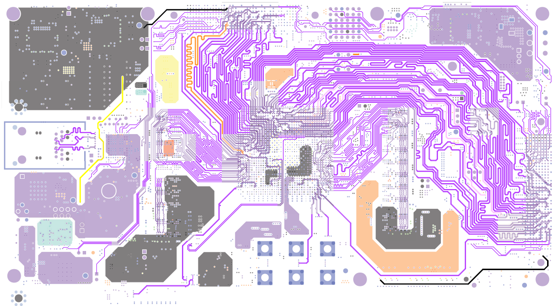
Figure 50. Layer 3
