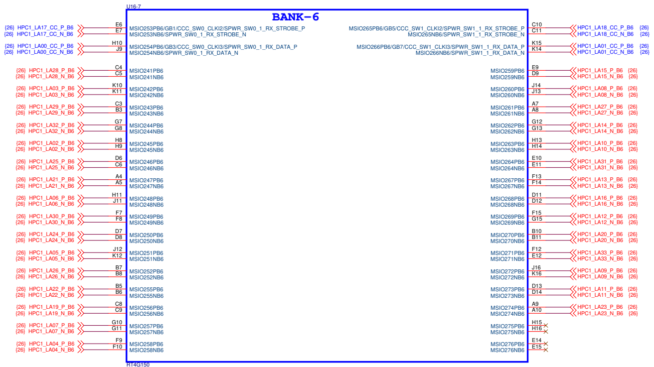
Figure 12. Schematic - Bank-6
