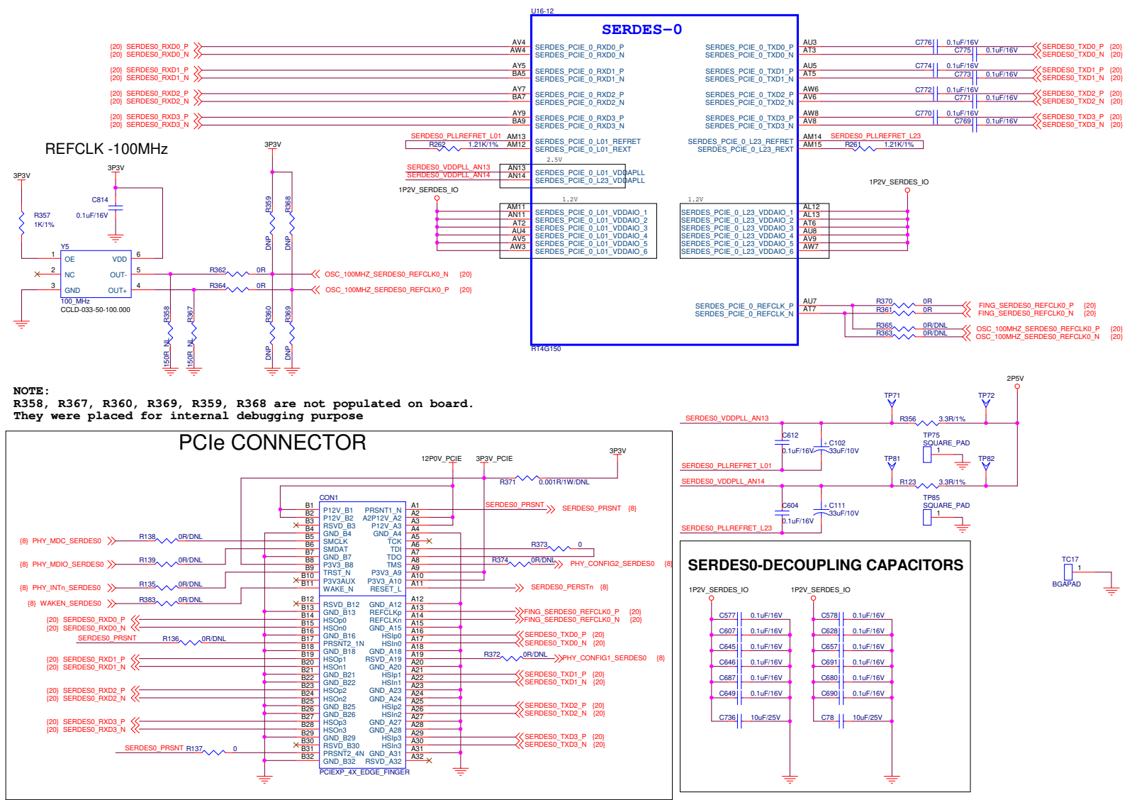
Figure 22. Schematic - SerDes-0 Connection
