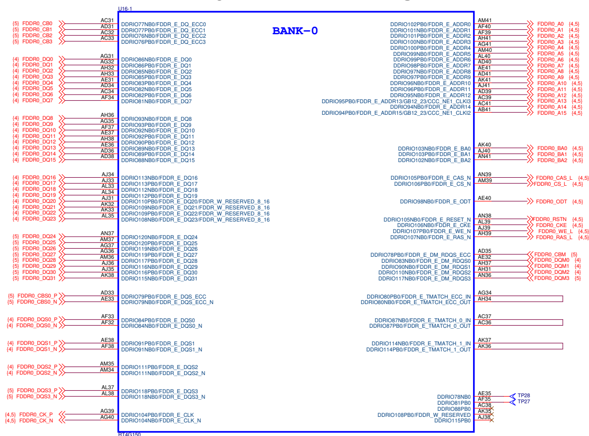
Figure 5. Schematic - Bank-0
