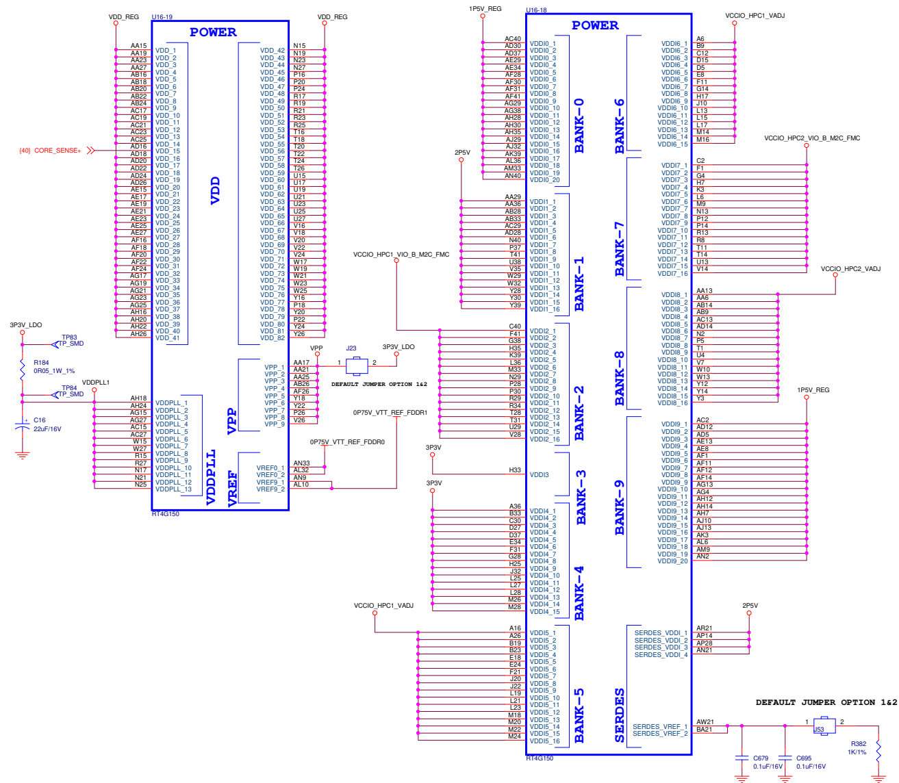
Figure 35. Schematic - Power Connection
