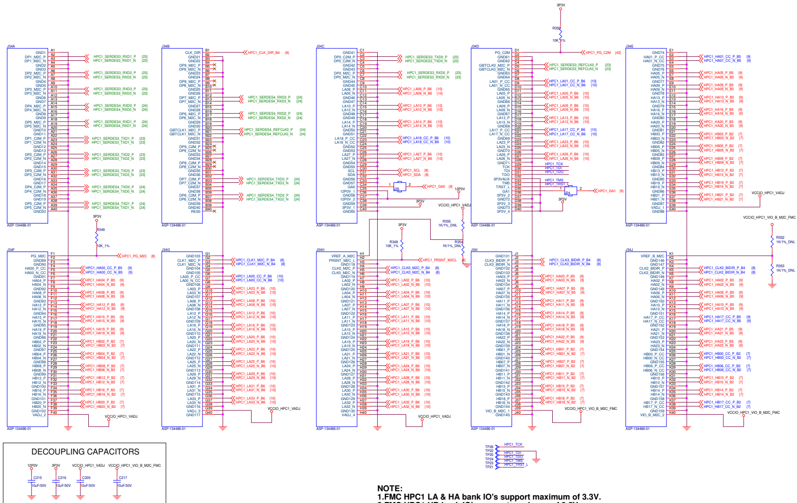
Figure 28. Schematic - FMC Connector - HPC1
