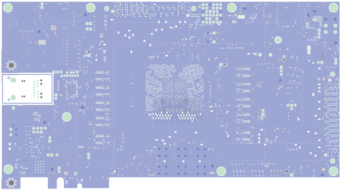
Figure 56. Layer 9
