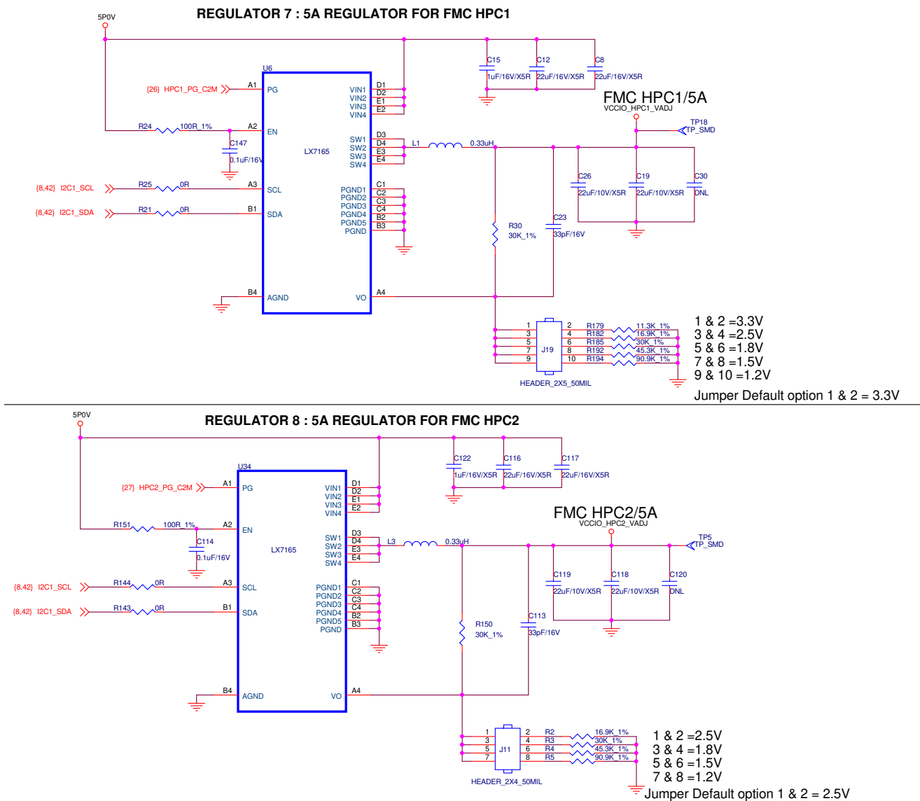
Figure 43. Schematic - Power Supplies-4
