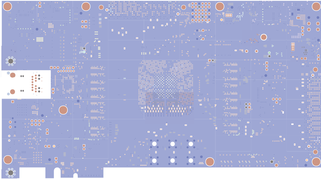
Figure 51. Layer 4
