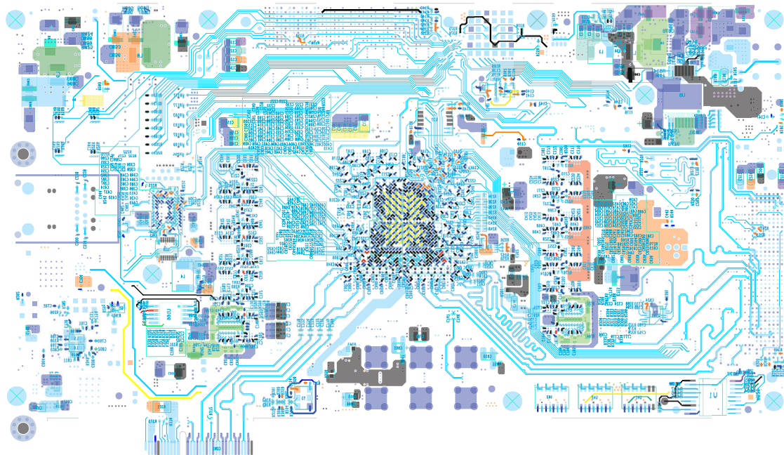
Figure 61. Bottom Layer
