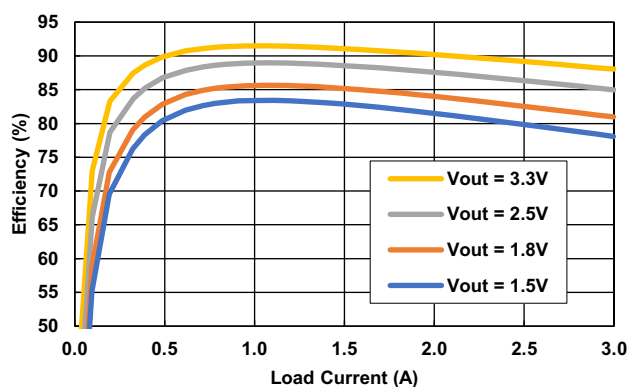
Figure 66. ISL70005SEH Buck Efficiency, V_{IN} = 5V , 1MHz
