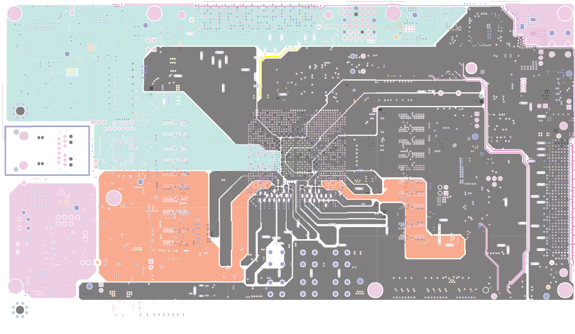
Figure 55. Layer 8
