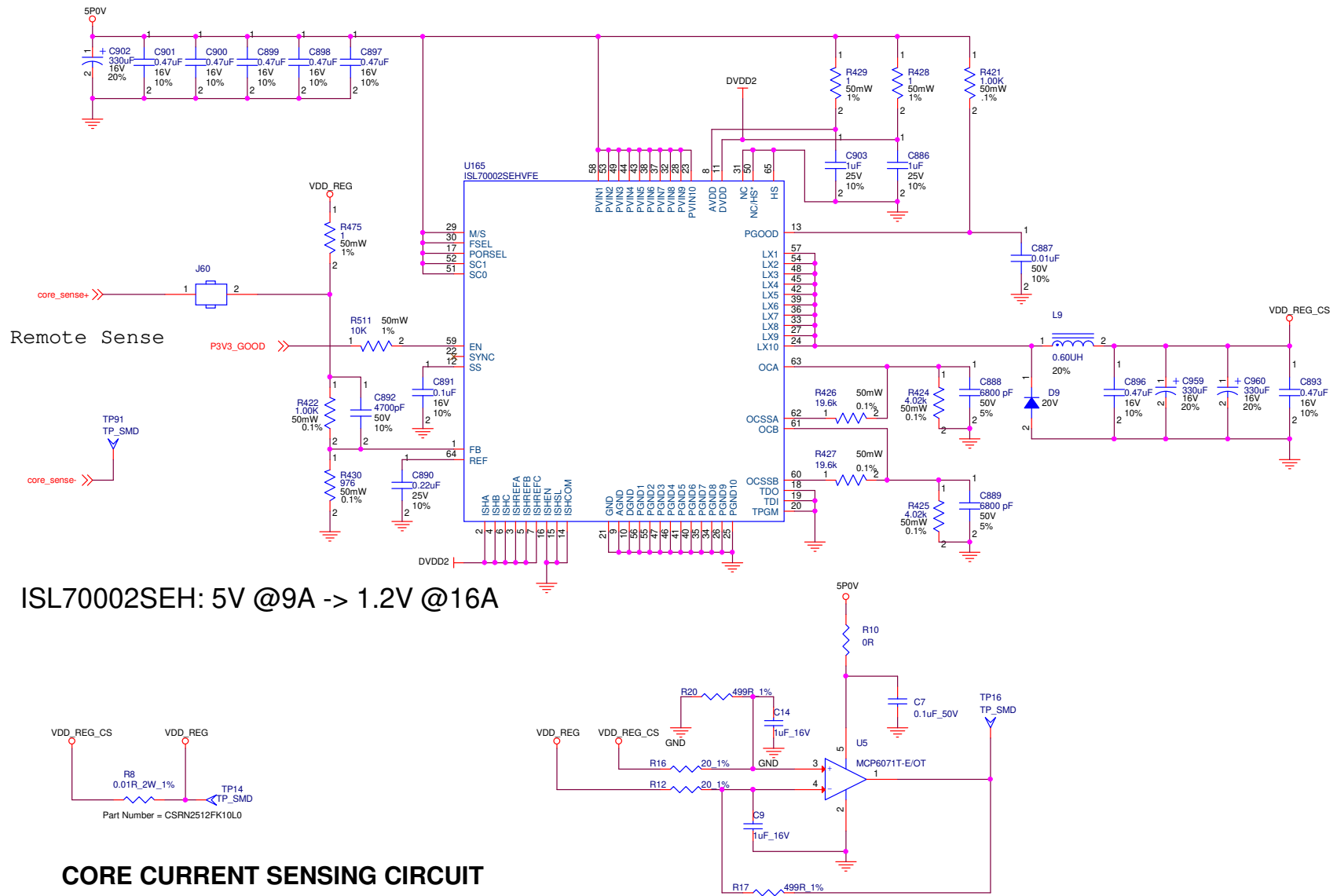
Figure 41. Schematic - Power Supplies-2
