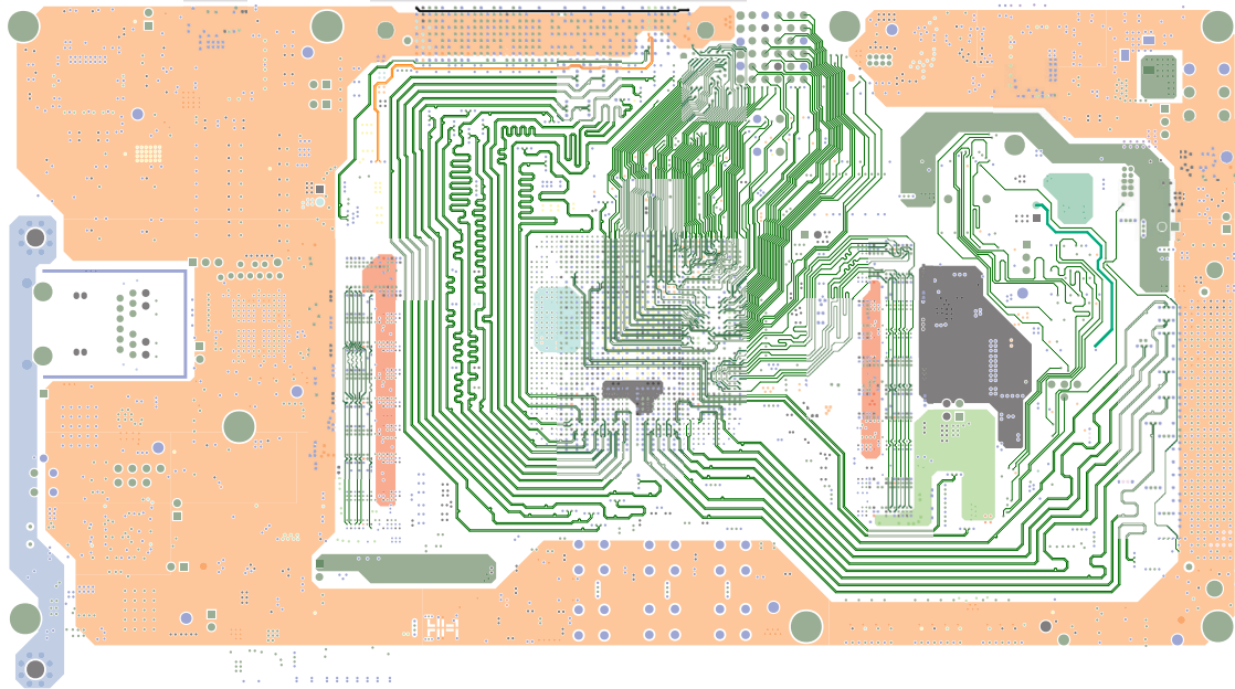
Figure 59. Layer 12
