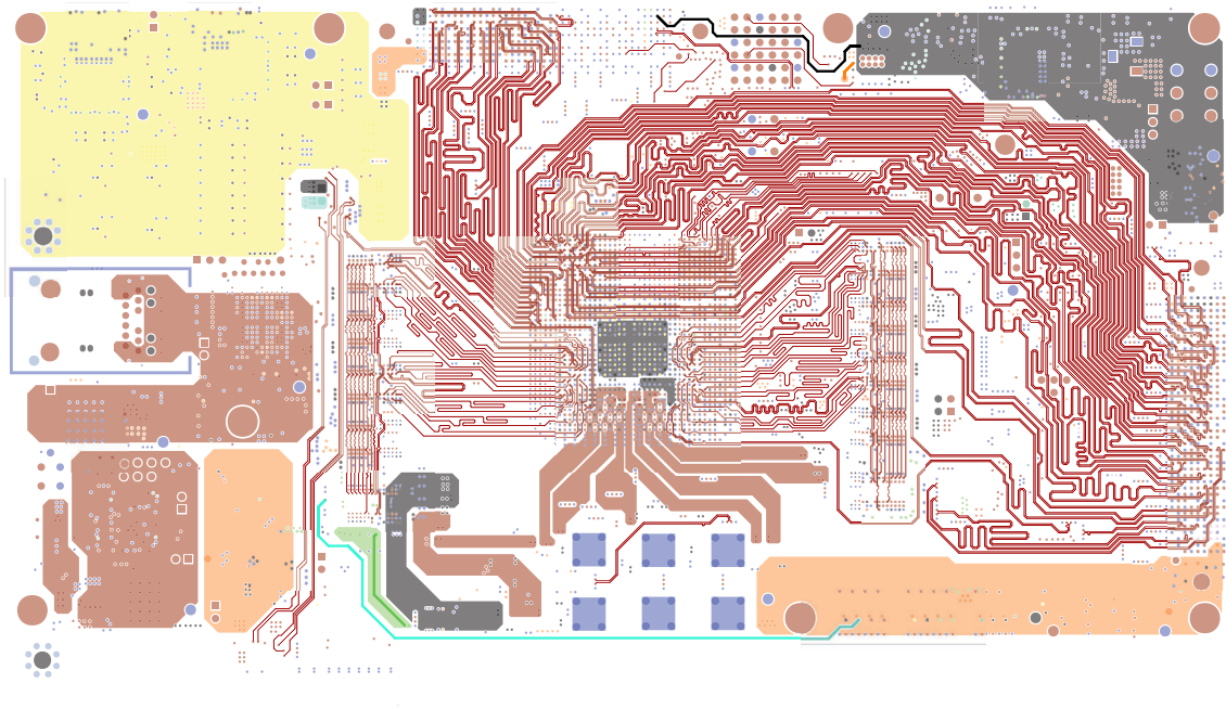
Figure 57. Layer 10
