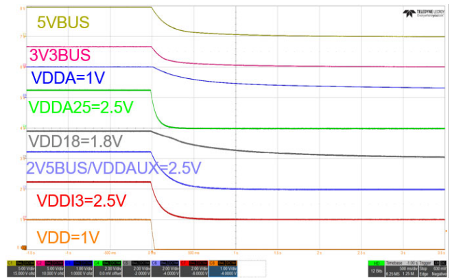
Figure 40. Shutdown, Rails 1-8, 50mA on VDD
