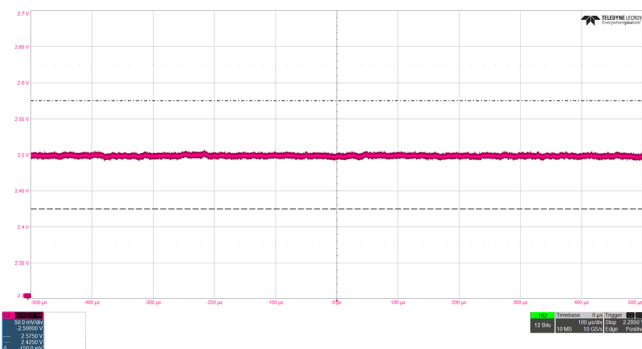
Figure 15. VDD25/VDDA25 Output Voltage, ISL75054, 2.5V/0.25A, \pm 75mV Limits
