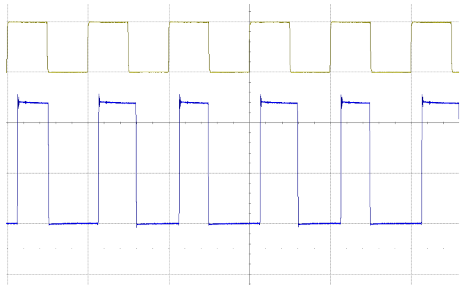
Figure 52. 5VBUS Switching Waveform, ISL73007, 5V/2A, (C1 = SYNC, C3 = LX)
