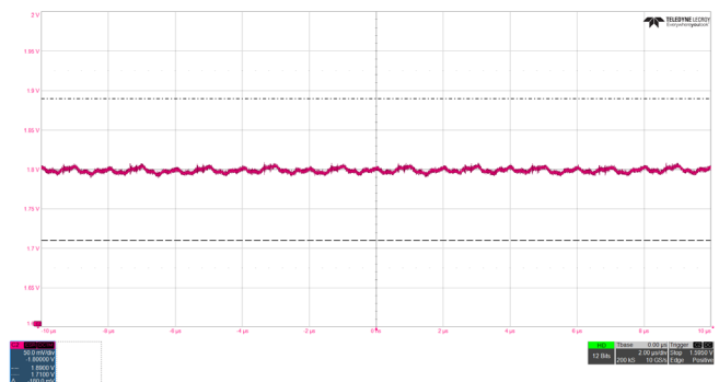
Figure 16. Figure 14. VDD18 Output Voltage Ripple, ISL73007, 1.8V/0.5A, \pm 90mV Limits
