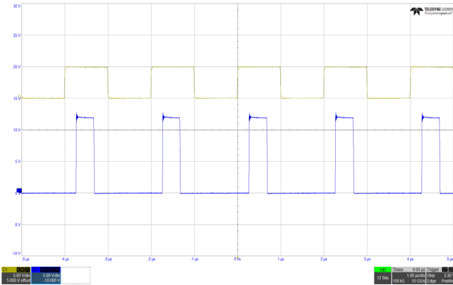
Figure 49. VDDAUX[2,4,5]/VPP/2V5BUS Switching Waveform, ISL73007, (C1 = SYNC, C3 = LX)
