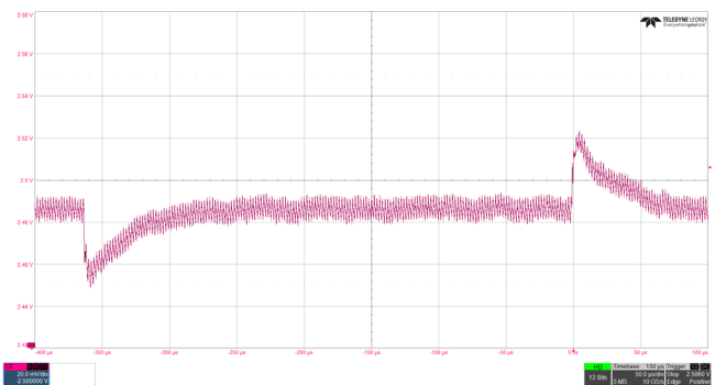
Figure 34. VDDAUX[2,4,5]/VPP/2V5BUS Output Voltage, Load Transient Response, ISL73007, 2.5V at 25% to 75% Load Step, ±200mV Limits
