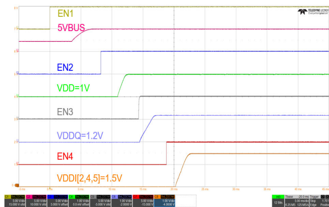
Figure 41. Sequencer Startup, No Load
