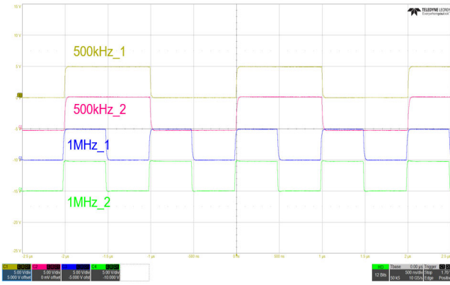
Figure 43. Quad Clock Signals, ISL74420
