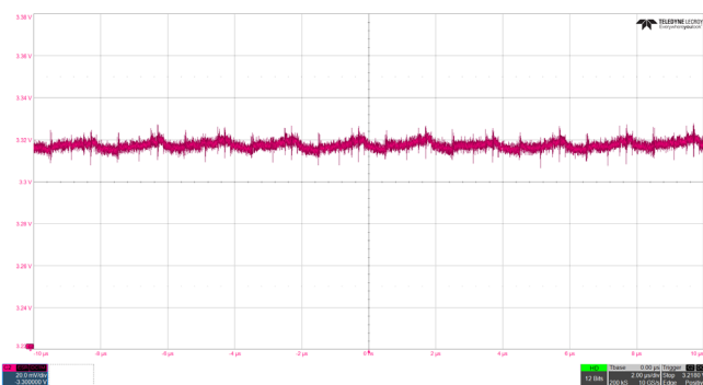
Figure 25. 3V3BUS Output Voltage Ripple, ISL73007, 3.3V/3A
