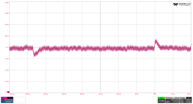
Figure 30. VDD18 Output Voltage, Load Transient Response, ISL73007, 1.8V at 25% to 75% Load Step, ±200mV Limits
