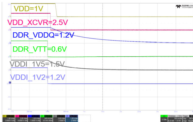
Figure 39. Shutdown, Rails 8 to 13, 50mA on VDD, VDDI_1V2
