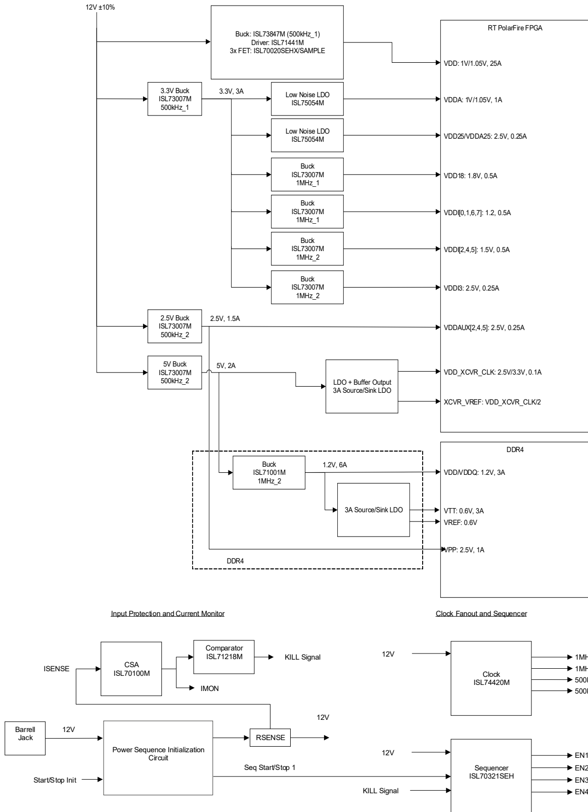
Figure 3. Renesas Radiation Tolerant Power Tree for Microchip RT PolarFire FPGA
