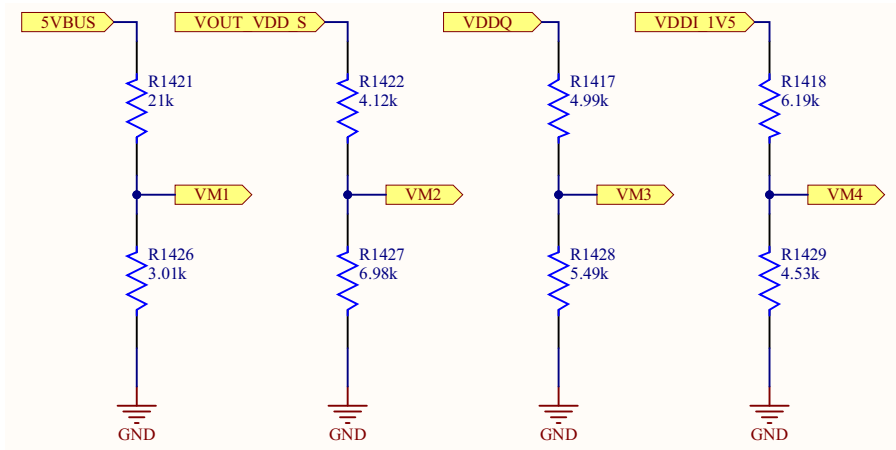
Figure 8. Power Supply Sequence Voltage Monitor Dividers
