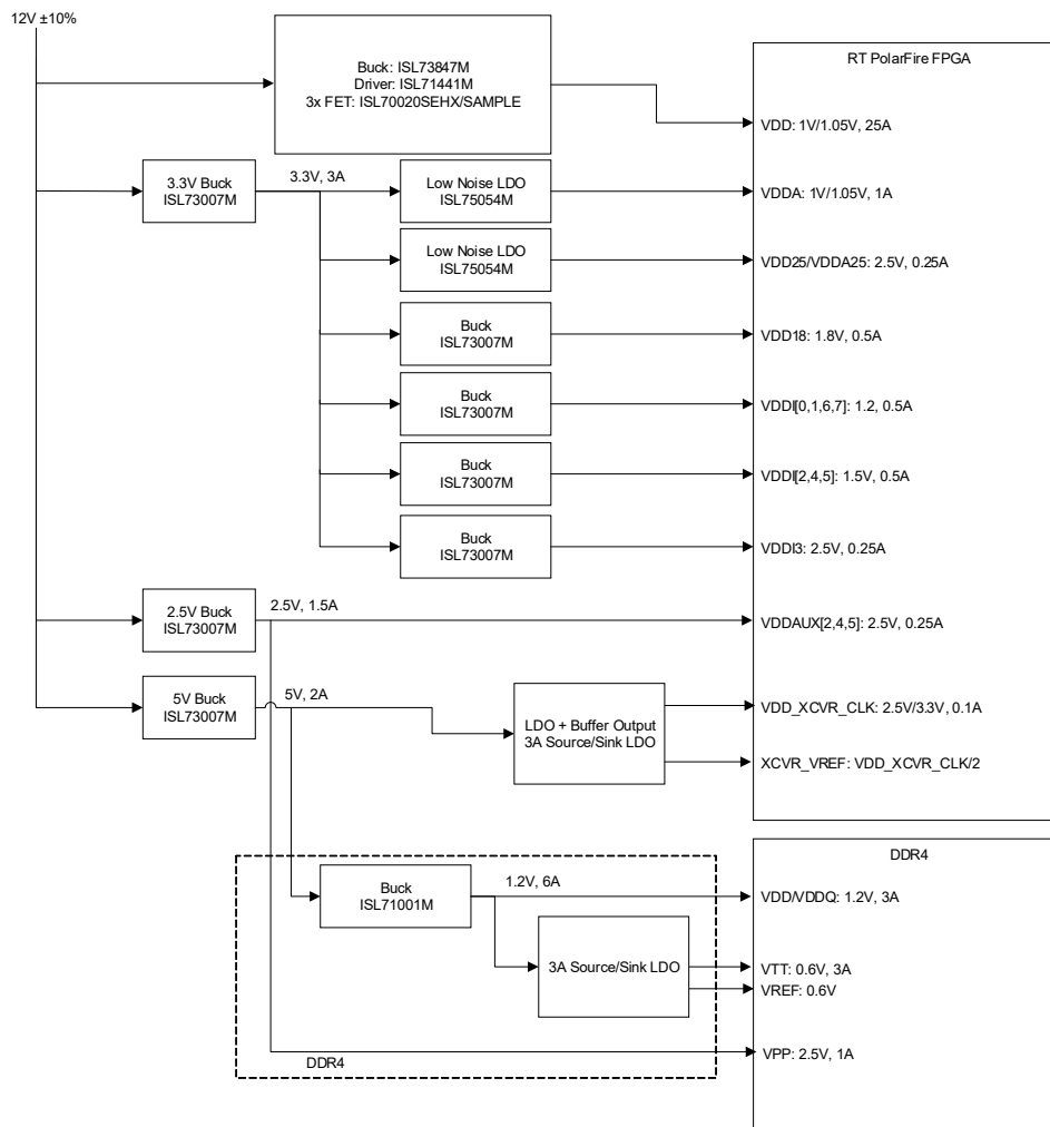
Figure 1. Power Management Block Diagram
