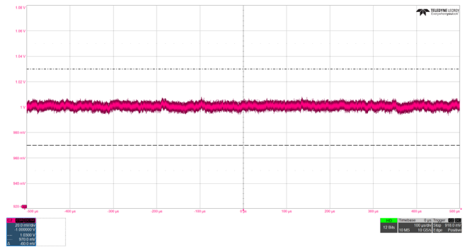
Figure 14. VDDA Output Voltage, ISL5054, 1V/1A, \pm 30mV Limits
