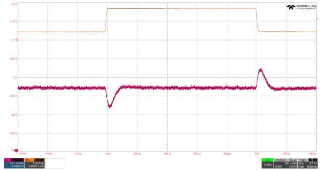
Figure 36. 5VBUS Output Voltage Ripple, Load Transient Response, ISL73007, 5V at 25% to 75% Load Step from External E-Load (C2 = V OUT , C8 = I OUT )
