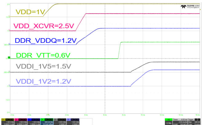
Figure 38. Startup, Rails 8-13, No Load
