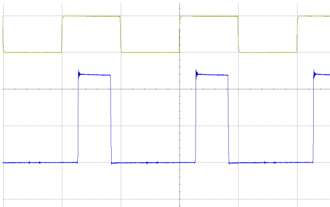
Figure 51. 3V3BUS Switching Waveform, ISL73007, 3.3V/3A, (C1 = SYNC, C3 = LX)
