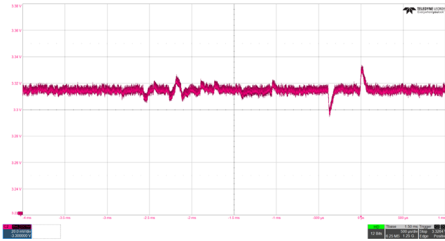
Figure 35. 3V3BUS Output Voltage, Load Transient Response, ISL73007, 3.3V w/ Downstream Transient Generators Enabled (VDDA, VDD25, VDD18, VDDI[0,1,6,7], VDDI[2,4,5], VDDI3)
