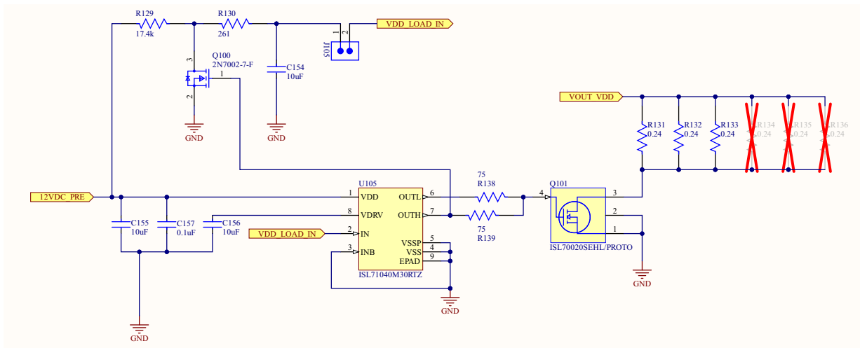
Figure 5. 12.5A VDD Load Transient Circuit using ISL71040 RT GaN FET Driver and ISL70020 GaN Power Transistor
