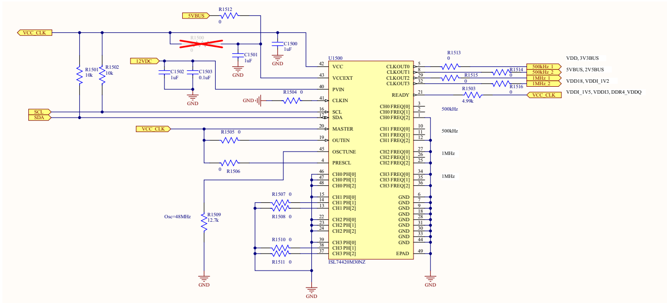
Figure 10. ISL74420 Quad Clock Schematic
