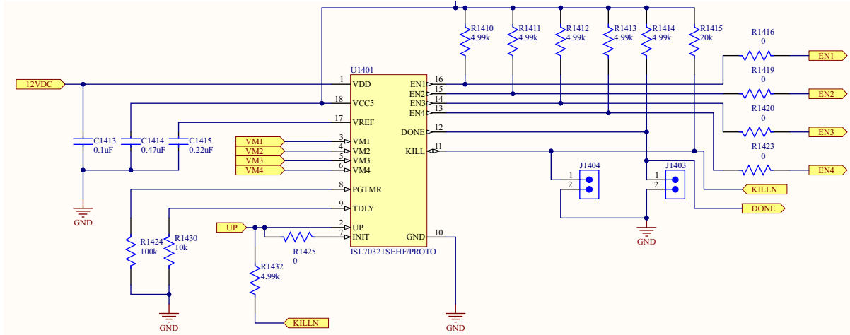
Figure 7. Power Supply Sequencer Schematic
