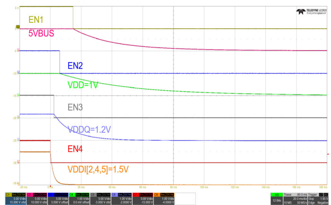
Figure 42. Sequencer Shutdown, 50mA Load (All Four Rails)
