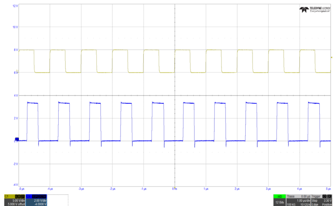
Figure 46. VDDI[0,1,6,7] Switching Waveform, ISL73007, 1.2V/0.5A, (C1 = SYNC, C3 = LX)
