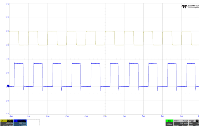
Figure 47. VDDI[2,4,5] Switching Waveform, ISL73007, 1.5V/0.5A, (C1 = SYNC, C3 = LX)
