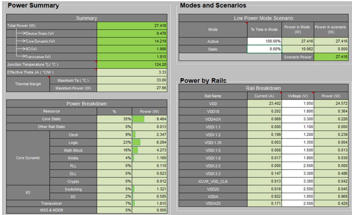
Figure 2. Power Management Specification from Microchip RT PolarFire FPGA Power Estimator Tool
