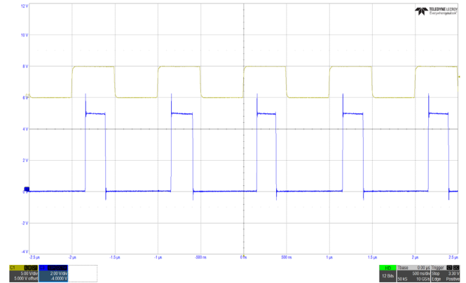
Figure 50. DDR_VDDQ Switching Waveform, ISL71001, 1.2V/6A, (C1 = SYNC, C3 = LX)
