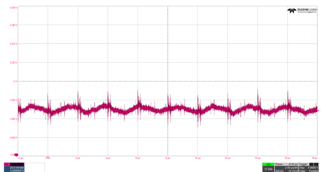
Figure 26. 5VBUS Output Voltage Ripple, ISL73007, 5V/2A
