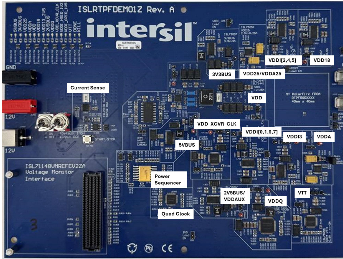
Figure 4. ISL RTPFDEMO1Z Board Photo
