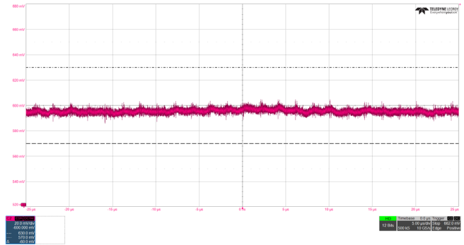
Figure 24. DDR_VTT Output Voltage, 3A Source/Sink LDO, 0.6V/3A, \pm 30\text{mV} Limits
