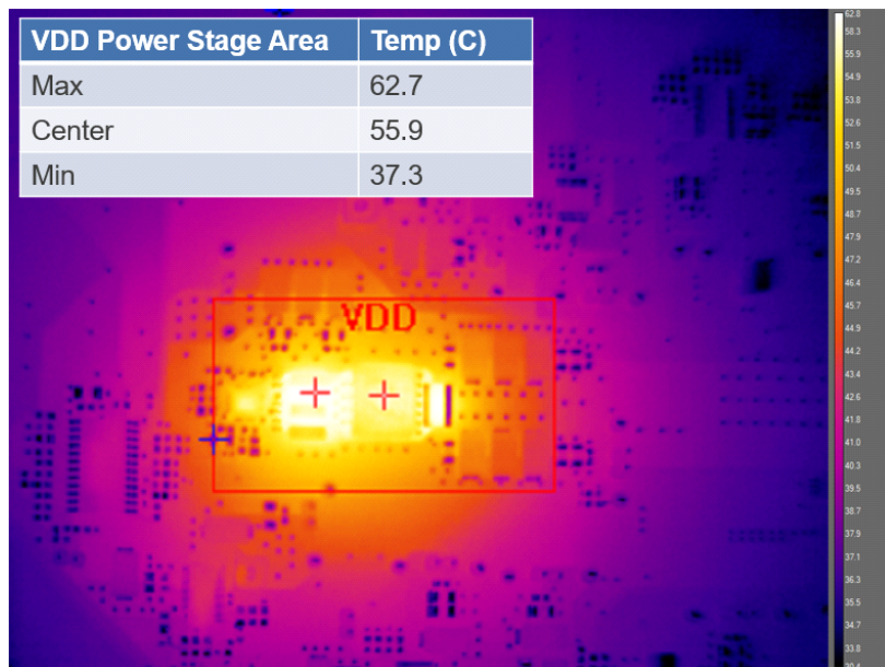
Figure 53. VDD Core Rail Thermal Image, 1V/25A, Open Air (25C Ambient)
