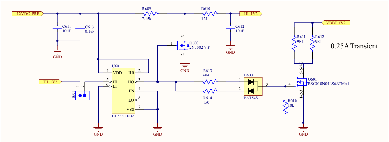
Figure 6. Typical Load Transient Circuit using HIP2211 HB Driver
