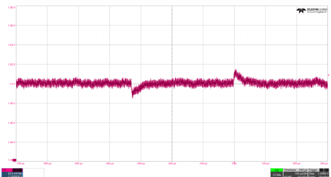
Figure 32. VDDI[2,4,5] Output Voltage, Load Transient Response, ISL73007, 1.5V at 25% to 75% Load Step, ±150mV Limits
