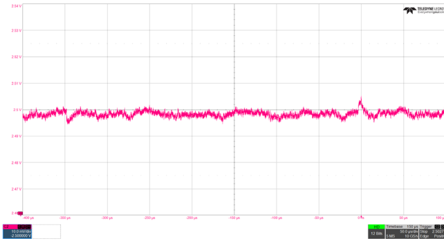
Figure 29. VDD25/VDDA25 Output Voltage, Load Transient Response, ISL75054, 2.5V at 25% to 75% Load Step, ±200mV Limits
