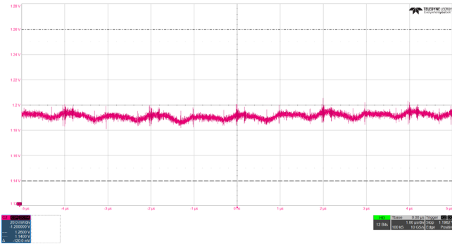
Figure 23. DDR_VDDQ Output Voltage Ripple, ISL71001, 1.2V/6A, \pm 60\text{mV} Limits
