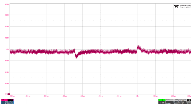
Figure 31. VDDI[0,1,6,7] Output Voltage, Load Transient Response, ISL73007, 1.2V at 25% to 75% Load Step, ±120mV Limits
