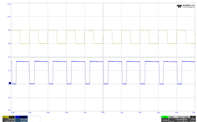
Figure 48. VDDI3 Switching Waveform, ISL73007, 2.5V/0.25A, (C1 = SYNC, C3 = LX)
