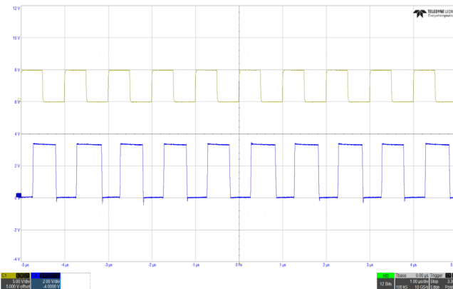
Figure 45. VDD18 Switching Waveform, ISL73007, 1.8V/0.5A, (C1 = SYNC, C3 = LX)
