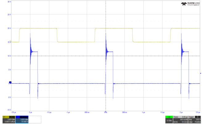
Figure 44. VDD Switching Waveform, ISL73847, 1V/25A (C1 = SYNC, C3 = LX)
