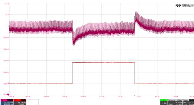
Figure 27. VDD Output Voltage, Load Transient Response, ISL73847, 1V at 25% to 75% Load Step, \pm 130\text{mV} Limits (C2 = VOUT, C7 = VLOAD)
