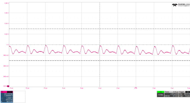
Figure 13. VDD Output Voltage Ripple, ISL73847, 1V/25A, \pm 30mV Limits
