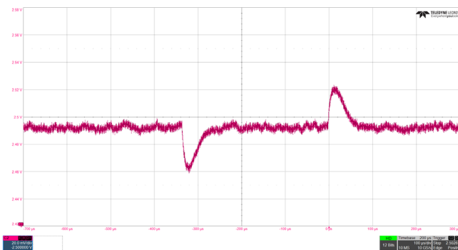
Figure 33. VDDI3 Output Voltage, Load Transient Response, ISL73007, 2.5V at 25% to 75% Load Step, ±180mV Limits
