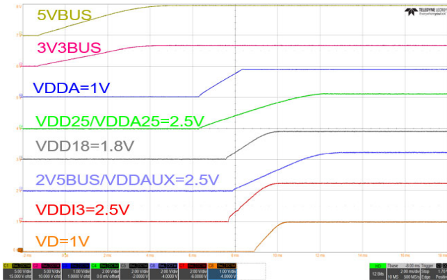
Figure 37. Startup, Rails 1-8, No Load
