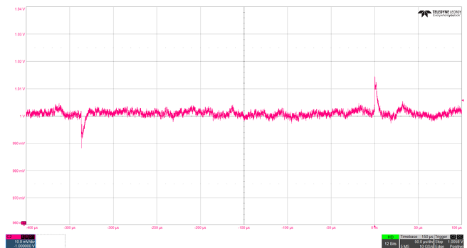
Figure 28. VDDA Output Voltage, Load Transient Response, ISL5054, 1V at 25% to 75% Load Step, \pm 130\text{mV} Limits
