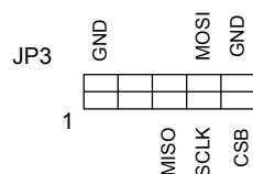
FIGURE 3. JP3 PINOUT
