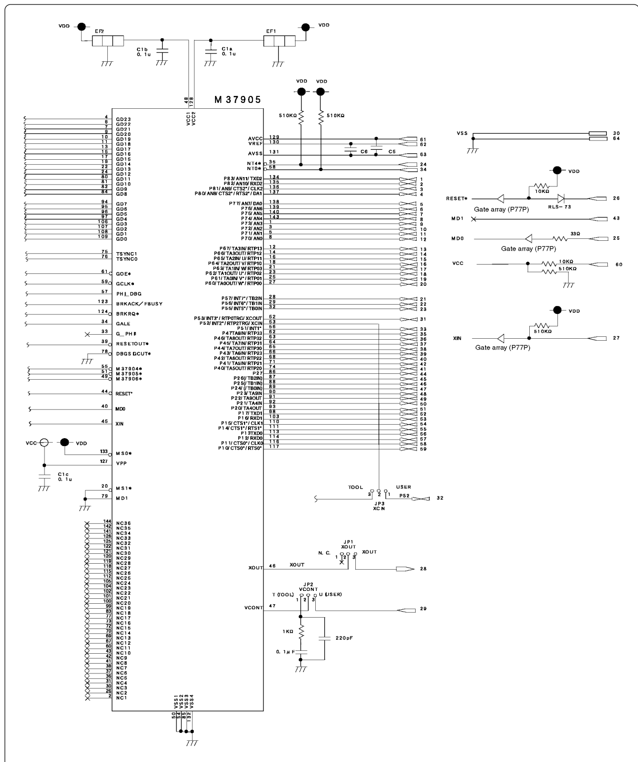
Figure 4.1 Connection diagram
