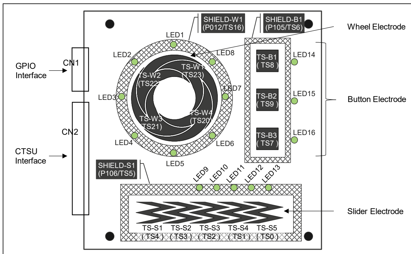
Figure 11 Capacitive Touch Application Board (connected to RA0L1 Cap Touch CPU board)
