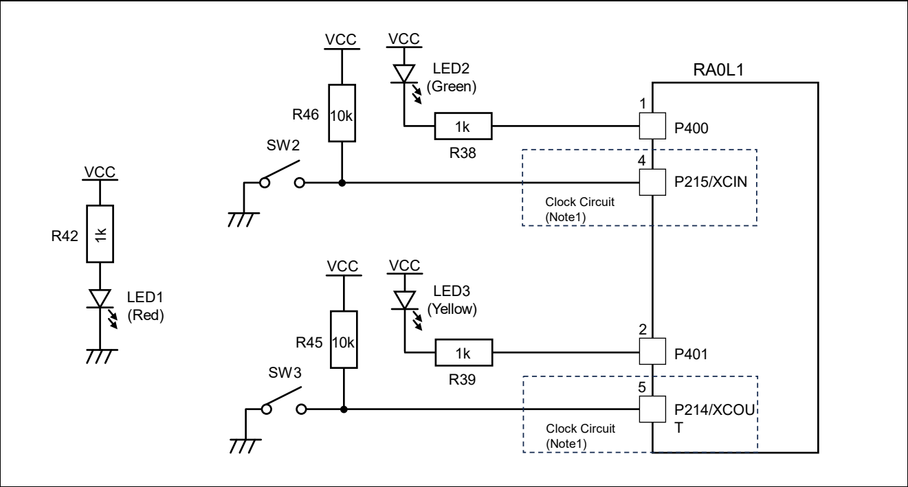
Figure 9 Push Switch and LED Circuits
