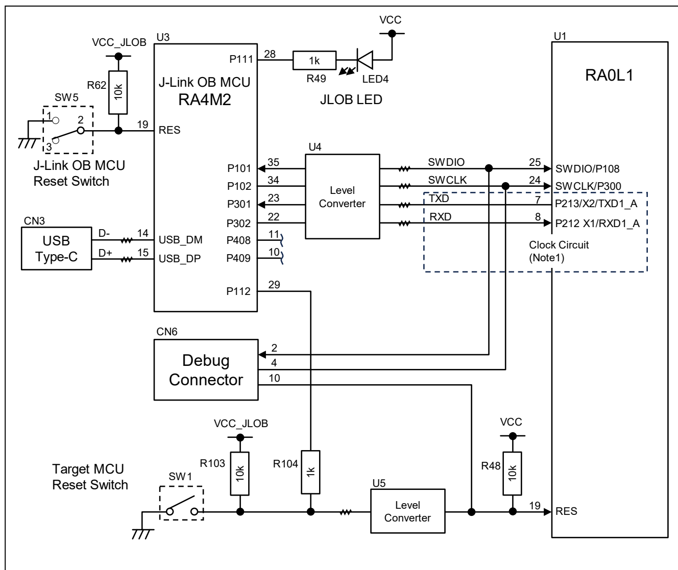
Figure 8 Reset Circuit / Debug Interface
