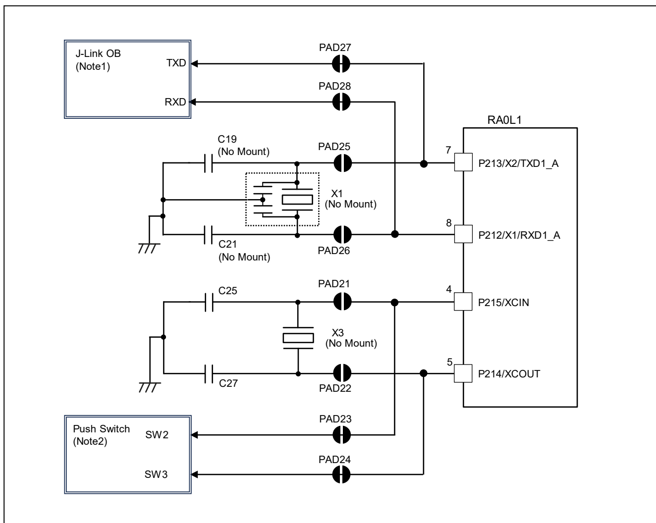
Figure 7 Clock Circuit
