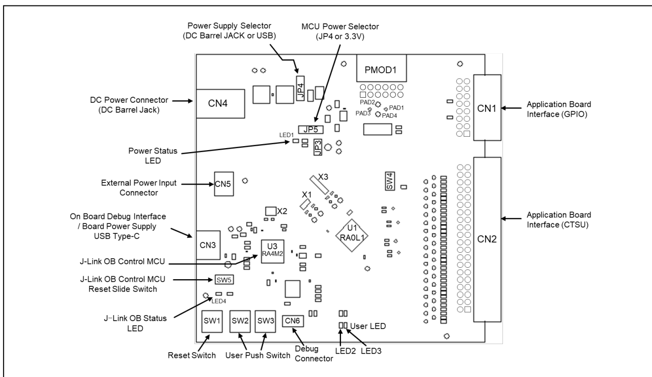
Figure 1 RA0L1 Cap Touch CPU Board
