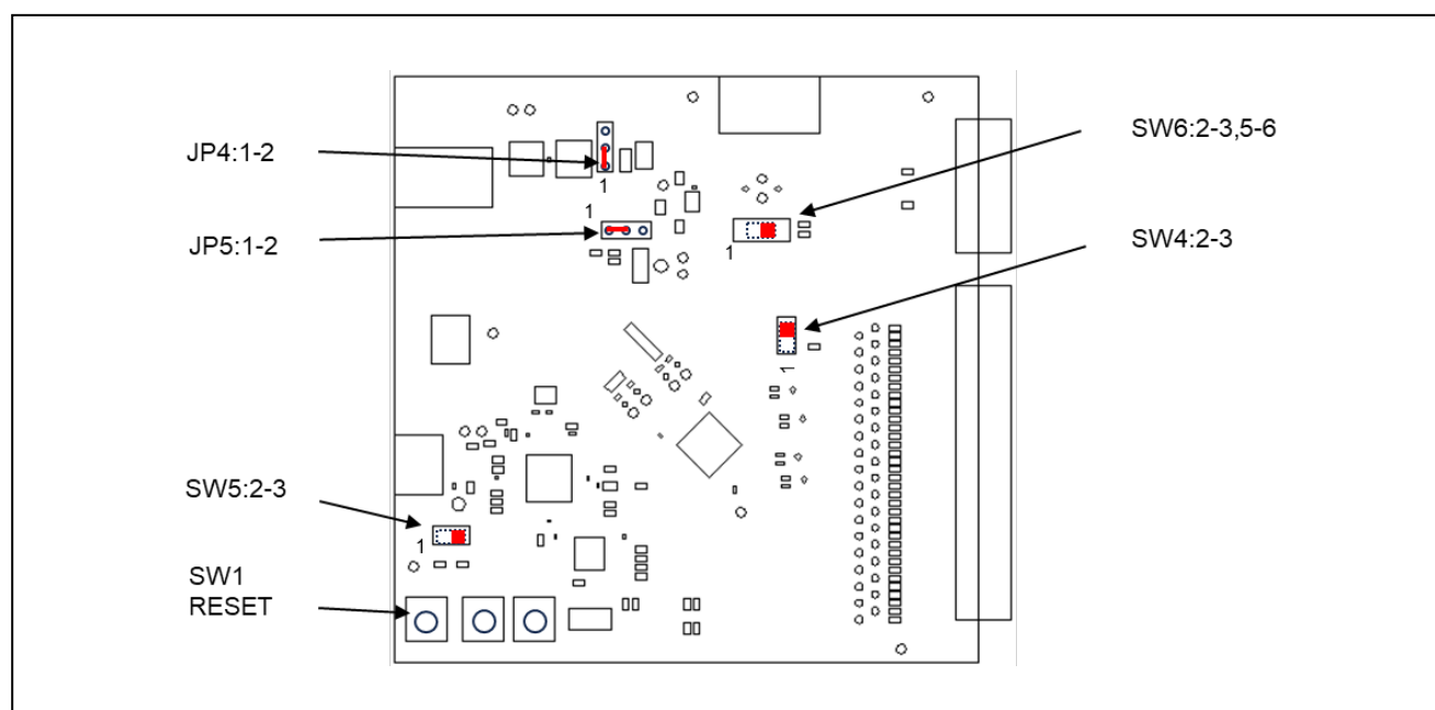
Figure 4 Board Switch Layout
