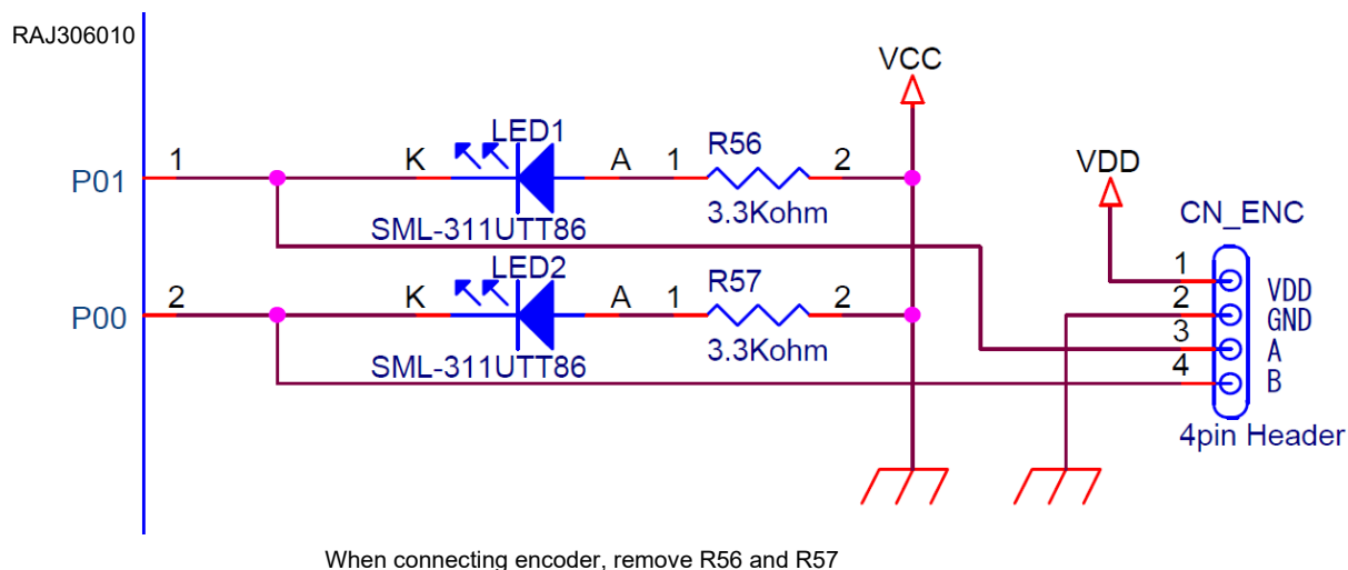
Figure 4-10. Encoder terminal
