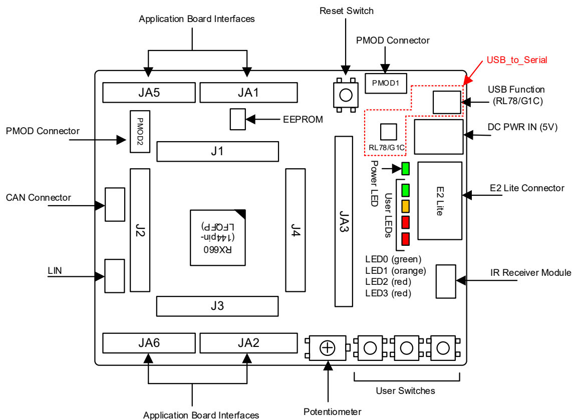
Figure 3-1: Board Layout
