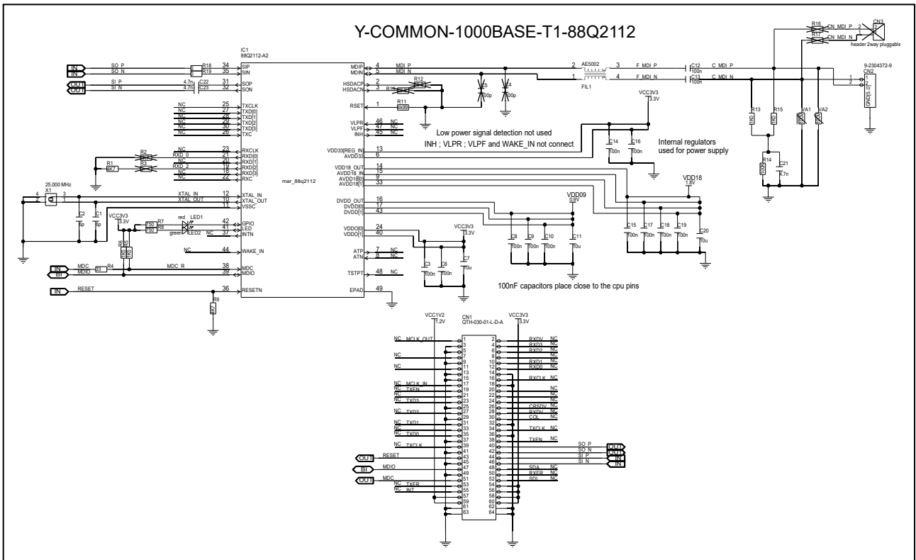
Figure 4.10 Circuit diagram of Renesas Ethernet board Y-COMMON-1000BASE-T1-88Q2112
