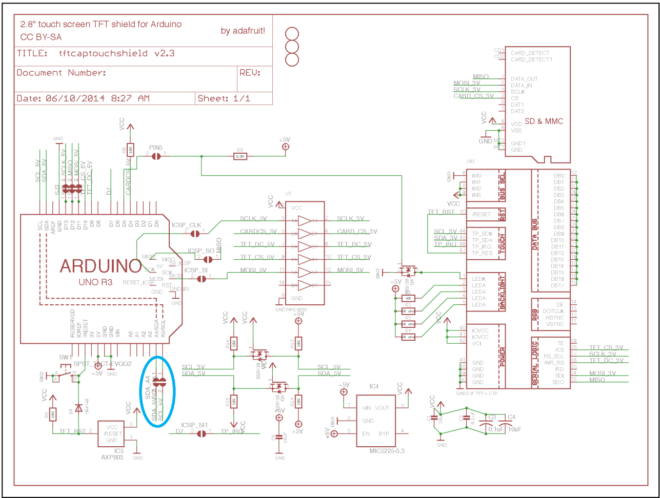
Figure 5.46 Touch display
