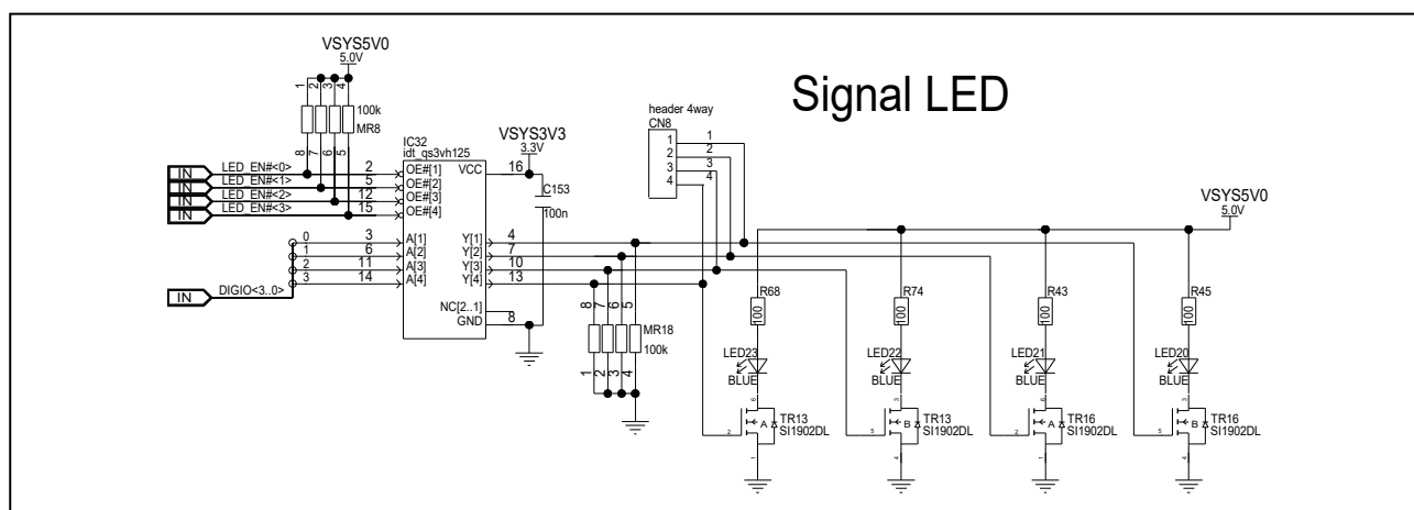
Figure 5.70 Signal LEDs
