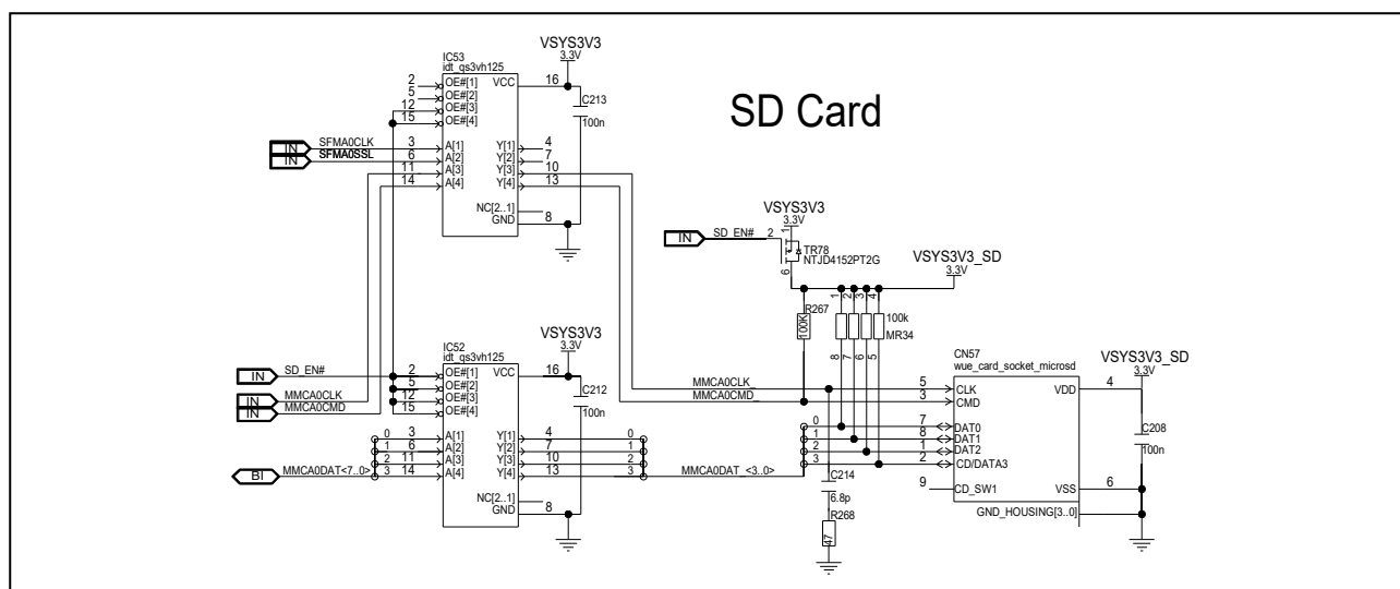
Figure 5.43 MicroSD card circuit of board version D019712_06_V01
