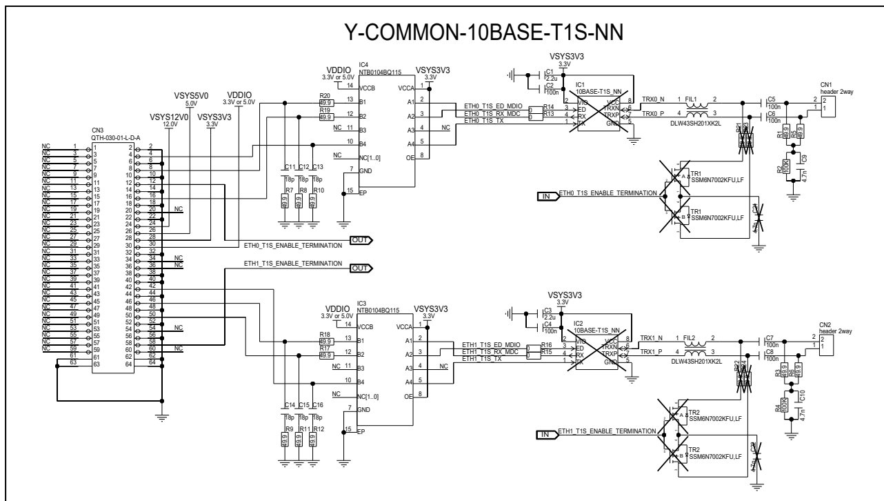
Figure 5.28 Circuit diagram of Renesas Ethernet board Y-COMMON-10BASE-T1S-NN
