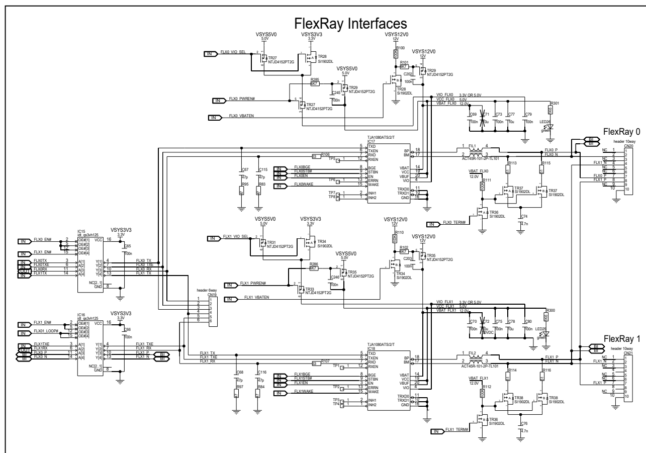
Figure 5.19 FlexRay interface circuit diagram of board version D019712_06_V04 and later
