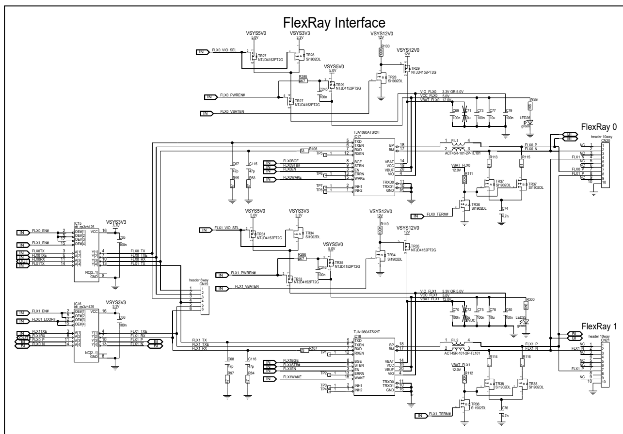
Figure 5.18 FlexRay interface circuit diagram of board version D019712_06_V03
