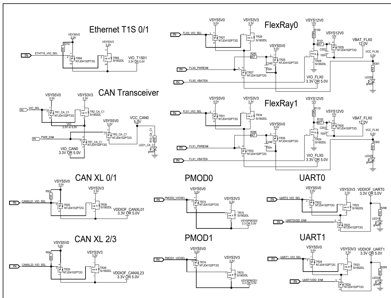
Figure 3.13 VDDIOF for peripheral circuits (2) of board version D019712_06_V04 and later
