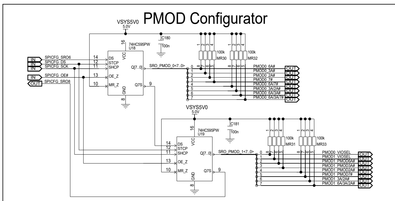
Figure 5.49 Pmod configuration signals
