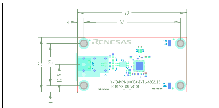
Figure 5.26 Y-COMMON-1000BASE-T1-88Q2112 dimensions
