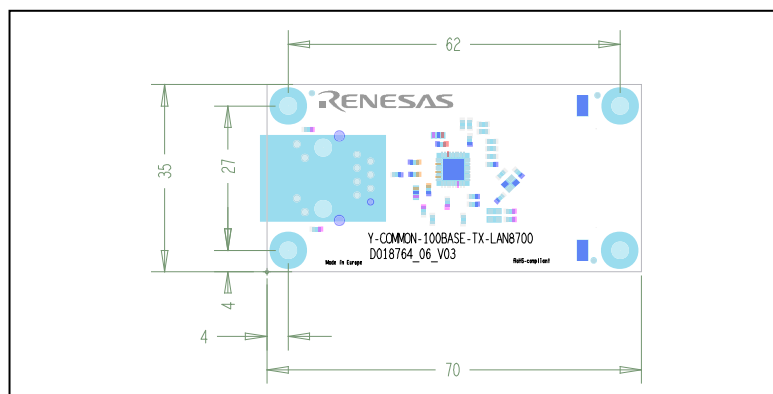
Figure 5.24 Y-COMMON-100BASE-TX-LAN8700 dimensions
