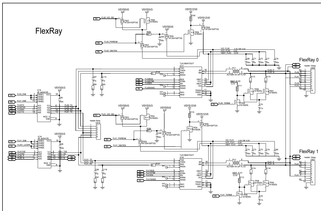
Figure 5.16 FlexRay interface circuit diagram of board version D019712_06_V01
