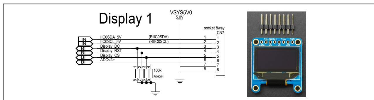
Figure 5.48 OLED display connection of board version D019712_06_V02 and later
