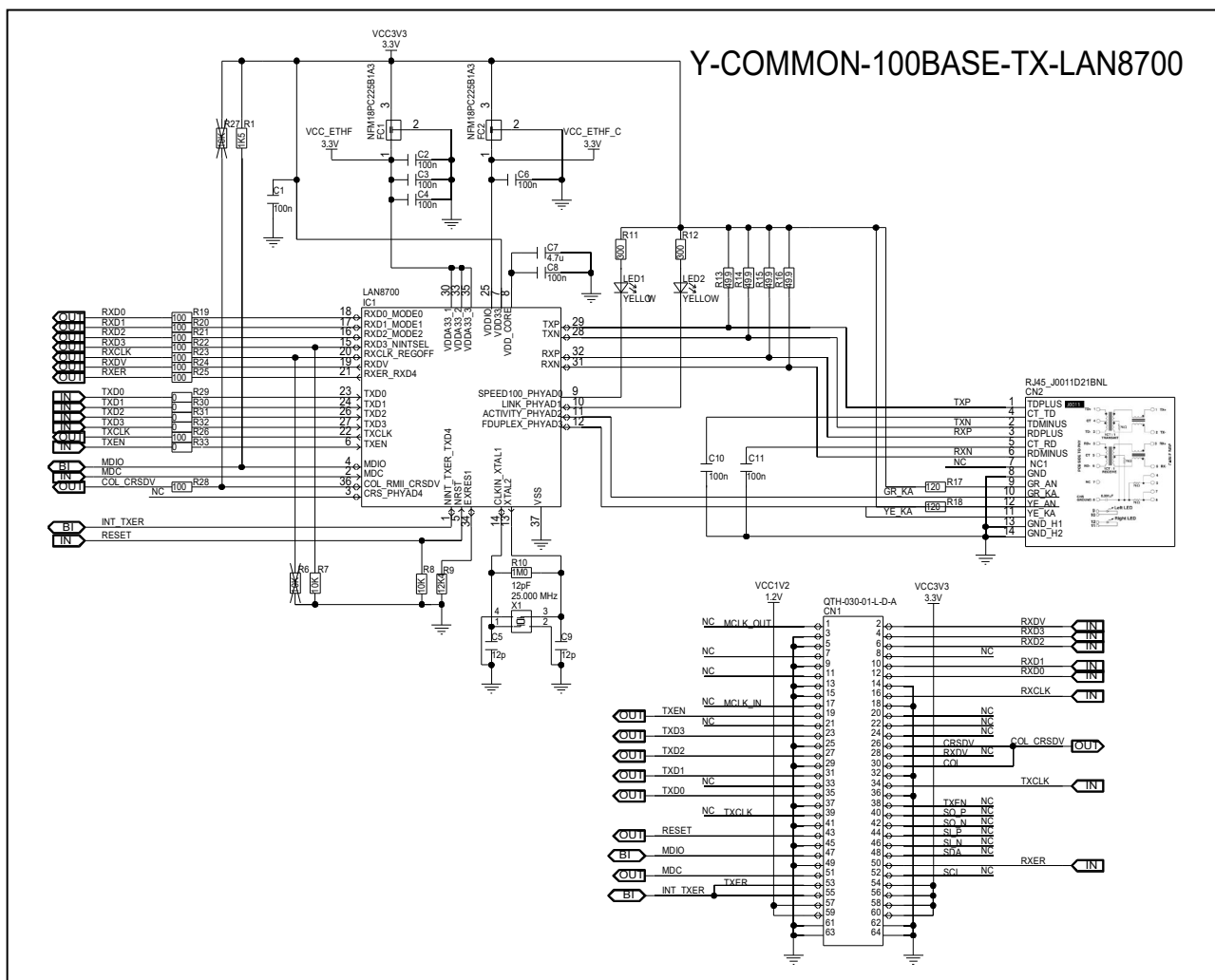
Figure 5.23 Circuit diagram of Renesas Ethernet board Y-COMMON-100BASE-TX-LAN8700
