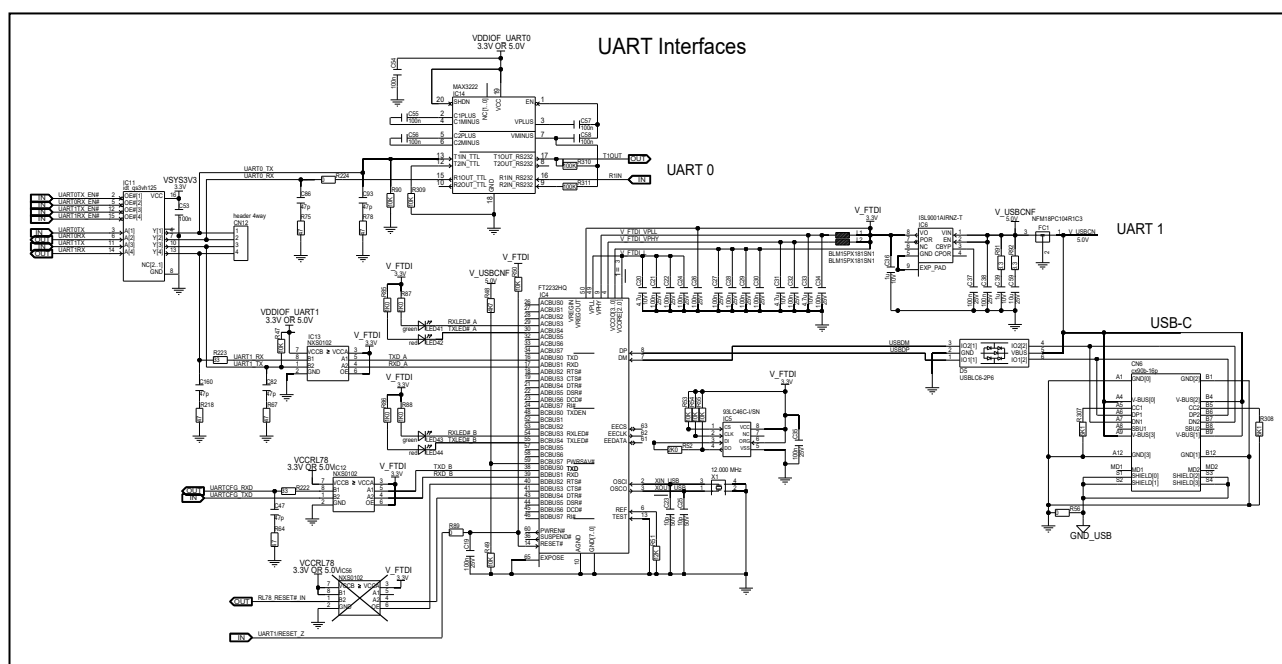
Figure 5.38 UART interface circuit diagram of board version D019712_06_V03
