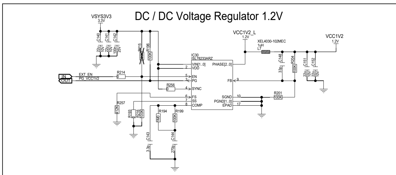
Figure 3.7 Core voltage regulator 1.2V
