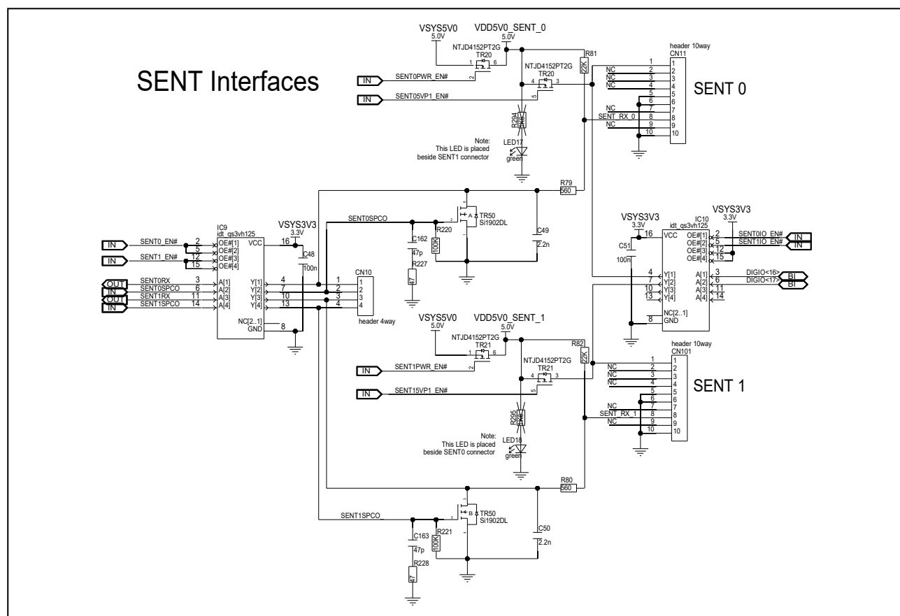
Figure 5.32 SENT interfaces of board version D019712_06_V02
