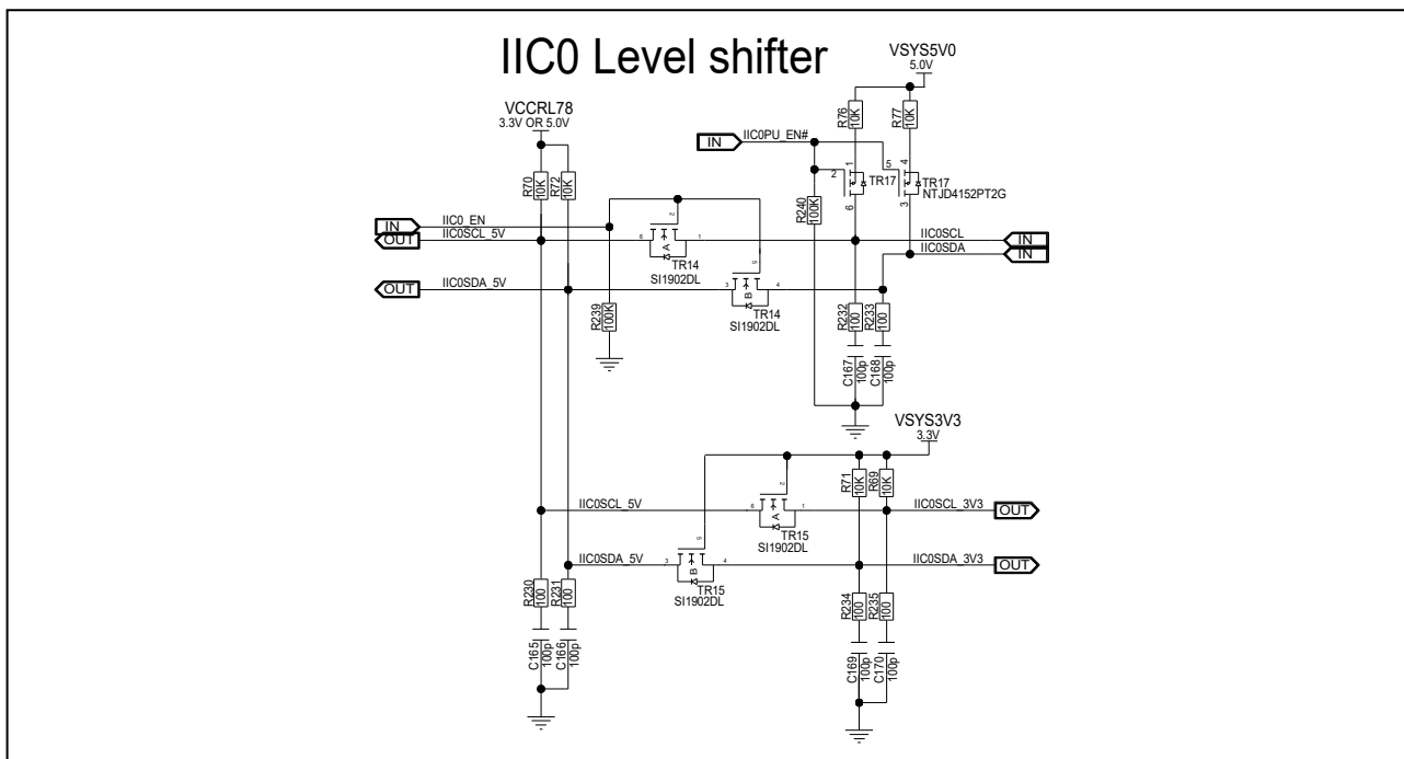
Figure 5.72 IIC level shift circuit of boardversion D019712_06_V01
