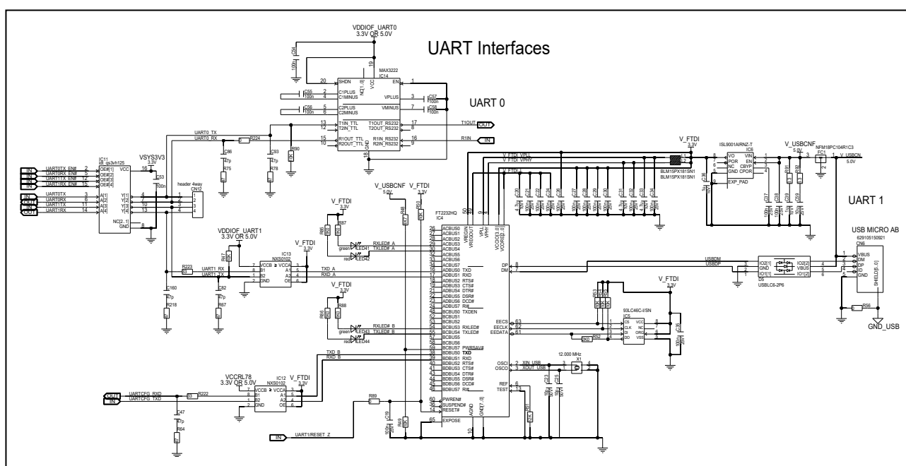
Figure 5.36 UART interface circuit diagram of board version D019712_06_V01
