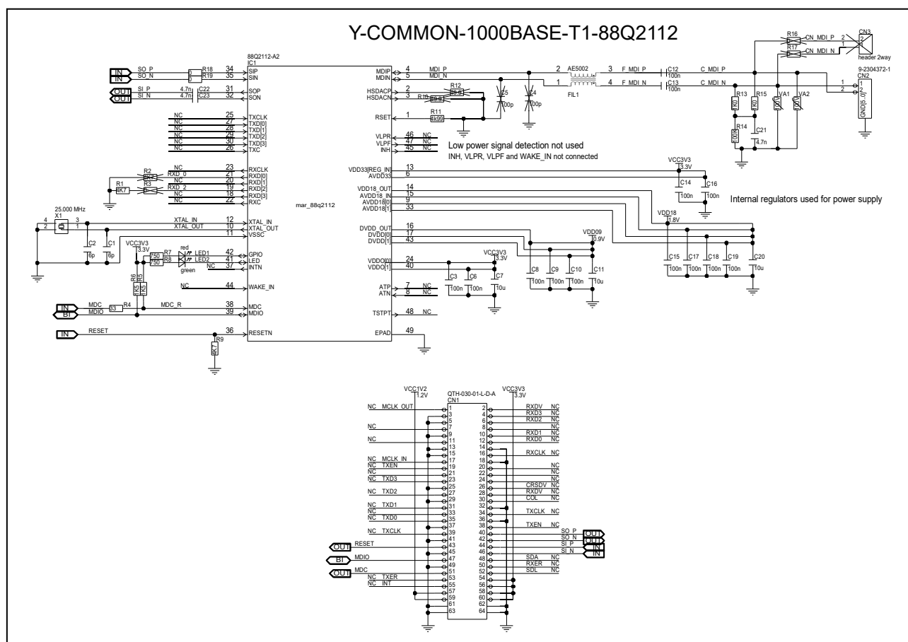
Figure 5.25 Circuit diagram of Renesas Ethernet board Y-COMMON-1000BASE-T1-88Q2112
