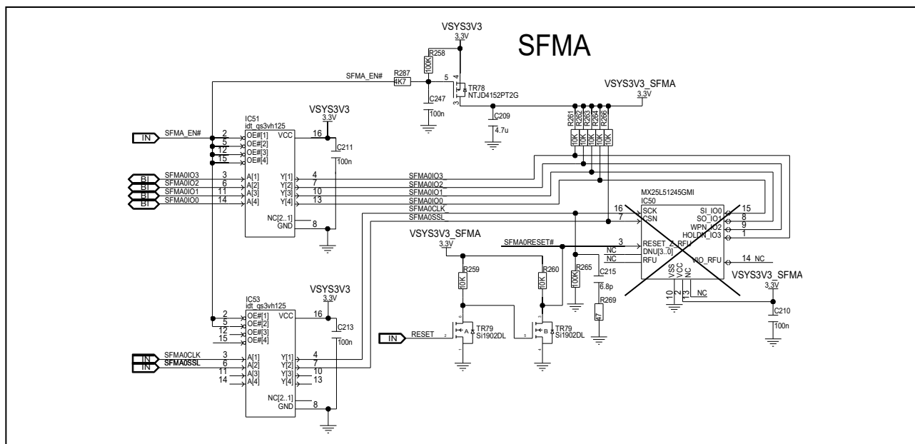
Figure 5.41 SFMA circuit of board version D019712_06_V01
