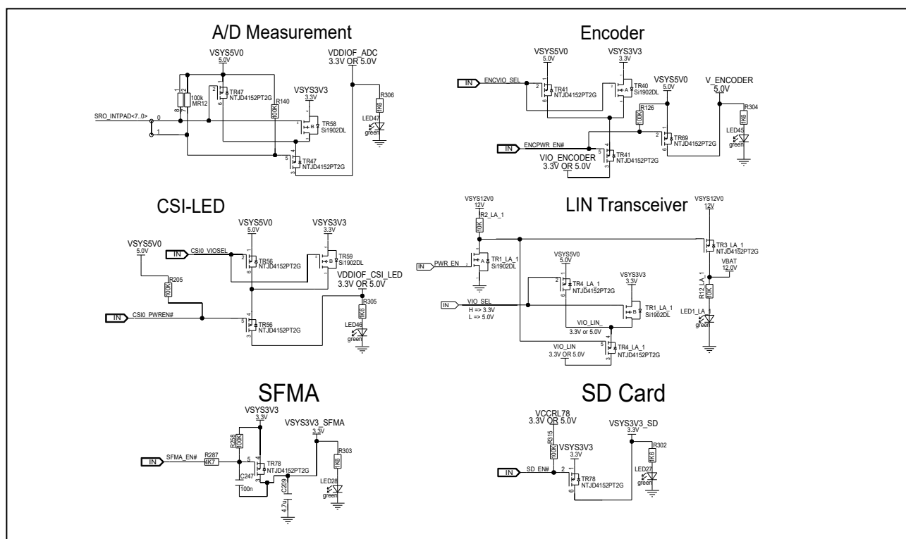
Figure 3.10 VDDIOF for peripheral circuits (1) of board version D019712_06_V02 and D019712_06_V03
