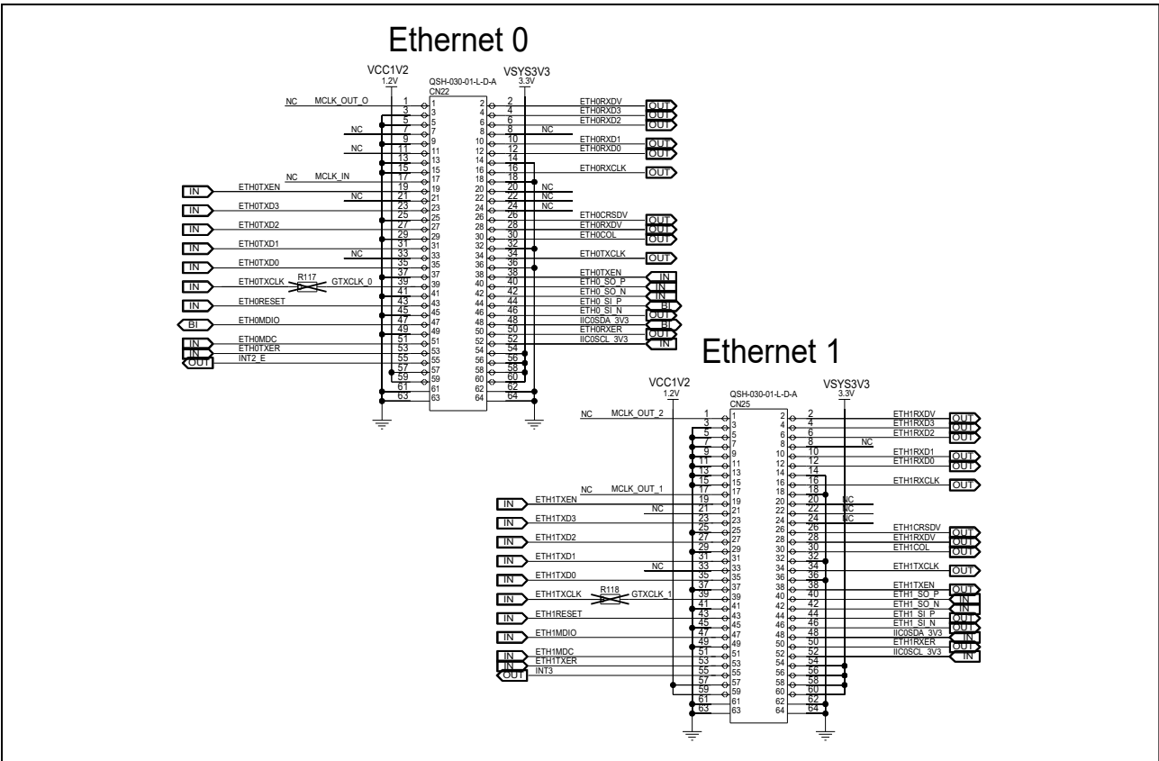
Figure 5.20 Ethernet module connector circuit for MII/SGMII compliant Ethernet modules of board version D019712_06_V01
