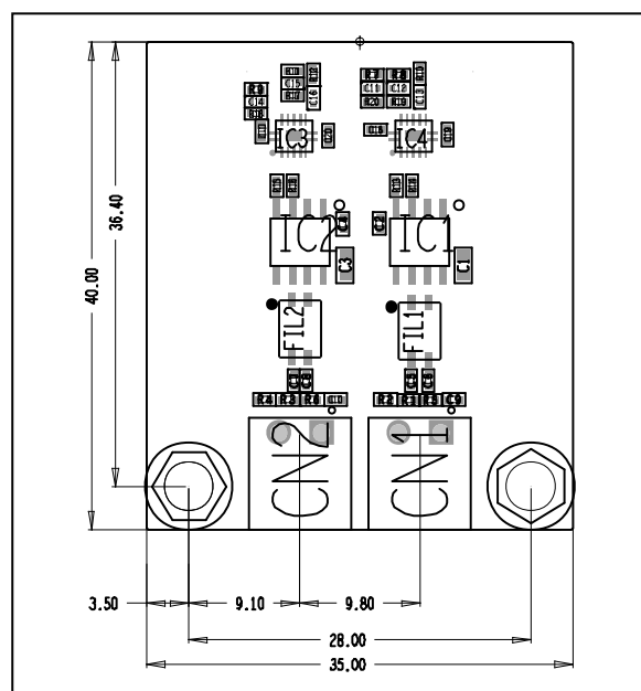
Figure 5.29 Y-COMMON-10BASE-T1S-NN dimensions
