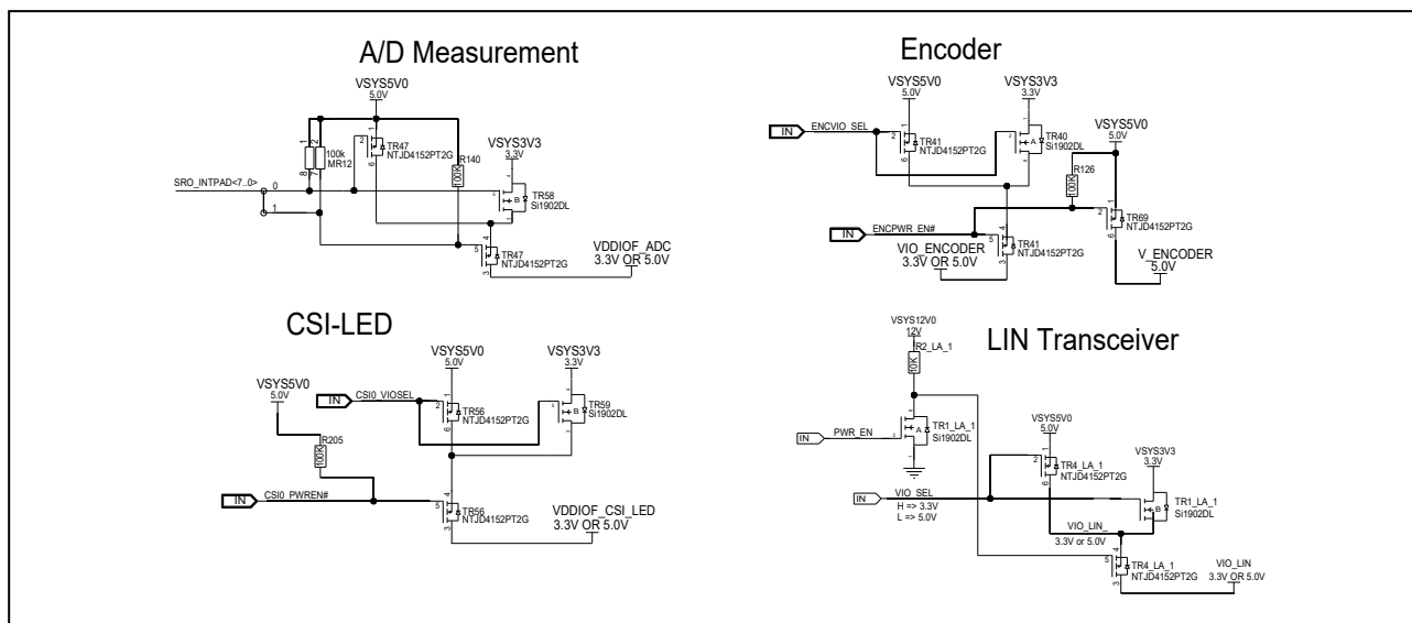
Figure 3.8 VDDIOF for peripheral circuits (1) of board version D019712_06_V01
