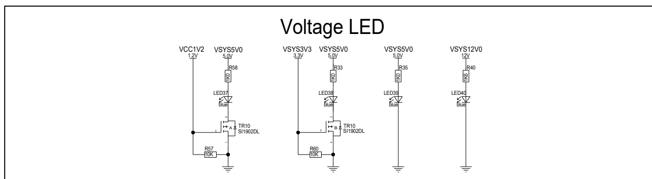
Figure 3.14 Power supply LEDs
