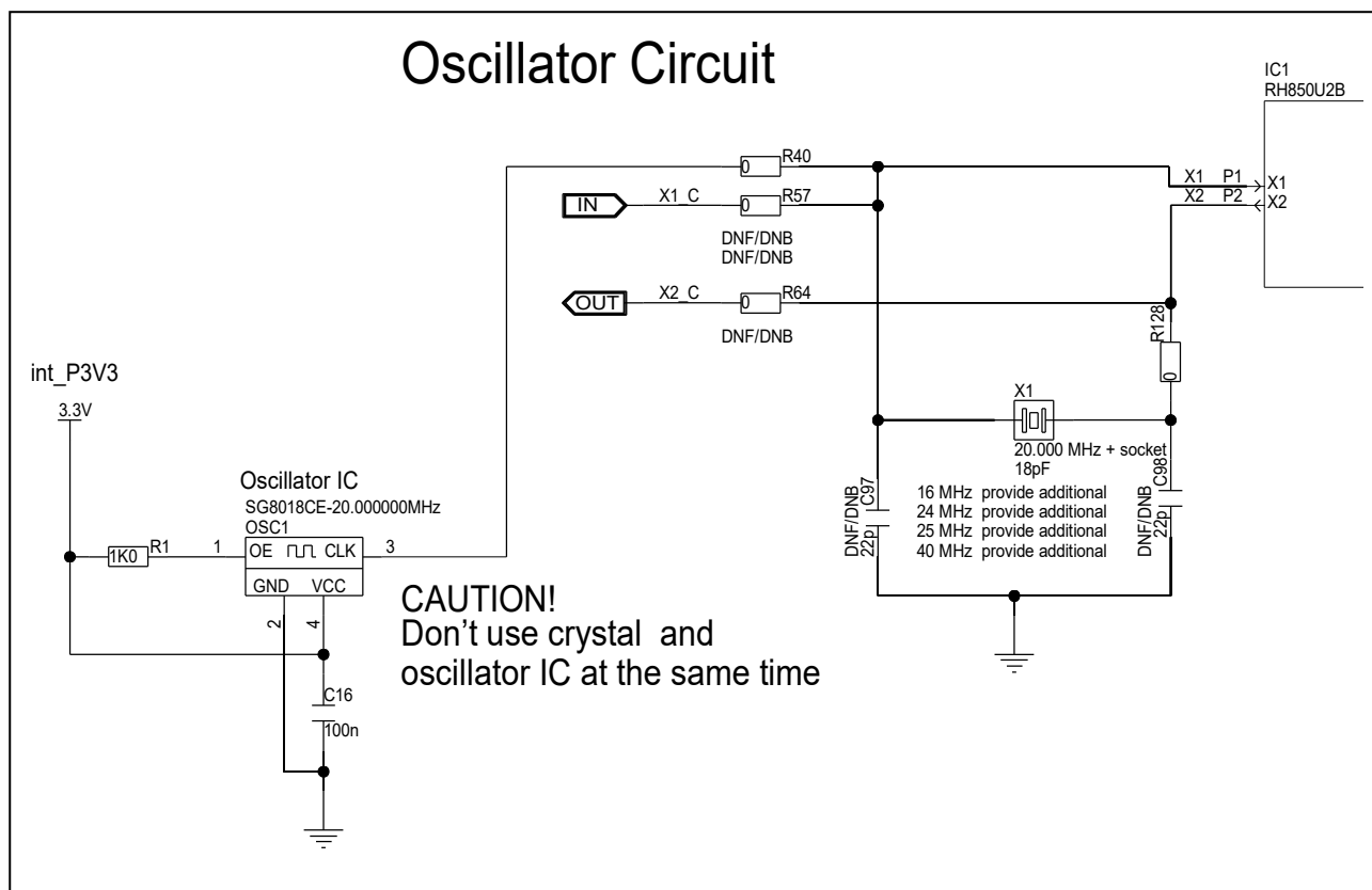
Figure 4.1 Clock supply
