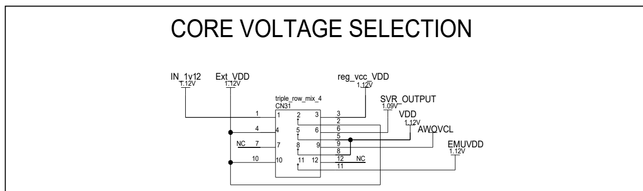
Figure 3.3 Device core voltage (VDD) selection
