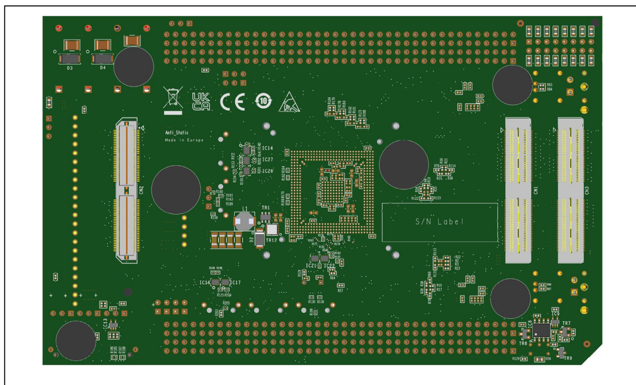
Figure 1.6 D018177_06_V03 Piggyback board bottom view
