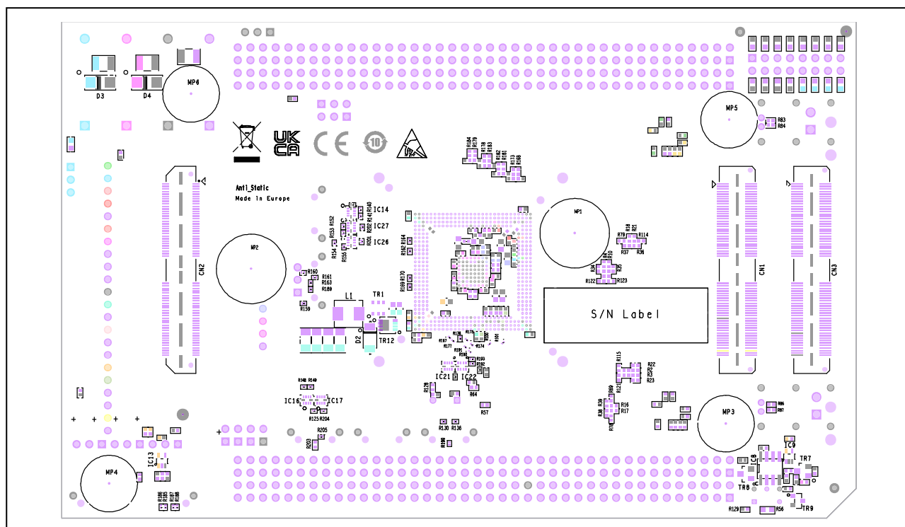
Figure 1.12 D018177_06_V03 Piggyback Board bottom view
