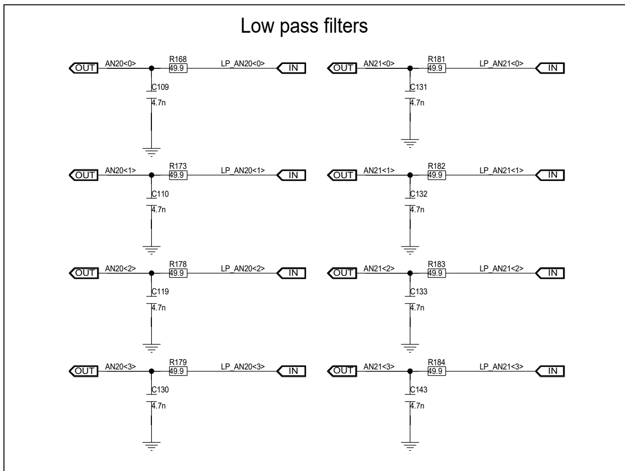
Figure 6.20 Circuit diagram for low pass filters
