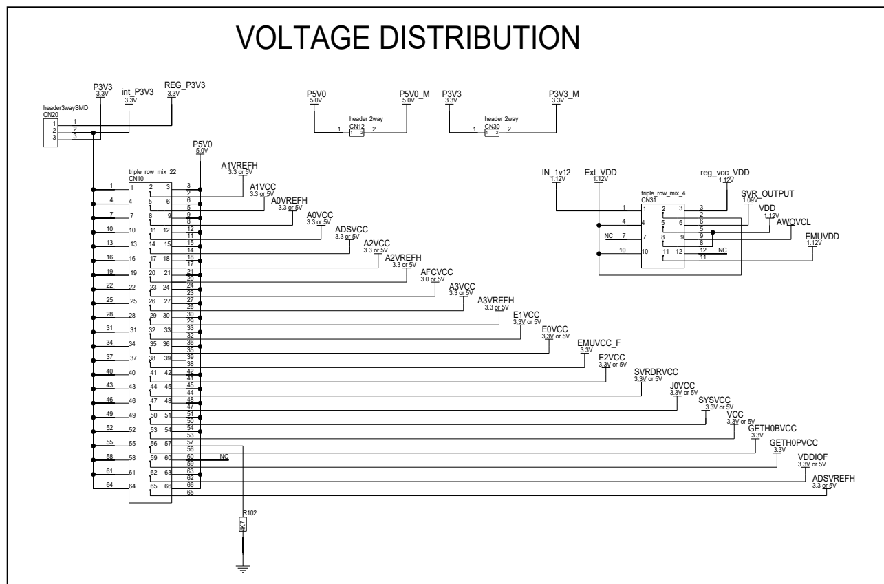
Figure 3.1 Voltage distribution on board version D018177_06_V01
