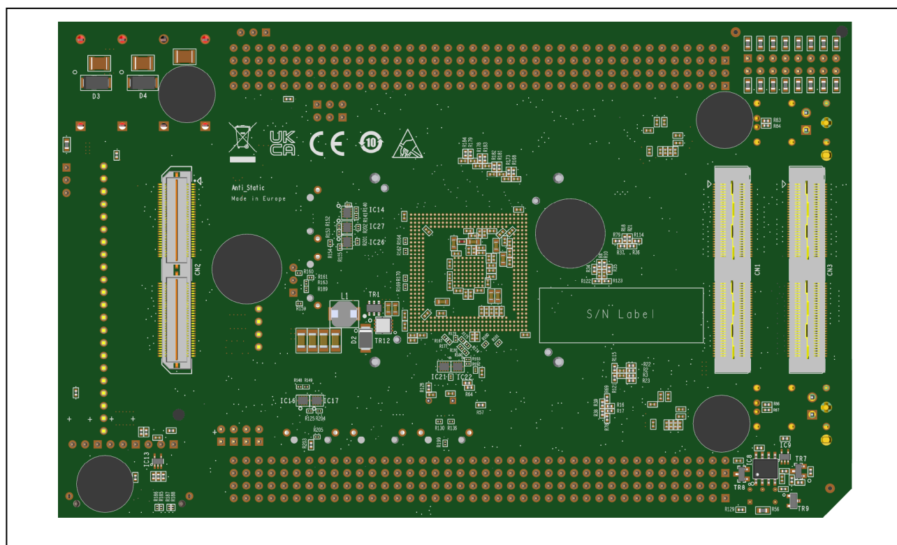
Figure 1.4 D018177_06_V02 Piggyback board bottom view
