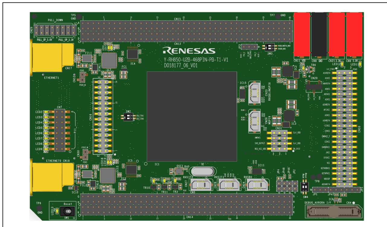
Figure 1.1 D018177_06_V01 Piggyback board top view
