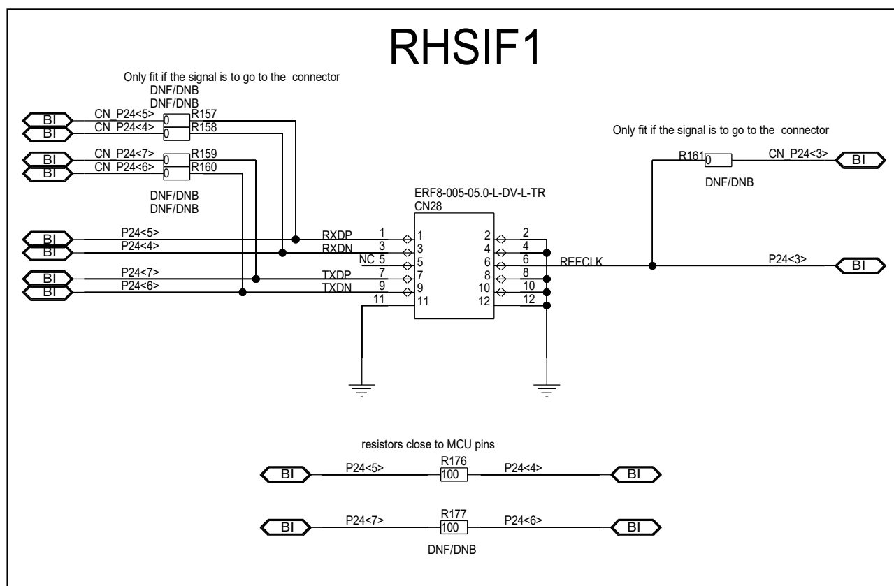
Figure 6.13 Circuit diagram for RHSIF1 interface on board version D018177_06_V01
