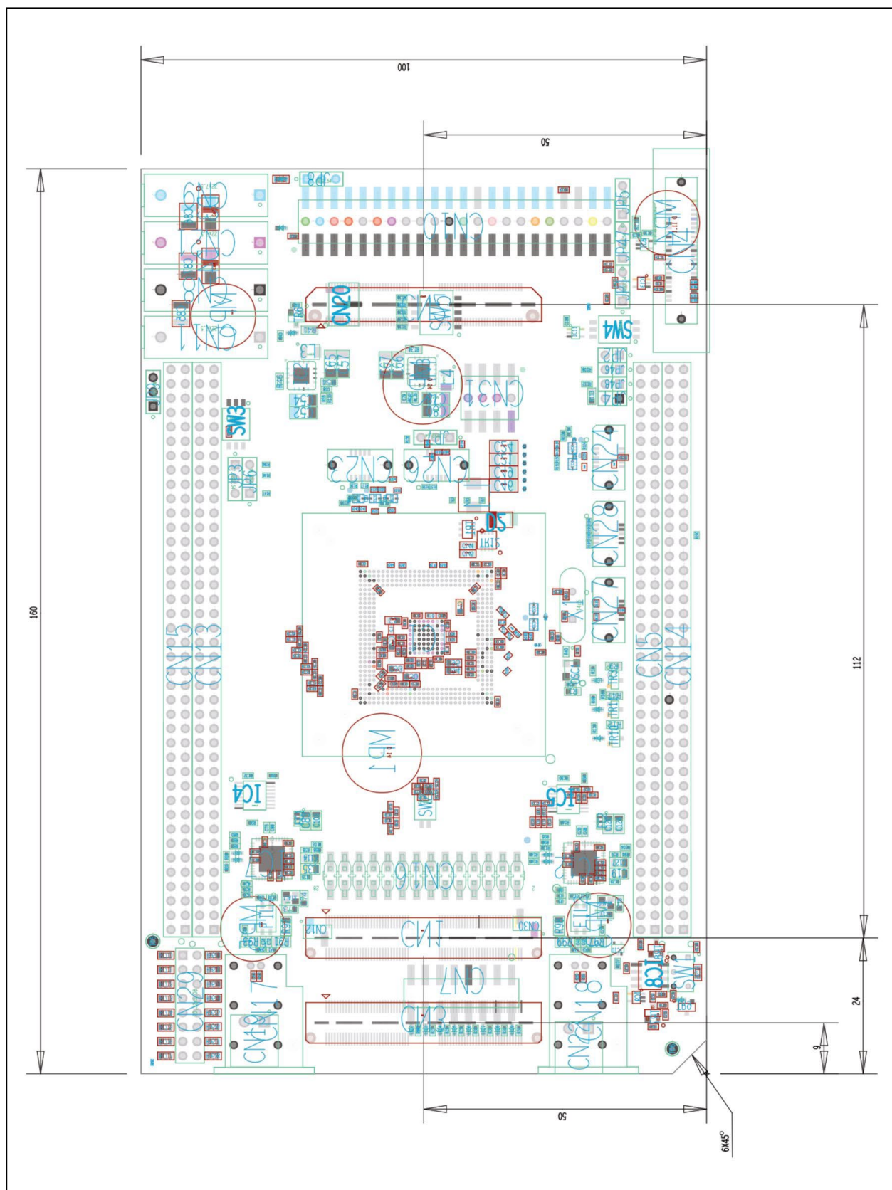
Figure 9.1 Mechanical dimensions
