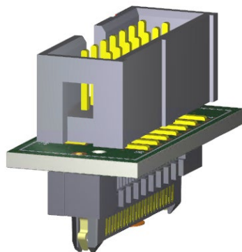
Figure 5.3 Outline view of debug adapter Y-RH850-DEBUG-ADAPTER-F14T46
