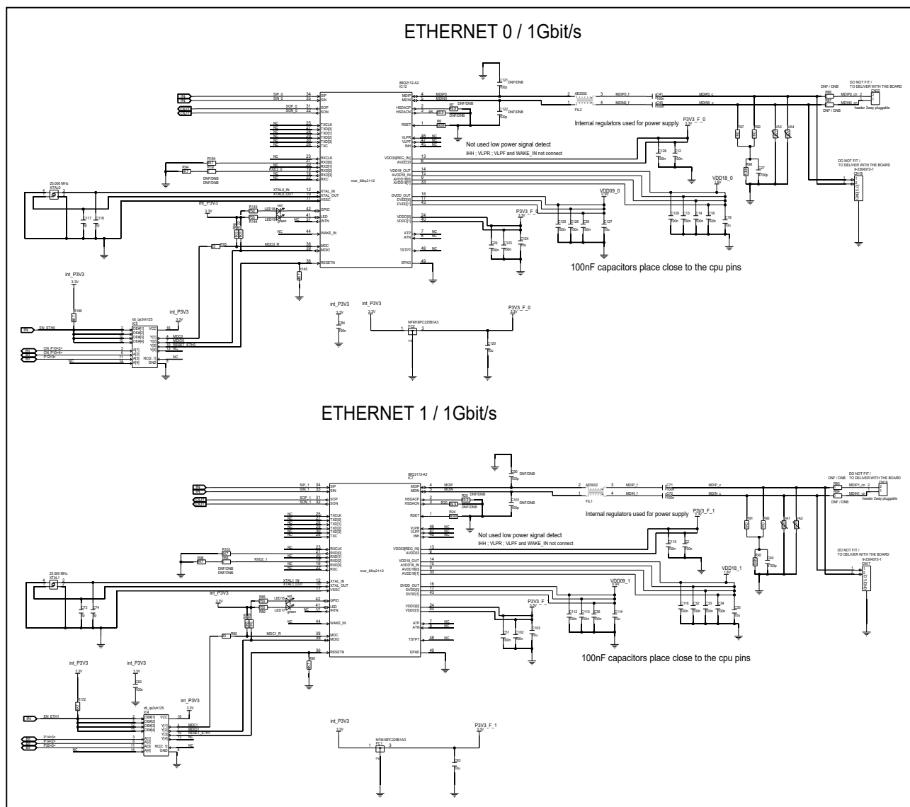
Figure 6.16 Ethernet circuits for ETN0 and ETN1 on board version D018177_06_V01
