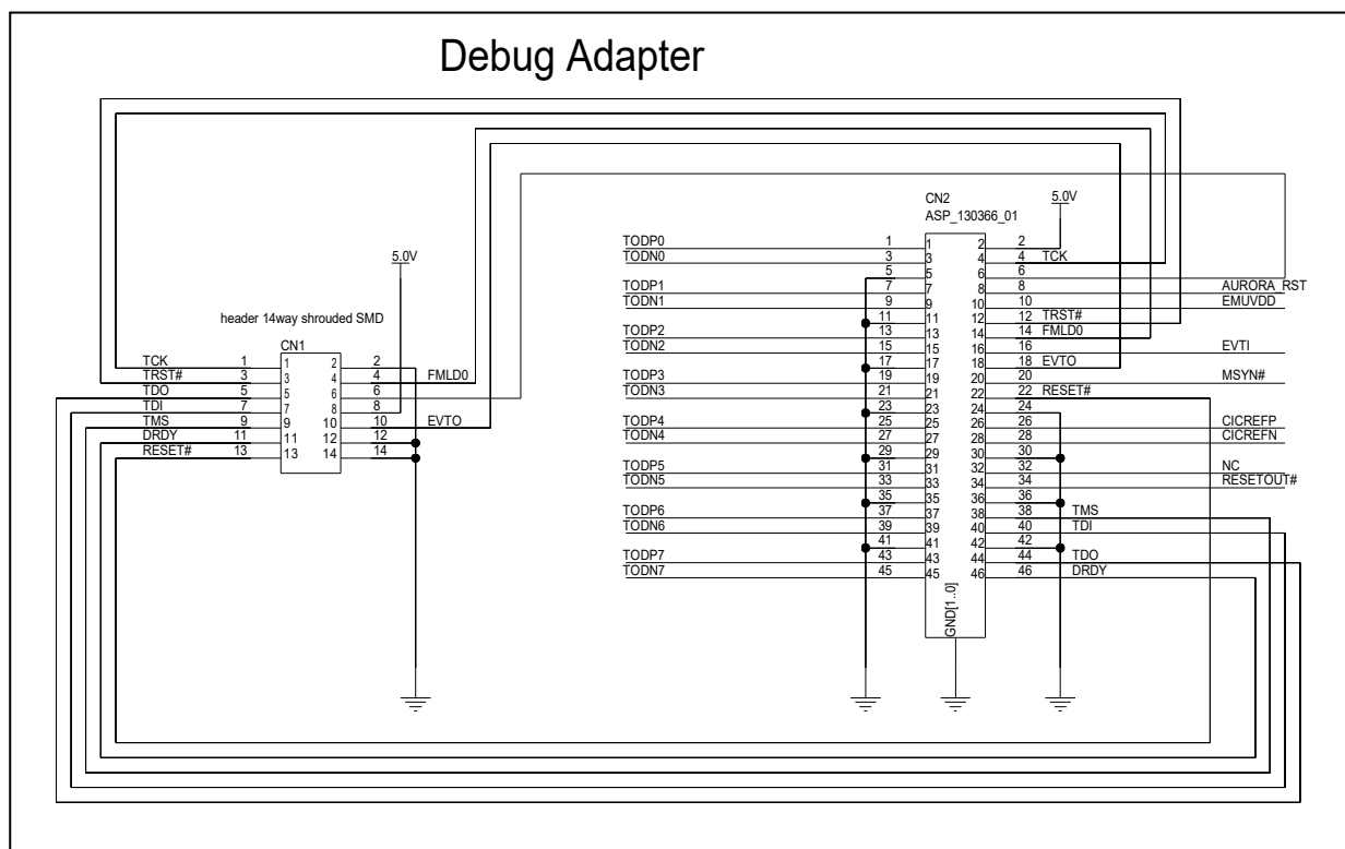
Figure 5.4 Circuit diagram of debug adapter Y-RH850-DEBUG-ADAPTER-F14T46
