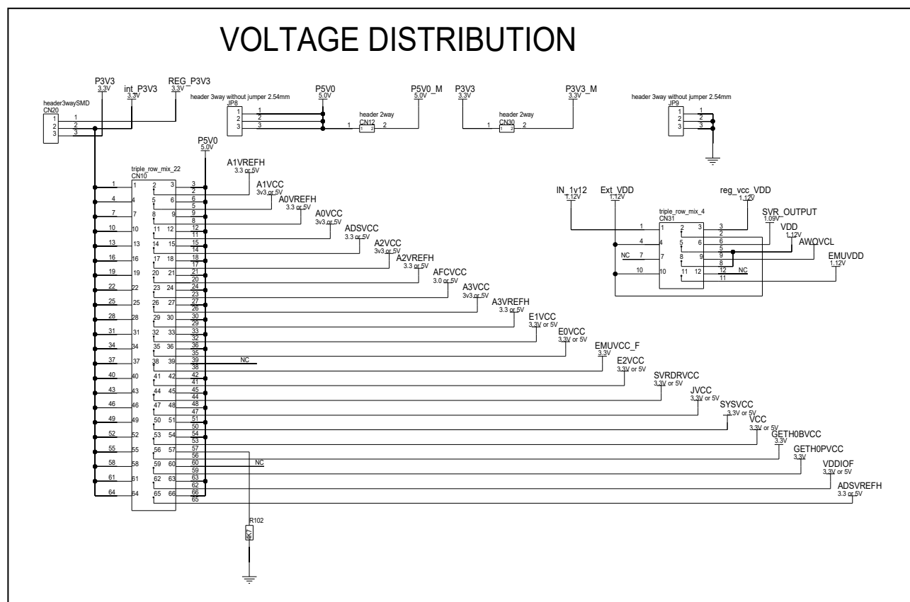
Figure 3.2 Voltage distribution on board versions other than D018177_06_V01
