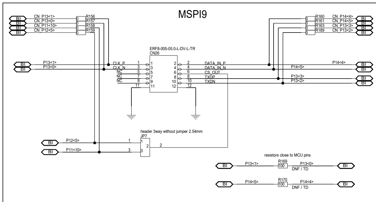
Figure 6.10 Circuit diagram for MSPI9 interface on board versions other than D018177_06_V01
