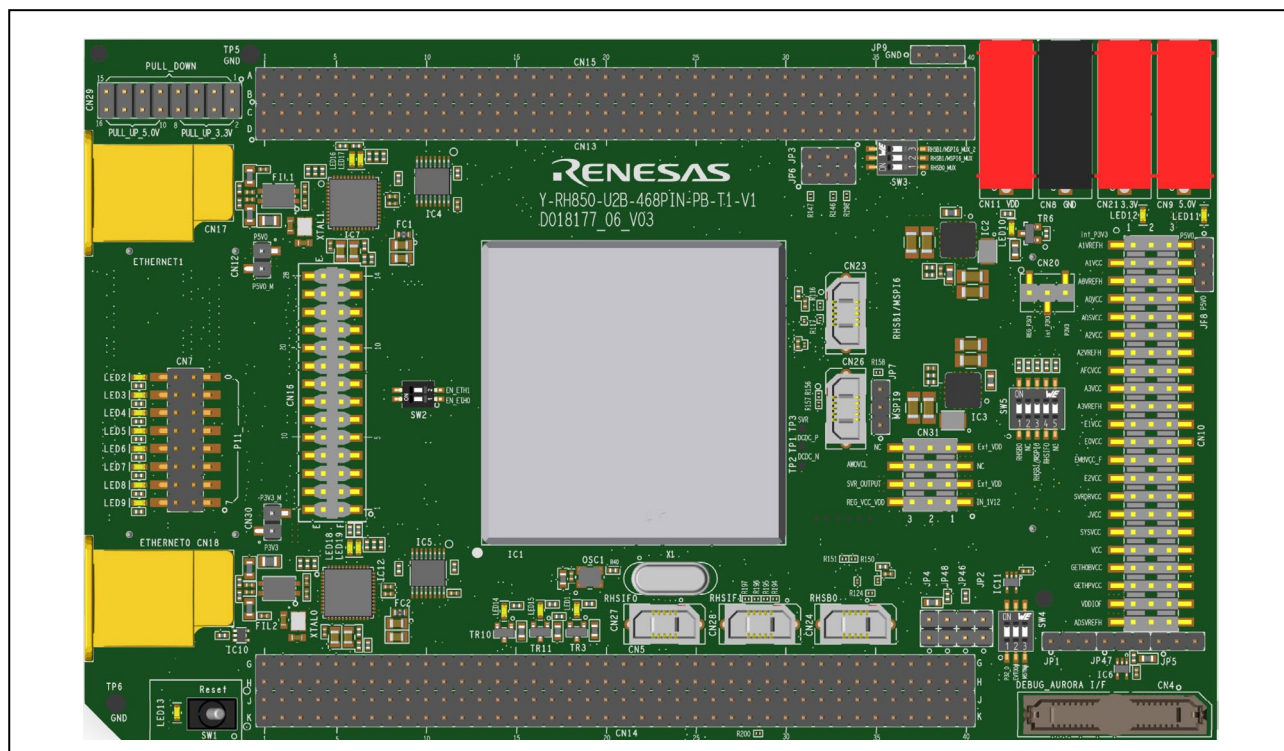
Figure 1.5 D018177_06_V03 Piggyback board top view
