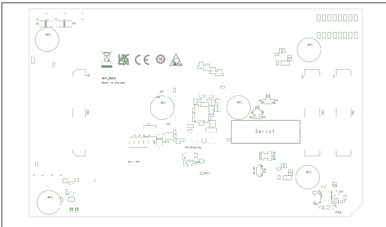
Figure 2.2 D018177_06_V01 Placement of jumpers, connectors and LEDs on top side
