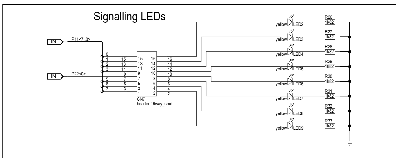
Figure 6.3 Circuit diagram for signaling LEDs on board versions other than D018177_06_V01
