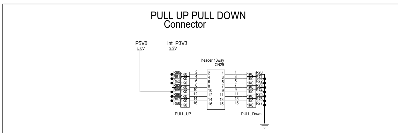
Figure 6.4 Circuit diagram for pull up / pull down signals
