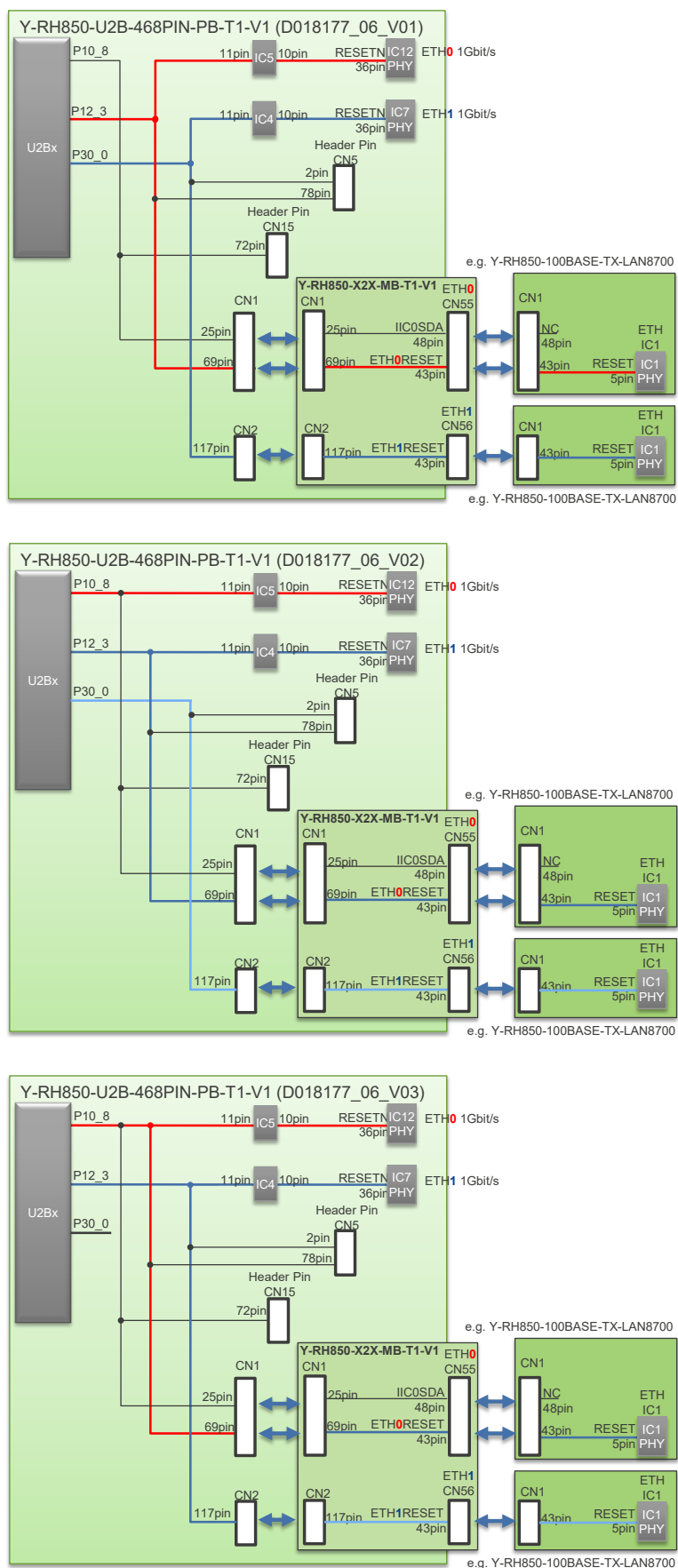
Figure 9.7 Ethernet reset signals on boards D018177_06_V01, D018177_06_V02 and D018177_06_V03
