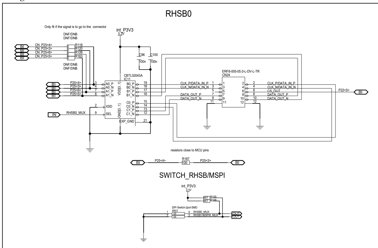
Figure 6.5 Circuit diagram for RHSB0 interface on board version D018177_06_V01
