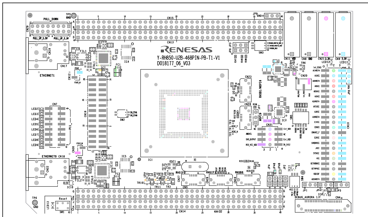
Figure 1.11 D018177_06_V03 Piggyback Board top view
