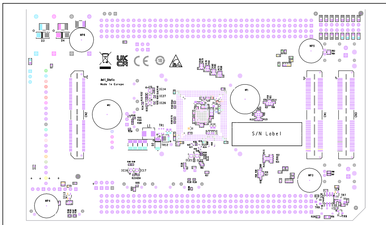
Figure 1.10 D018177_06_V02 Piggyback Board bottom view
