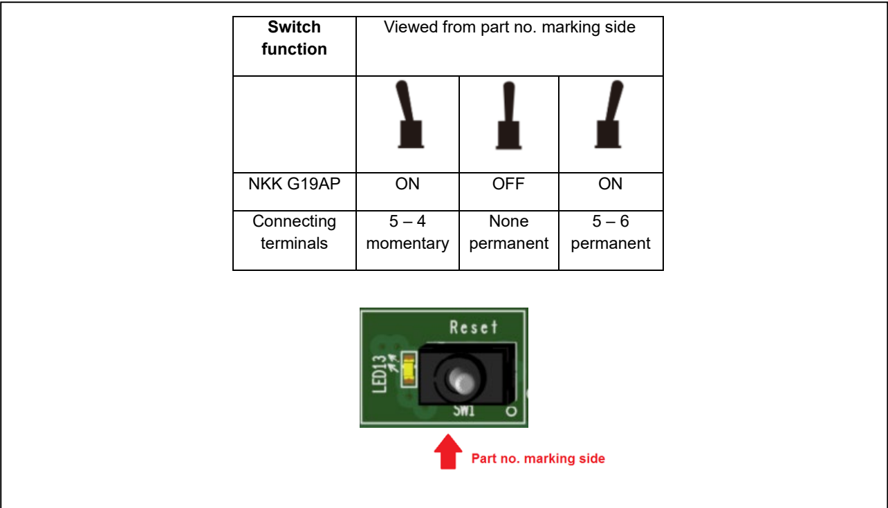
Figure 6.1 Operation of RESET switch
