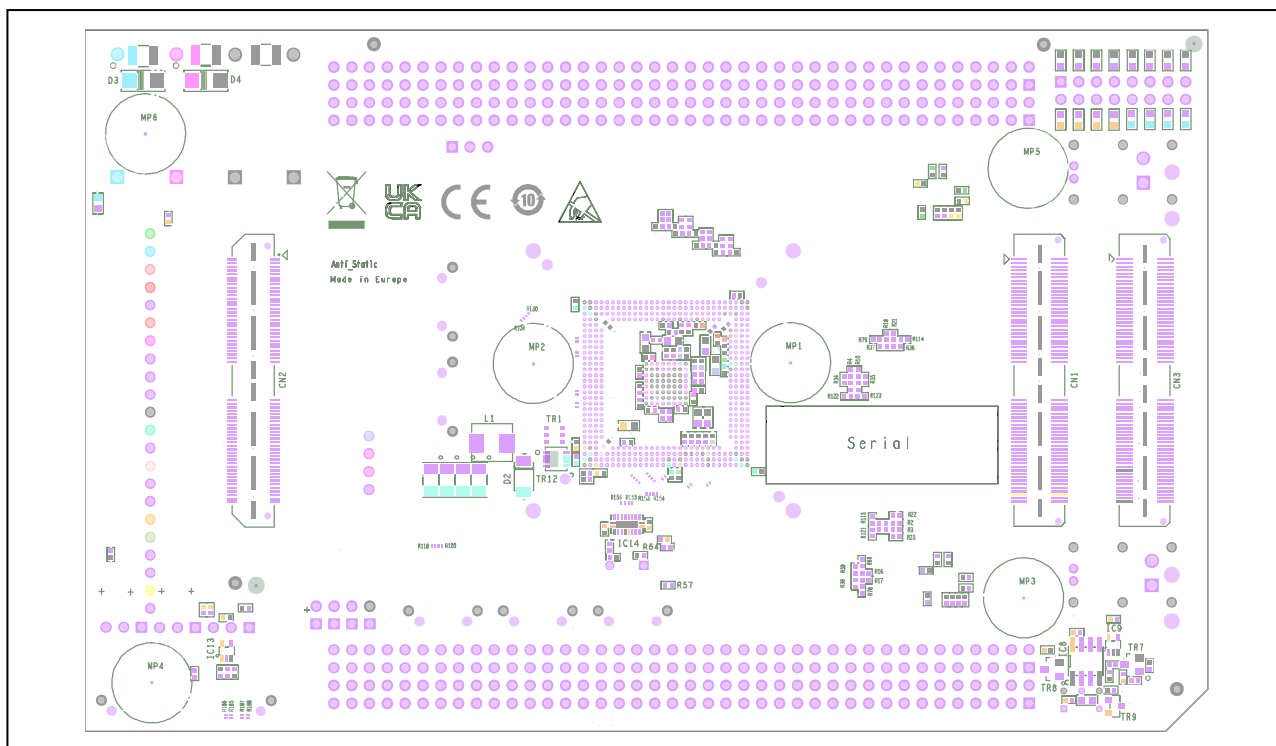
Figure 1.8 D018177_06_V01 Piggyback Board bottom view
