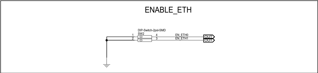
Figure 6.15 Switches to enable Ethernet channels
