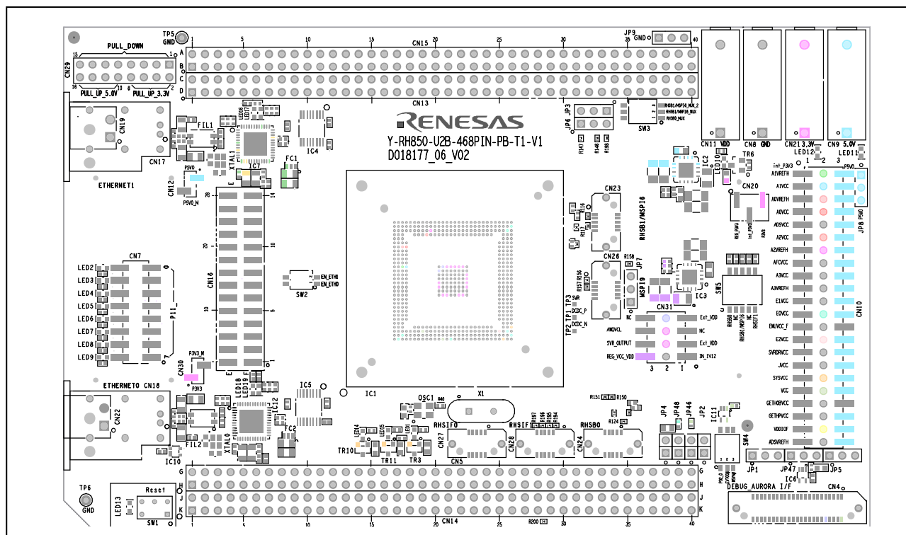
Figure 1.9 D018177_06_V02 Piggyback Board top view
