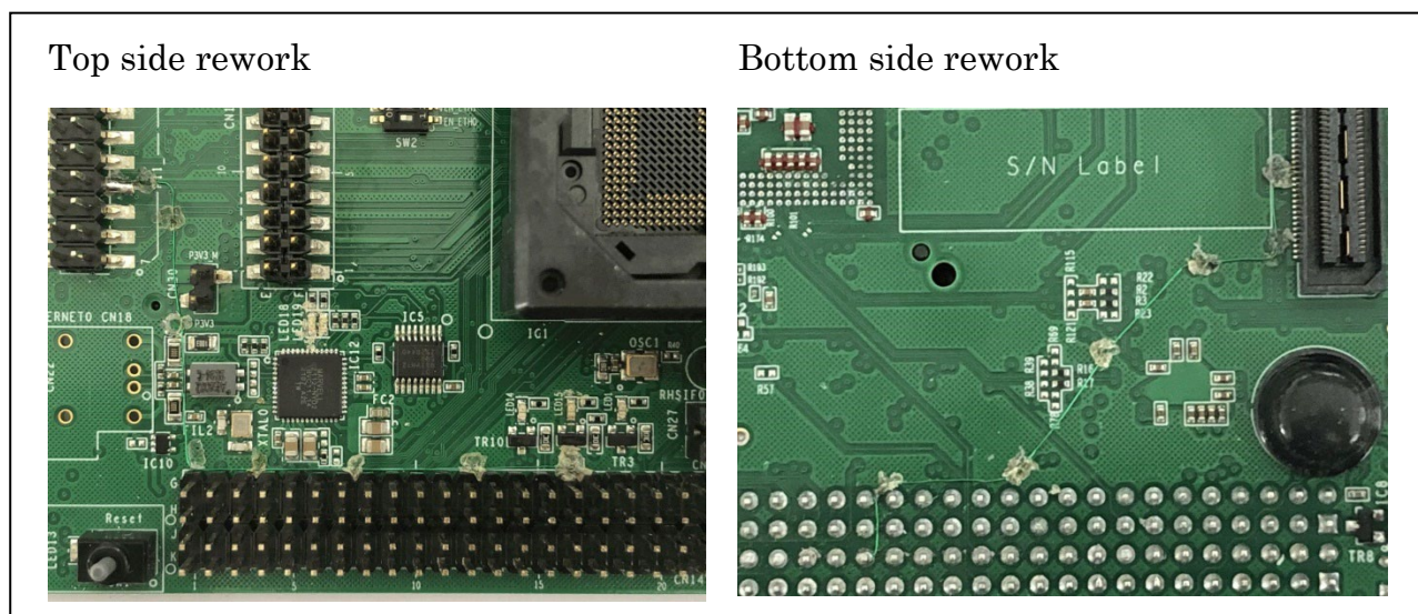
Figure 9.5 Board rework
